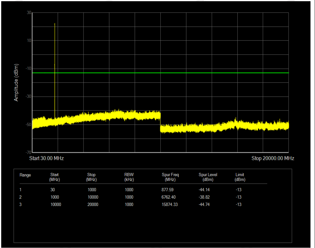
n66 SCS=15kHz DFT_BPSK BW=5MHz Channel=355500 RB=1@24
