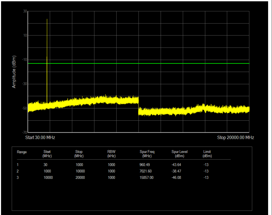
n66 SCS=15kHz DFT_BPSK BW=20MHz Channel=349000 RB=1@105
