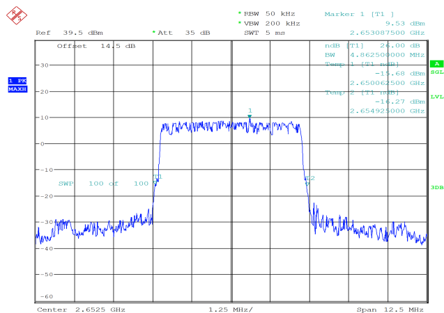
26dB Bandwidth 4.862MHz
