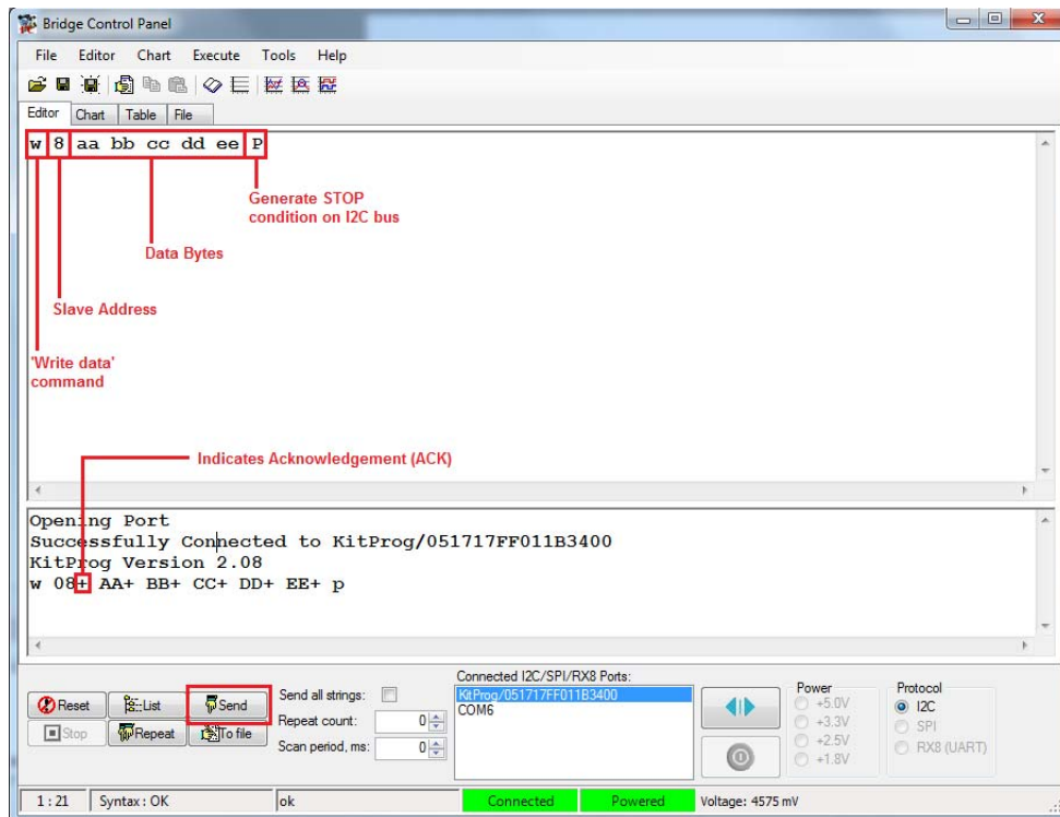
Figure 6-24. Entering Commands in BCP
