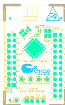
Figure A-11. Primary Silkscreen of PProC BLE Module
