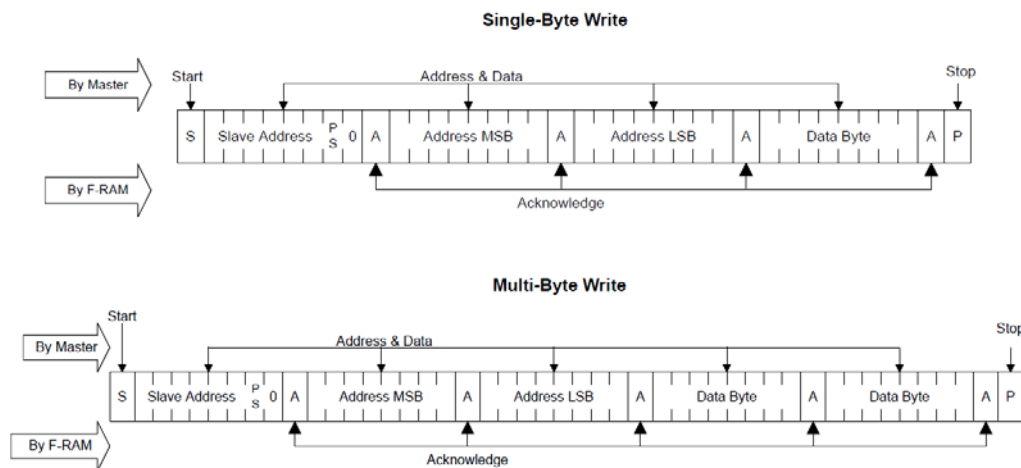
Figure 6-48. F-RAM Single-Byte and Multiple-Byte Write Packet Structure
