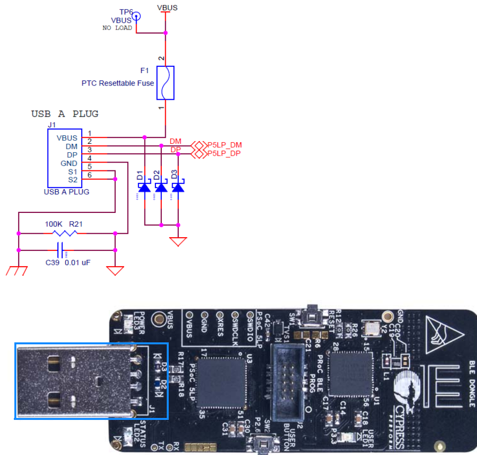
Figure 5-27. Schematics and Board Highlight of USB Type A Plug
