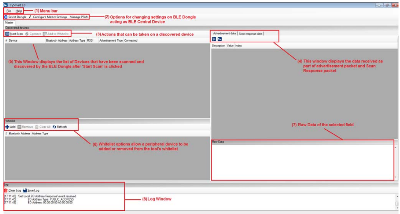
Figure 6-62. CySmart PC Tool Main Window
