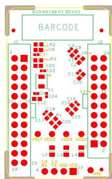
Figure A-12. Secondary Silkscreen of PProC BLE Module
