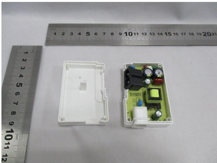
LED driver open view
