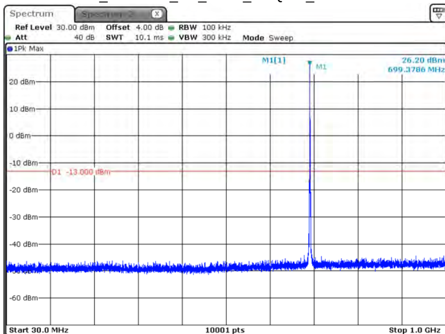
B12_CH23035_5M_1RB0_16-QAM_Below 1G
