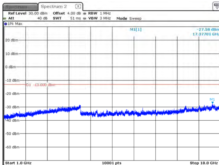
B12_CH23130_10M_1RB5_16-QAM_Above 1G
