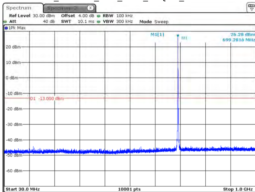
B12_CH23017_1.4M_1RB0_16-QAM_Below 1G
