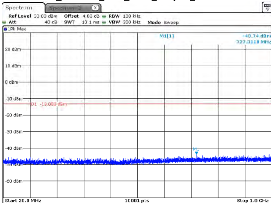
B25_CH26365_1.4M_1RB0_16-QAM_Below 1G
