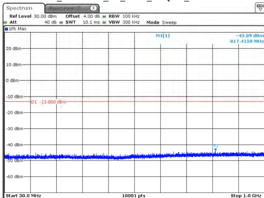
B66_CH131997_5M_1RB0_16-QAM_Below 1G
