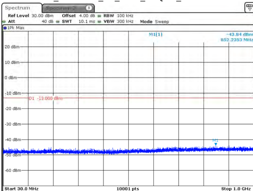
B66_CH132322_5M_1RB0_16-QAM_Below 1G
