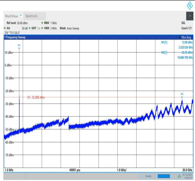
7-7-15MHz-10MHz-QPSK-QPSK-21051-21171-1RB#0-1RB#4 9-1000~20000MHz-PASS
