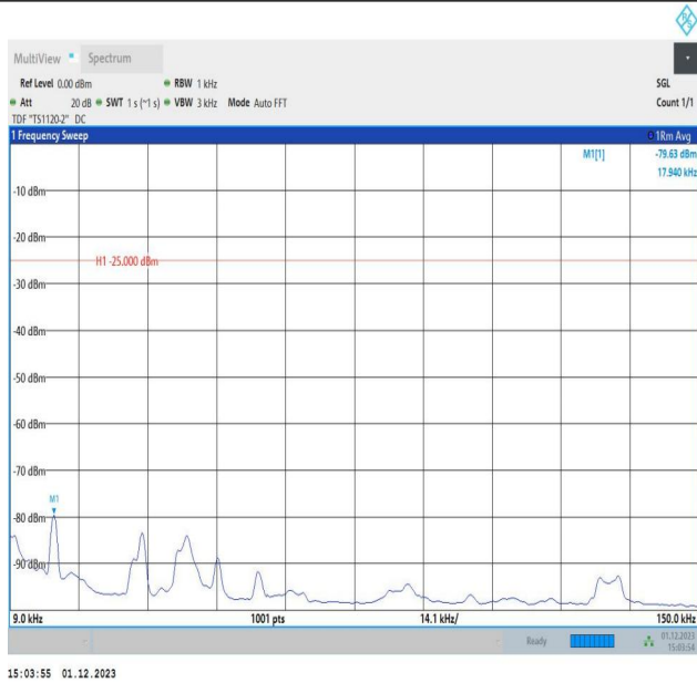
7-7-15MHz-10MHz-16QAM-16QAM-21051-21171-75RB#0-50 RB#0-0.009~0.15MHz-PASS
