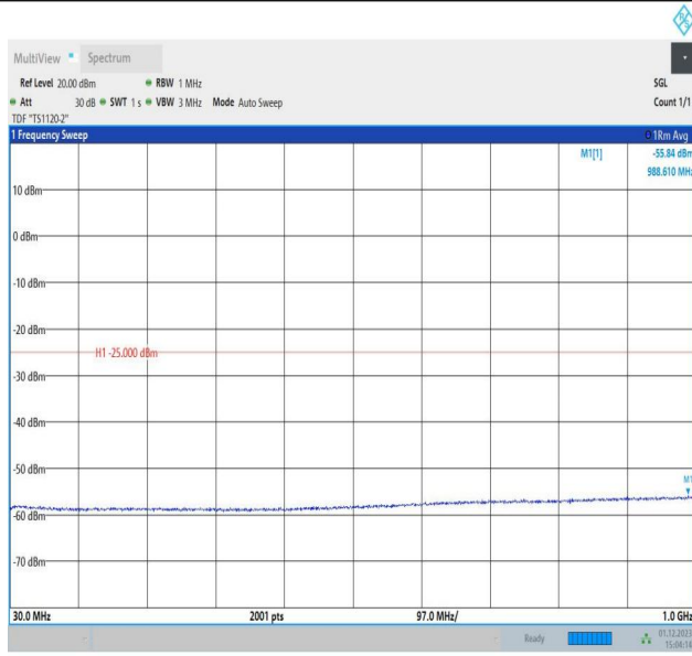
7-7-15MHz-10MHz-16QAM-16QAM-21051-21171-75RB#0-50 RB#0-30~1000MHz-PASS
