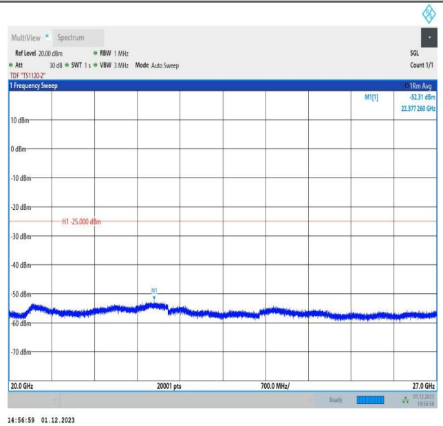
7-7-15MHz-10MHz-64QAM-64QAM-20825-20945-75RB#0-50 RB#0-20000~27000MHz-PASS
