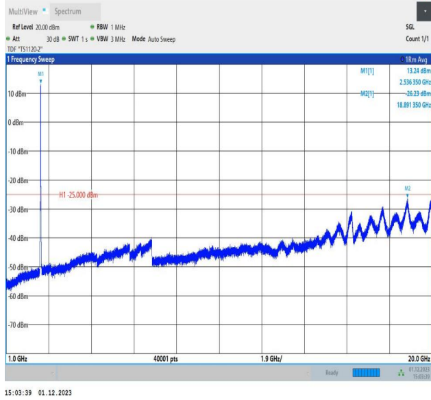
7-7-15MHz-10MHz-QPSK-QPSK-21051-21171-75RB#0-50RB #0-1000~20000MHz-PASS
