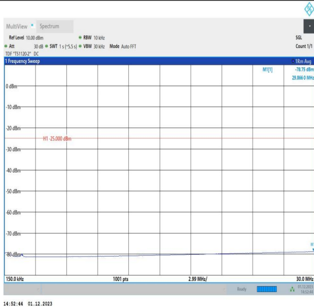
7-7-15MHz-10MHz-64QAM-64QAM-20825-20945-1RB#74-0R B#0-0.15~30MHz-PASS
