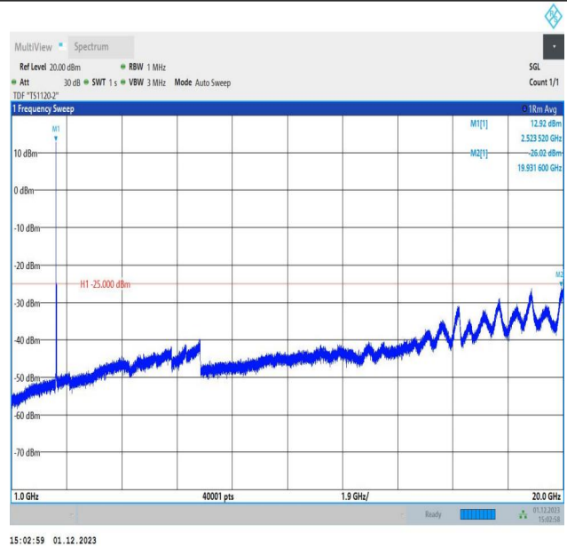
7-7-15MHz-10MHz-64QAM-64QAM-21051-21171-1RB#0-1RB #49-1000~20000MHz-PASS
