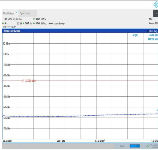
7-7-15MHz-10MHz-QPSK-QPSK-20825-20945-1RB#0-1RB#4 9-30~1000MHz-PASS
