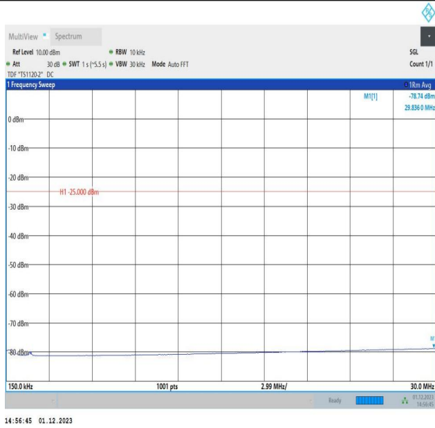
7-7-15MHz-10MHz-64QAM-64QAM-20825-20945-75RB#0-50 RB#0-0.15~30MHz-PASS
