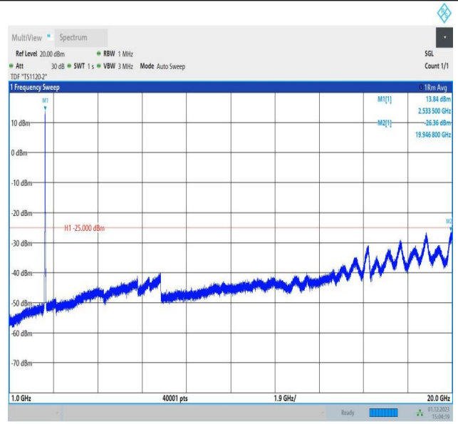
7-7-15MHz-10MHz-16QAM-16QAM-21051-21171-75RB#0-50 RB#0-1000~20000MHz-PASS
