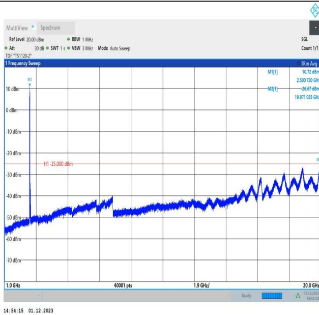
7-7-15MHz-10MHz-16QAM-16QAM-20825-20945-1RB#0-1RB #49-1000~20000MHz-PASS
