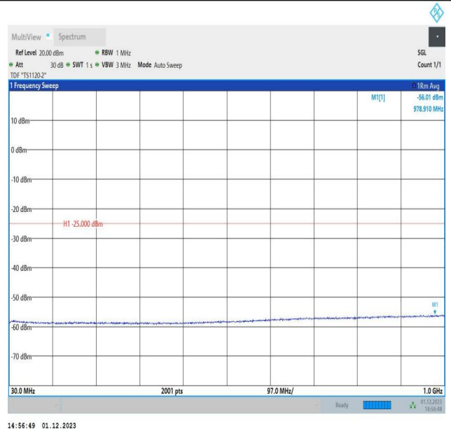
7-7-15MHz-10MHz-64QAM-64QAM-20825-20945-75RB#0-50 RB#0-30~1000MHz-PASS
