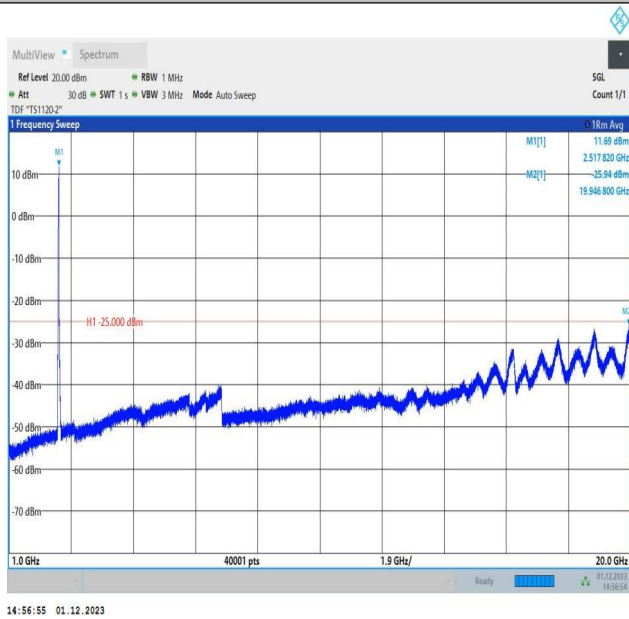
7-7-15MHz-10MHz-64QAM-64QAM-20825-20945-75RB#0-50 RB#0-1000~20000MHz-PASS
