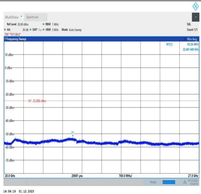
7-7-15MHz-10MHz-16QAM-16QAM-20825-20945-1RB#0-1RB #49-20000~27000MHz-PASS
