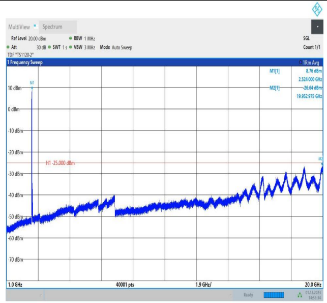
7-7-15MHz-10MHz-QPSK-QPSK-20825-20945-1RB#0-1RB#4 9-1000~20000MHz-PASS
