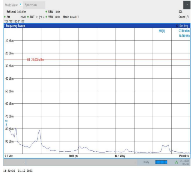
7-7-15MHz-10MHz-64QAM-64QAM-20825-20945-1RB#74-0R B#0-0.009~0.15MHz-PASS
