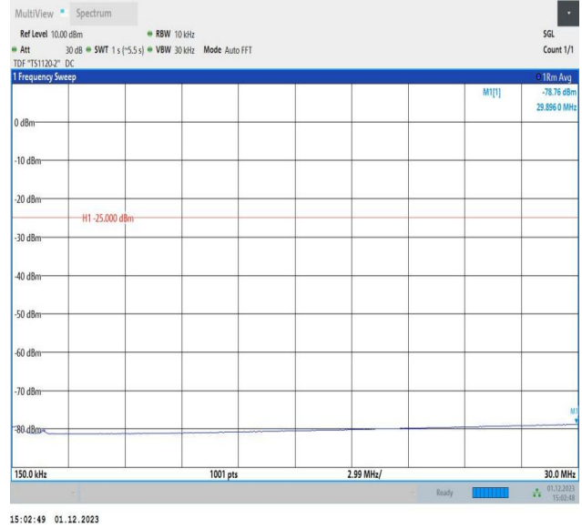
7-7-15MHz-10MHz-64QAM-64QAM-21051-21171-1RB#0-1RB #49-0.15~30MHz-PASS
