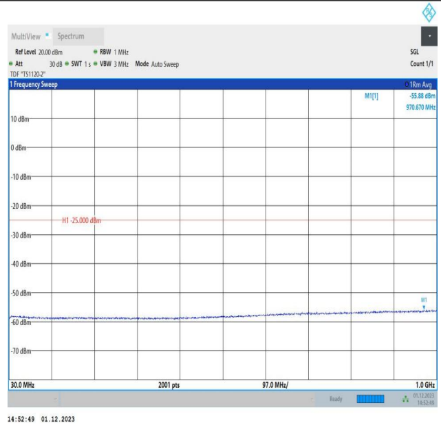
7-7-15MHz-10MHz-64QAM-64QAM-20825-20945-1RB#74-0R B#0-30~1000MHz-PASS
