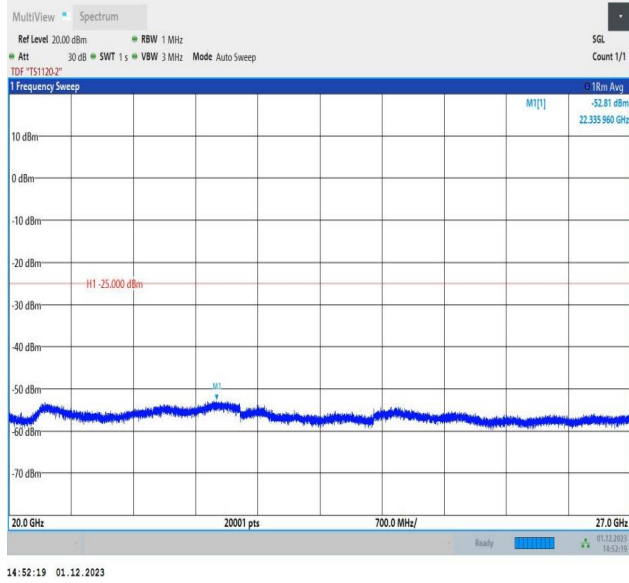
7-7-15MHz-10MHz-16QAM-16QAM-20825-20945-1RB#74-0R B#0-20000~27000MHz-PASS
