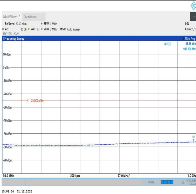
7-7-15MHz-10MHz-64QAM-64QAM-21051-21171-1RB#0-1RB #49-30~1000MHz-PASS
