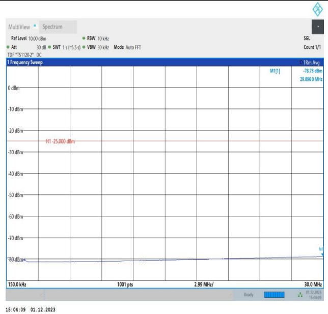
7-7-15MHz-10MHz-16QAM-16QAM-21051-21171-75RB#0-50 RB#0-0.15~30MHz-PASS
