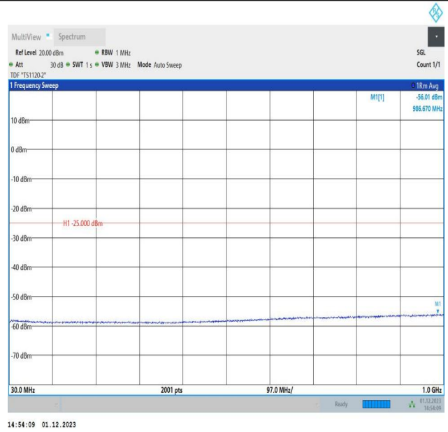
7-7-15MHz-10MHz-16QAM-16QAM-20825-20945-1RB#0-1RB #49-30~1000MHz-PASS
