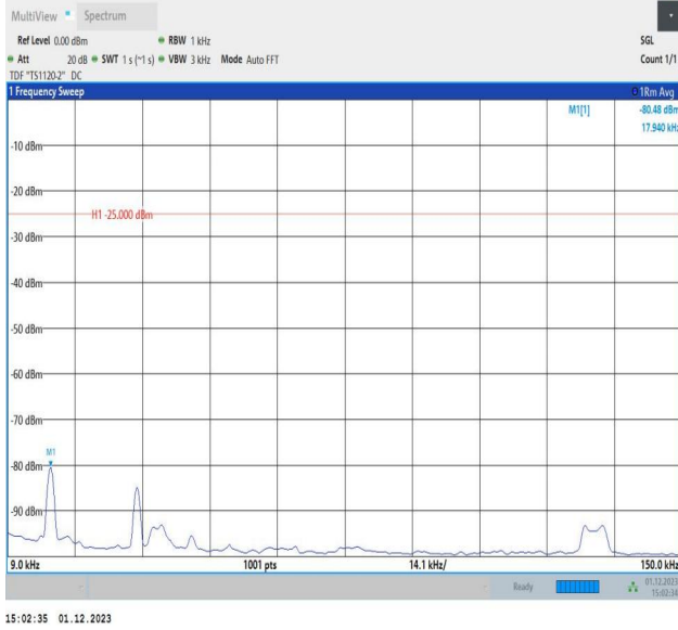
7-7-15MHz-10MHz-64QAM-64QAM-21051-21171-1RB#0-1RB #49-0.009~0.15MHz-PASS
