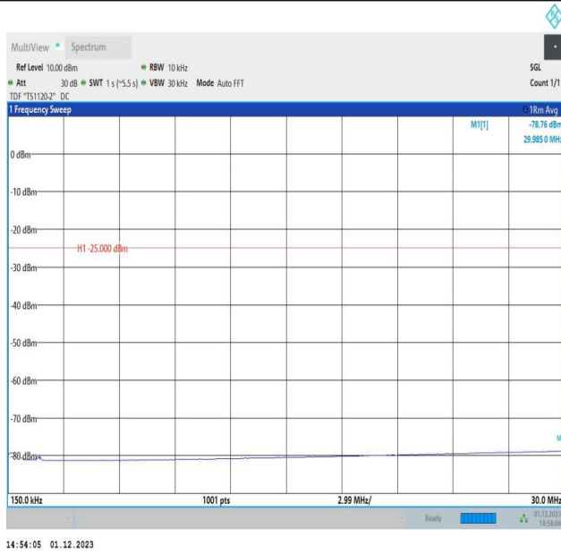
7-7-15MHz-10MHz-16QAM-16QAM-20825-20945-1RB#0-1RB #49-0.15~30MHz-PASS
