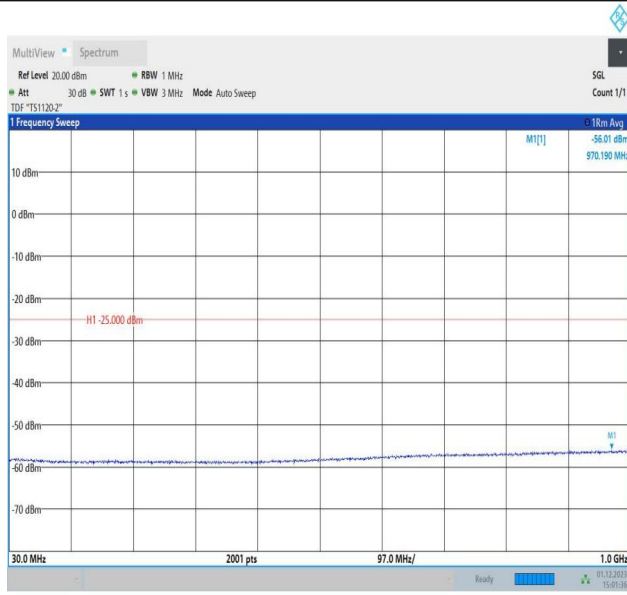
7-7-15MHz-10MHz-QPSK-QPSK-21051-21171-1RB#0-1RB#4 9-30~1000MHz-PASS
