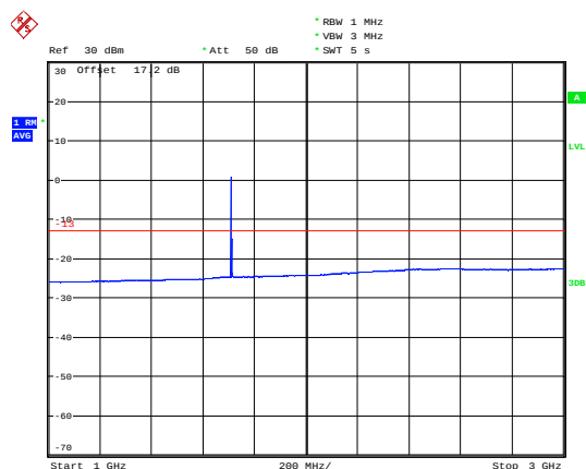
LTE Band 66 1.4MHz CH-Low 1GHz~3GHz
