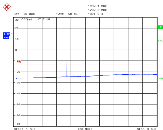
LTE Band 66 1.4MHz CH-Middle 1GHz~3GHz
