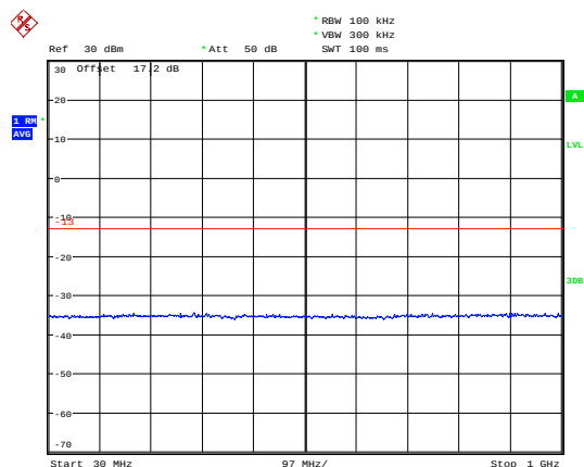
LTE Band 66 1.4MHz CH-Low 30MHz~1GHz
