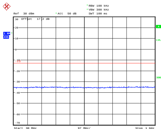
LTE Band 66 1.4MHz CH-Middle 30MHz~1GHz
