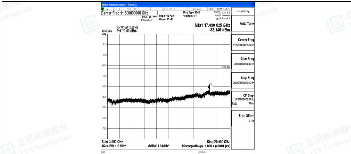
Band4_5MHz_16QAM_19975_1RB#0_3000~20000_3000~20000
