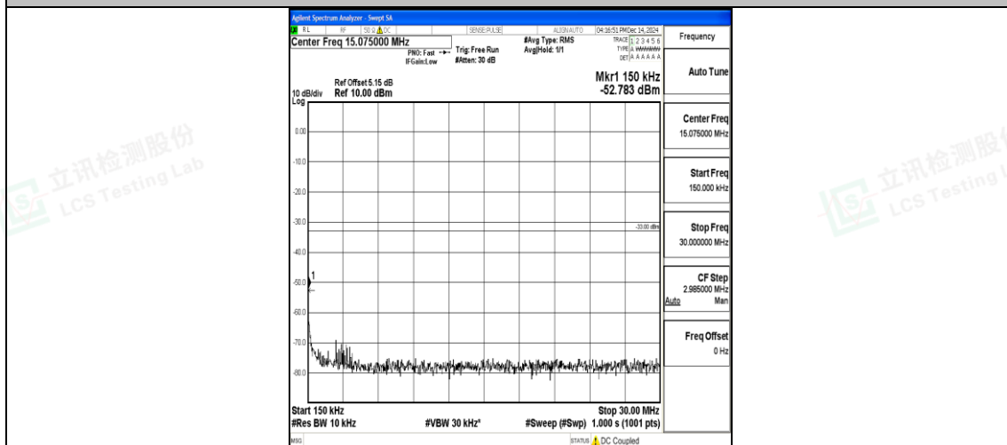
Band4_10MHz_QPSK_20175_1RB#0_0.15~30_0.15~30
