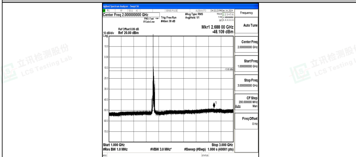
Band4_15MHz_16QAM_20025_1RB#0_1000~3000_1000~3000
