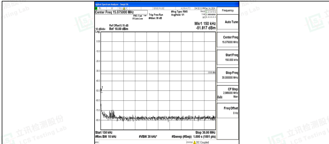
Band4_15MHz_16QAM_20025_1RB#0_0.15~30_0.15~30
