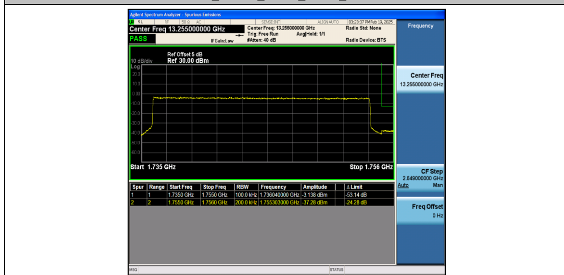
Band4_20MHz_QPSK_20300_100RB#0
