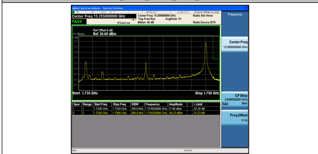
Band4_20MHz_QPSK_20300_1RB#99
