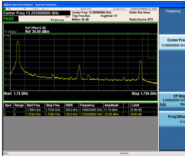
Band4_15MHz_16QAM_20325_1RB#0
