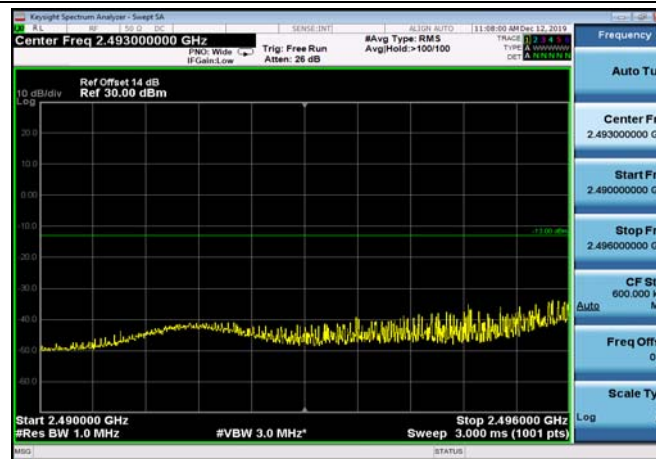
LowRange_FDD07_10MHz_2505_fullRB _Low_Q16
