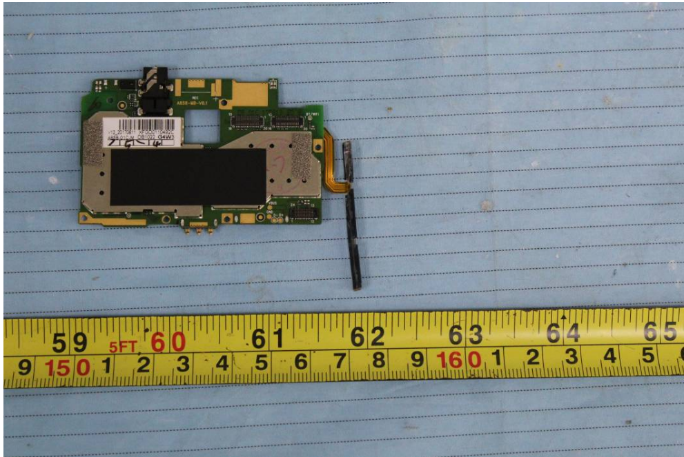
EUT – Mainboard 2 Bottom View 2
