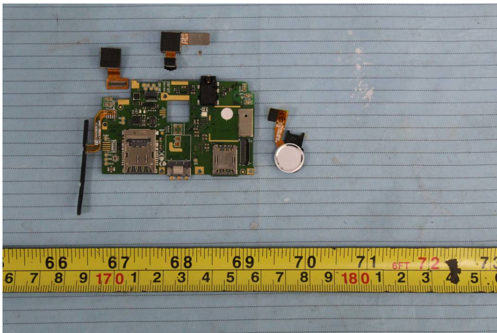
EUT – Mainboard 2 Top Cover off View
