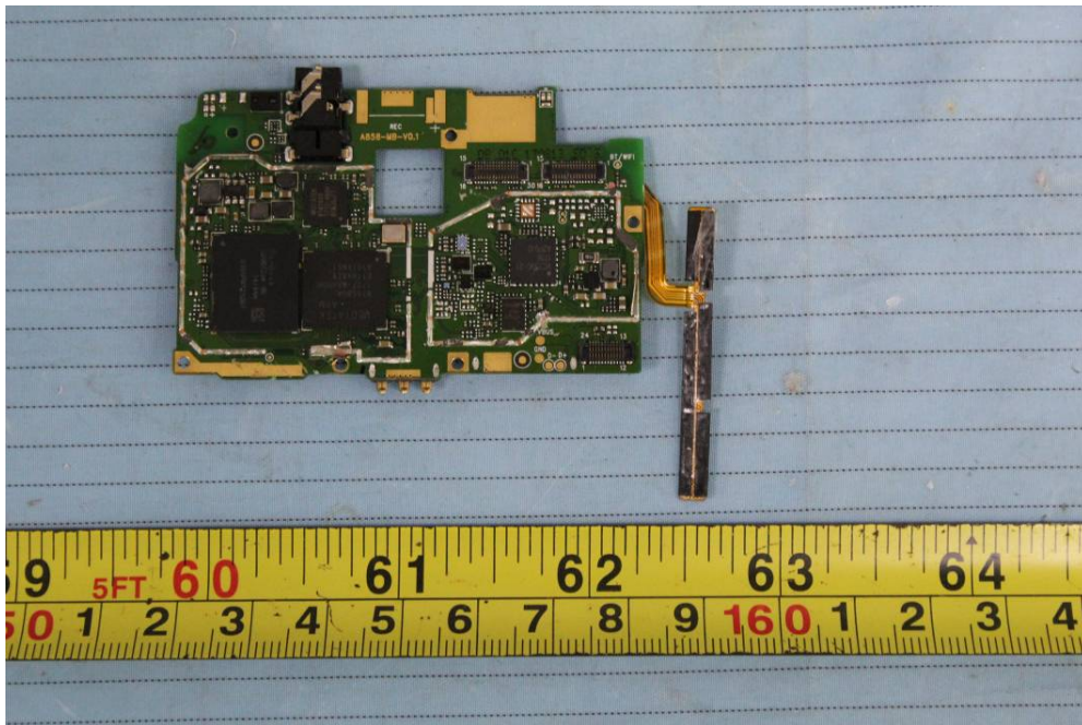
EUT – Mainboard 2 Bottom Shielding off View
