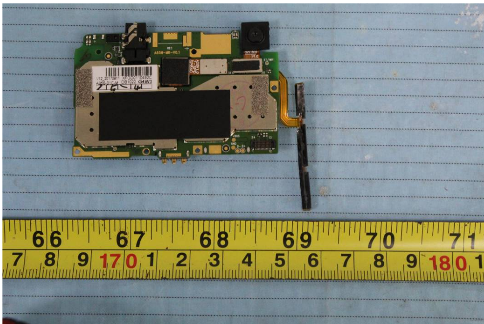
EUT – Mainboard 2 Bottom View 1
