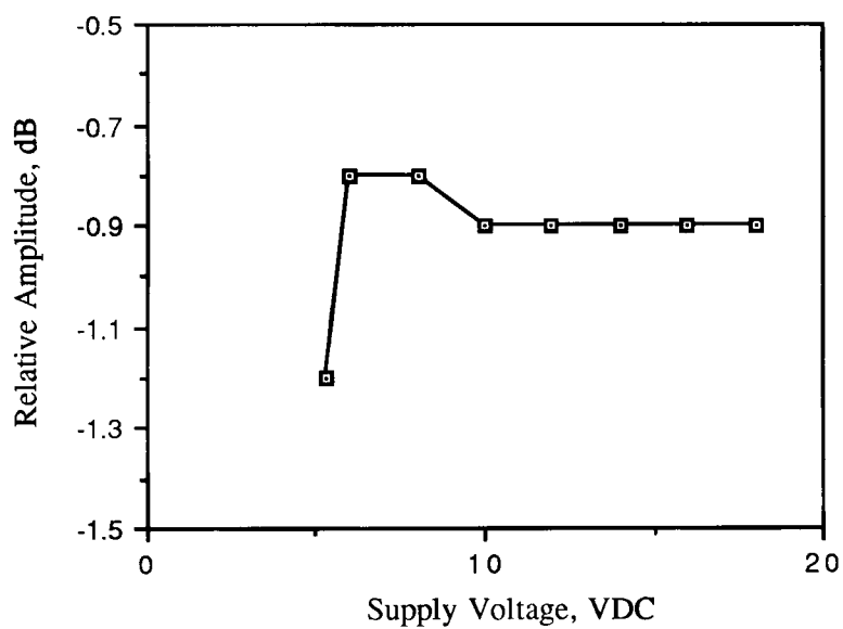
Figure 6.4. Relative emission at 125 kHz vs. supply voltage.
