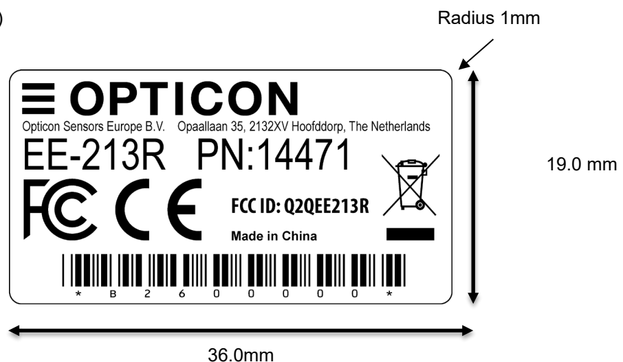
Figure 3: Product Label dimensions
