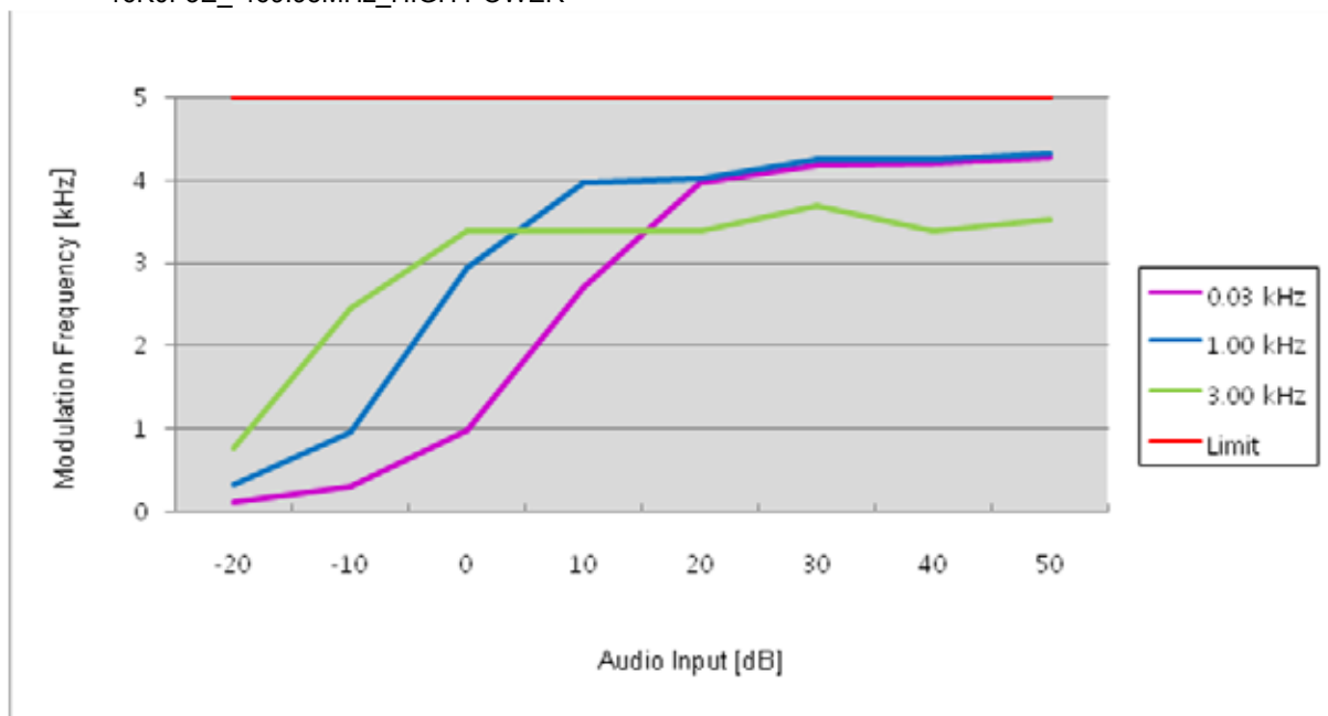
16K0F3E_469.95MHz_HIGH POWER
