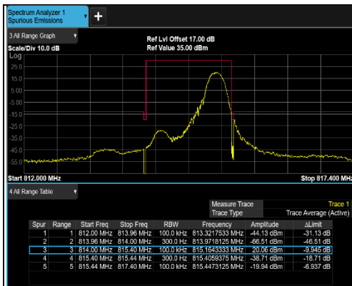
1RB#MAX (814.7MHz)
