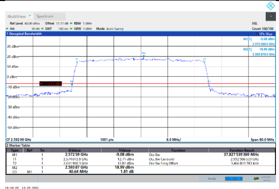
N41-30kHz-40MHz-CP-QPSK-Mid-Outer_Full---PASS
