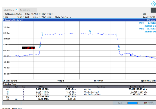
N41-30kHz-80MHz-DFT-QPSK-Mid-Outer_Full---PASS
