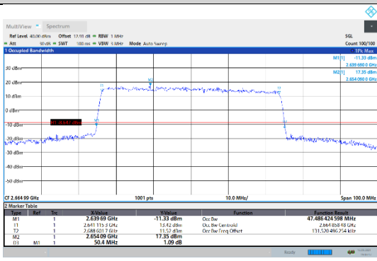
N41-30kHz-50MHz-CP-16QAM-High-Outer_Full---PASS
