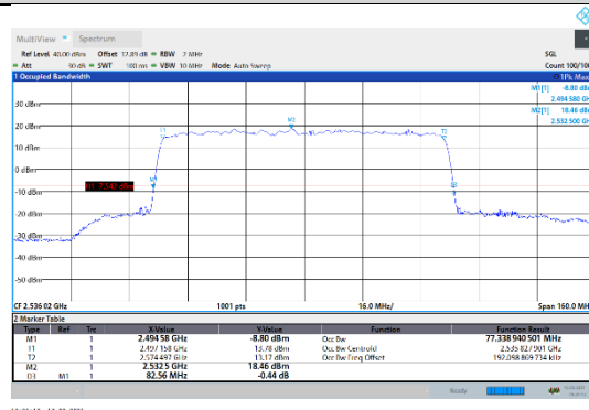
N41-30kHz-80MHz-DFT-64QAM-Low-Outer_Full---PASS
