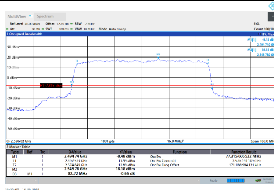
N41-30kHz-80MHz-CP-64QAM-Low-Outer_Full--- PASS
