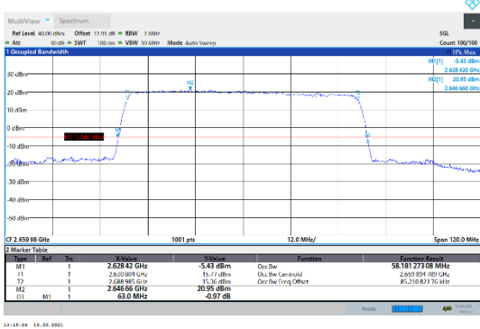
N41-30kHz-60MHz-DFT-QPSK-High-Outer_Full--- PASS
