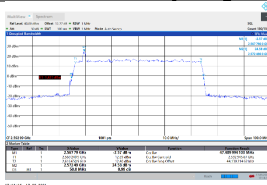
N41-30kHz-50MHz-CP-16QAM-Mid-Outer_Full---PASS
