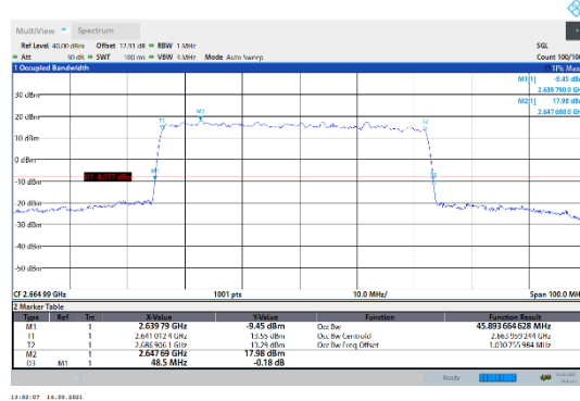
N41-30kHz-50MHz-DFT-64QAM-High-Outer_Full---PASS
