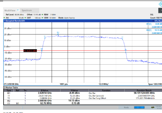
N41-30kHz-60MHz-DFT-256QAM-High-Outer_Full---PASS
