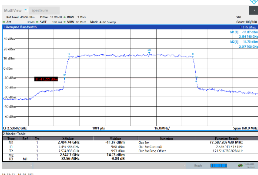
N41-30kHz-80MHz-CP-256QAM-Low-Outer_Full--- PASS
