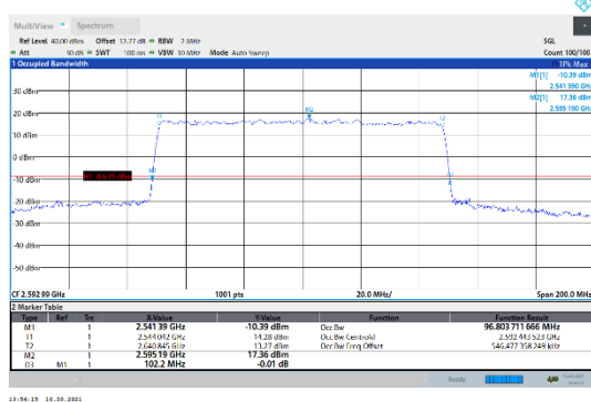
N41-30kHz-100MHz-DFT-64QAM-Mid-Outer_Full--- PASS
