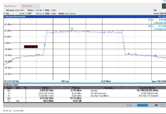
N41-30kHz-50MHz-DFT-QPSK-Low-Outer_Full---PASS
