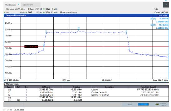
N41-30kHz-90MHz-CP-64QAM-Mid-Outer_Full--- PASS
