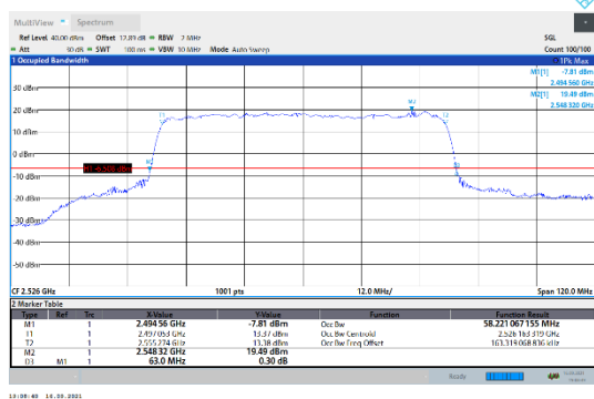
N41-30kHz-60MHz-CP-64QAM-Low-Outer_Full--- PASS
