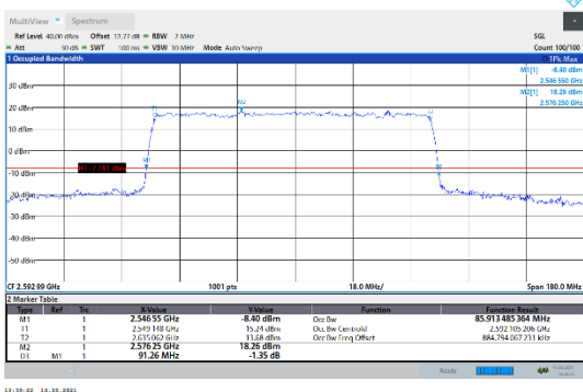
N41-30kHz-90MHz-DFT-16QAM-Mid-Outer_Full---PASS
