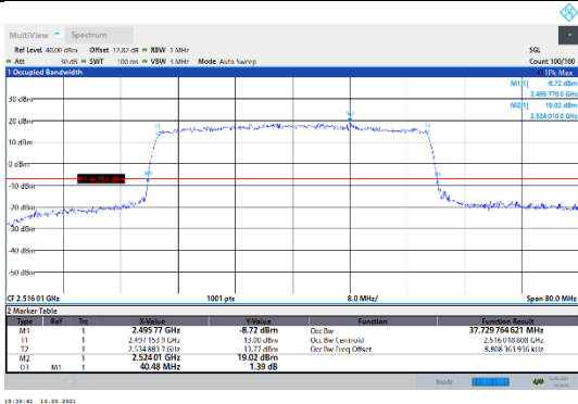
N41-30kHz-40MHz-CP-QPSK-Low-Outer_Full---PASS
