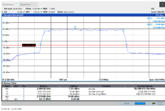
N41-30kHz-60MHz-DFT-64QAM-Low-Outer_Full--- PASS
