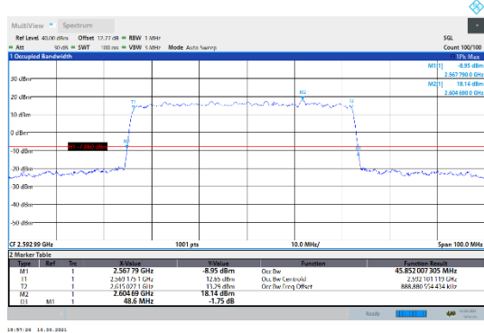
N41-30kHz-50MHz-DFT-64QAM-Mid-Outer_Full---PASS
