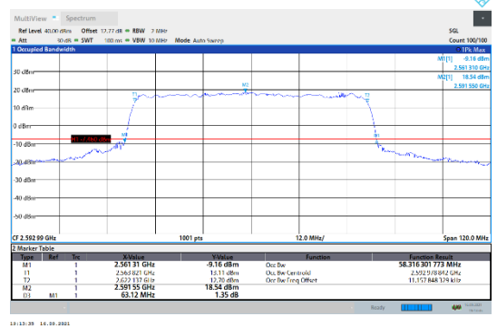
N41-30kHz-60MHz-CP-64QAM-Mid-Outer_Full--- PASS
