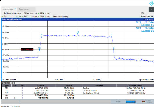
N41-30kHz-50MHz-DFT-256QAM-High-Outer_Full---PASS
