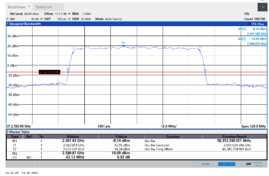
N41-30kHz-60MHz-DFT-64QAM-Mid-Outer_Full--- PASS
