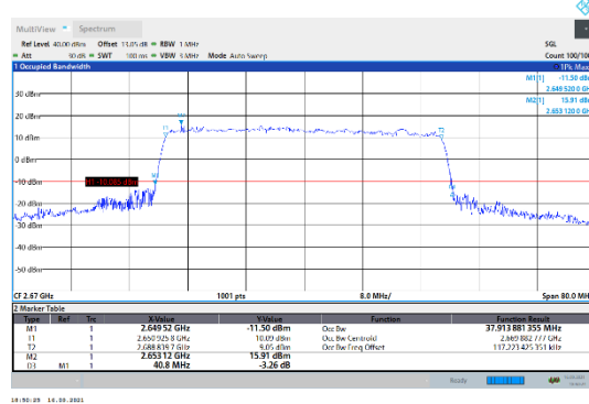
N41-30kHz-40MHz-CP-256QAM-High-Outer_Full---PASS
