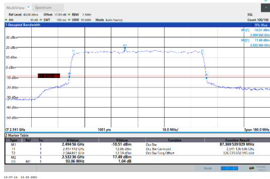
N41-30kHz-90MHz-CP-64QAM-Low-Outer_Full--- PASS
