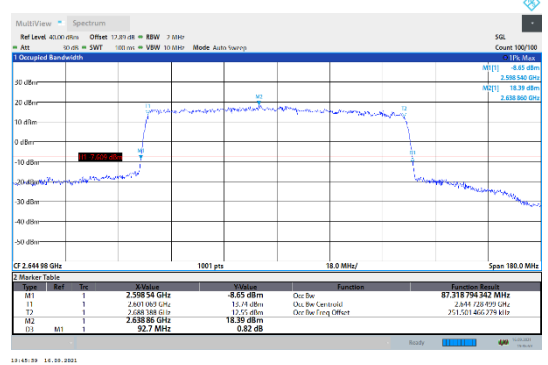
N41-30kHz-90MHz-CP-16QAM-High-Outer_Full--- PASS
