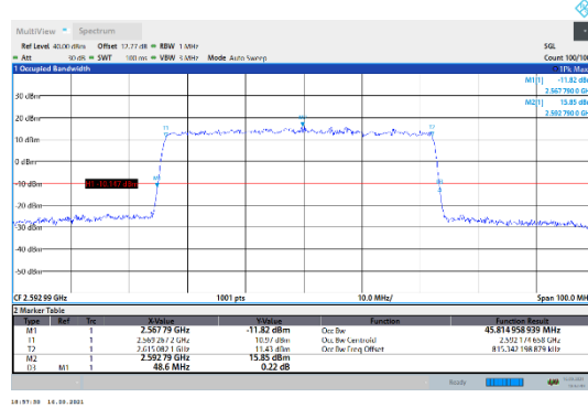
N41-30kHz-50MHz-DFT-256QAM-Mid-Outer_Full---PASS
