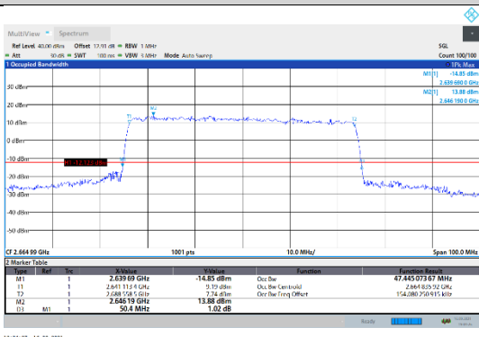
N41-30kHz-50MHz-CP-256QAM-High-Outer_Full--- PASS
