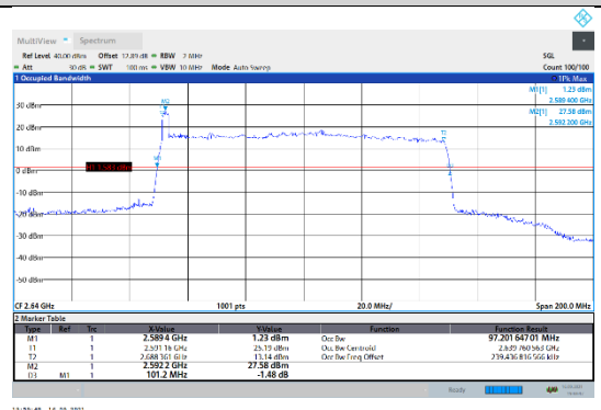
N41-30kHz-100MHz-CP-QPSK-High-Outer_Full--- PASS
