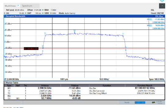
N41-30kHz-90MHz-CP-256QAM-High-Outer_Full--- PASS
