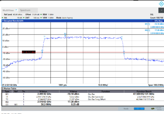
N41-30kHz-50MHz-CP-16QAM-Low-Outer_Full---PASS
