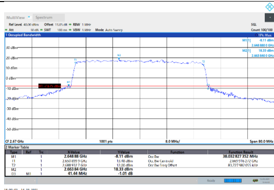
N41-30kHz-40MHz-CP-64QAM-High-Outer_Full---PASS
