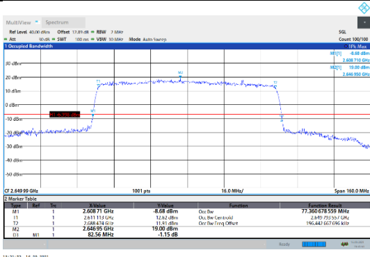
N41-30kHz-80MHz-CP-16QAM-High-Outer_Full--- PASS
