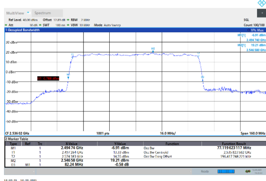
N41-30kHz-80MHz-DFT-16QAM-Low-Outer_Full---PASS
