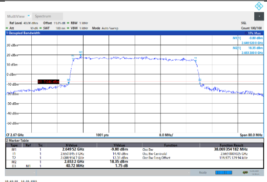
N41-30kHz-40MHz-CP-16QAM-High-Outer_Full---PASS
