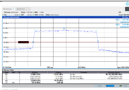
N41-30kHz-100MHz-DFT-256QAM-High-Outer_Full--- PASS
