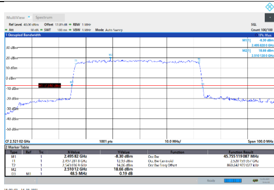
N41-30kHz-50MHz-DFT-16QAM-Low-Outer_Full---PASS
