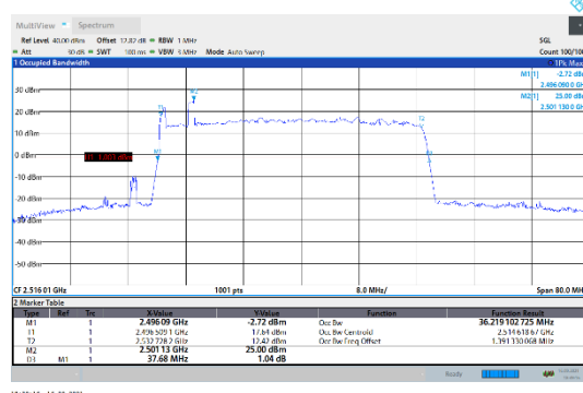
N41-30kHz-40MHz-DFT-256QAM-Low-Outer_Full--- PASS
