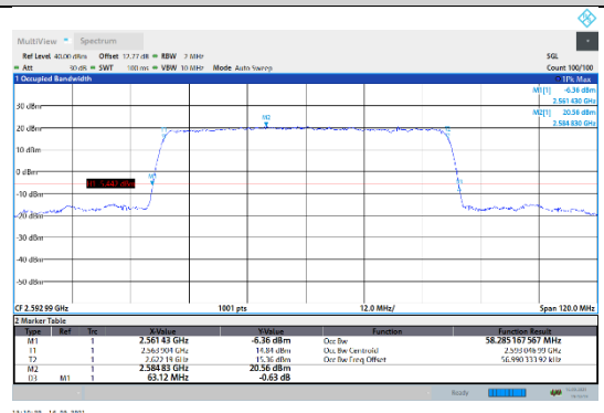
N41-30kHz-60MHz-DFT-QPSK-Mid-Outer_Full--- PASS
