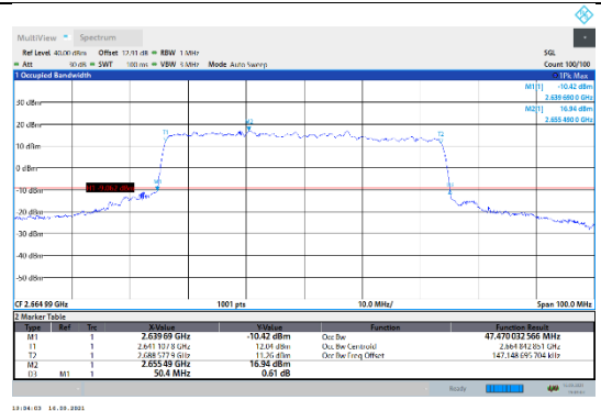
N41-30kHz-50MHz-CP-64QAM-High-Outer_Full--- PASS
