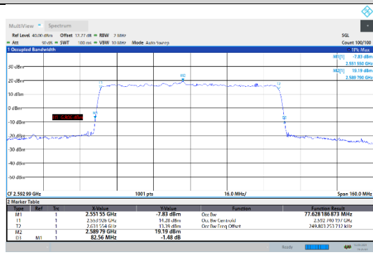
N41-30kHz-80MHz-DFT-64QAM-Mid-Outer_Full---PASS
