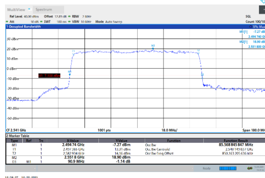
N41-30kHz-90MHz-DFT-16QAM-Low-Outer_Full---PASS
