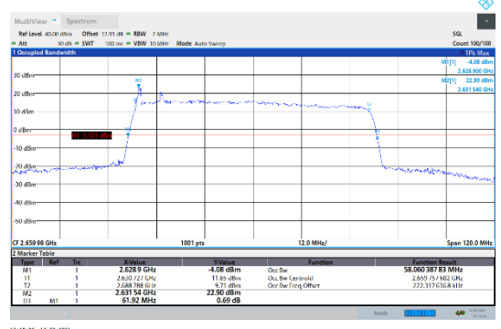
N41-30kHz-60MHz-CP-256QAM-High-Outer_Full--- PASS
