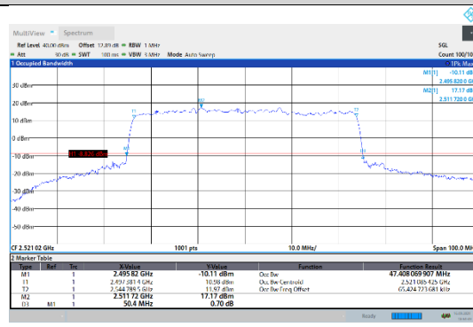
N41-30kHz-50MHz-CP-64QAM-Low-Outer_Full---PASS
