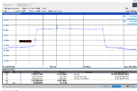
N41-30kHz-90MHz-CP-256QAM-Mid-Outer_Full--- PASS
