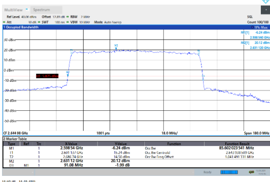
N41-30kHz-90MHz-DFT-QPSK-High-Outer_Full---PASS
