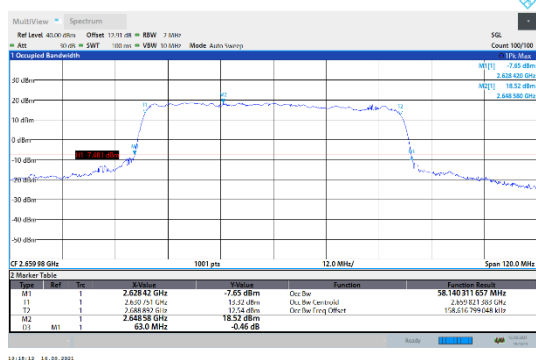
N41-30kHz-60MHz-CP-64QAM-High-Outer_Full--- PASS
