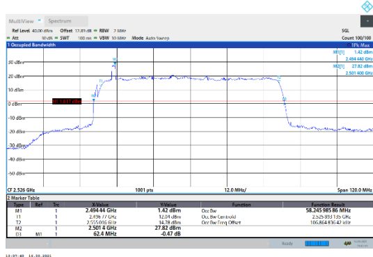
N41-30kHz-60MHz-CP-QPSK-Low-Outer_Full---PASS
