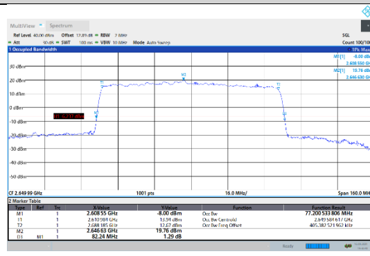
N41-30kHz-80MHz-DFT-64QAM-High-Outer_Full---PASS
