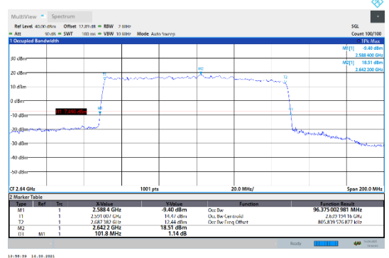
N41-30kHz-100MHz-DFT-64QAM-High-Outer_Full--- PASS
