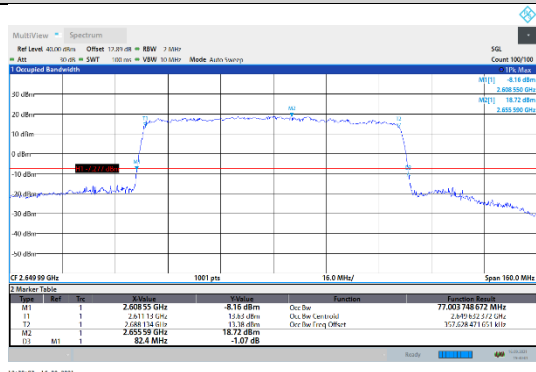
N41-30kHz-80MHz-DFT-16QAM-High-Outer_Full---PASS
