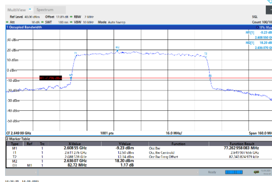
N41-30kHz-80MHz-CP-64QAM-High-Outer_Full--- PASS
