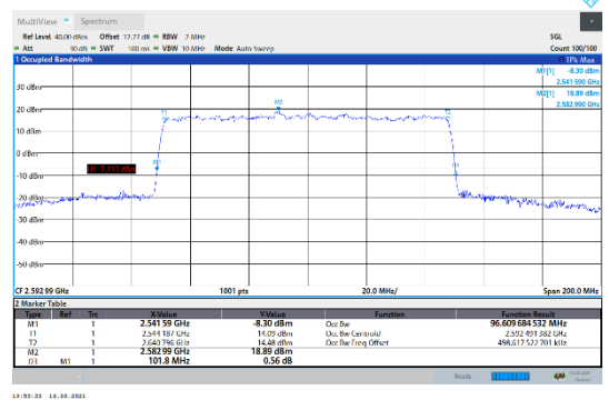
N41-30kHz-100MHz-DFT-16QAM-Mid-Outer_Full---PASS
