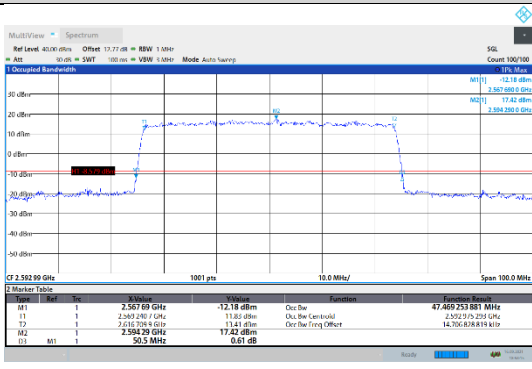
N41-30kHz-50MHz-CP-QPSK-Mid-Outer_Full---PASS
