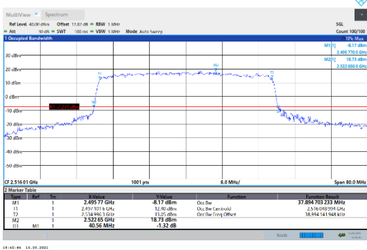
N41-30kHz-40MHz-CP-64QAM-Low-Outer_Full---PASS
