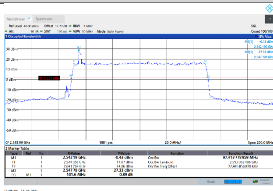
N41-30kHz-100MHz-CP-QPSK-Mid-Outer_Full--- PASS
