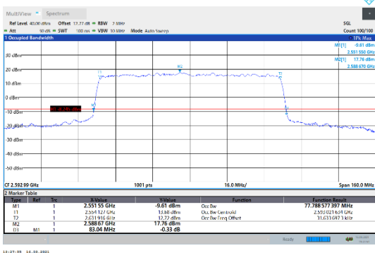
N41-30kHz-80MHz-CP-64QAM-Mid-Outer_Full--- PASS
