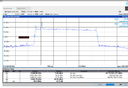
N41-30kHz-50MHz-CP-QPSK-High-Outer_Full---PASS
