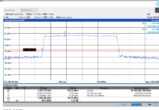
N41-30kHz-50MHz-DFT-16QAM-Mid-Outer_Full---PASS
