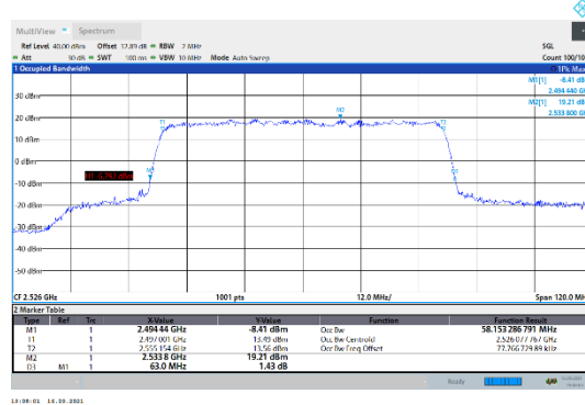
N41-30kHz-60MHz-CP-16QAM-Low-Outer_Full---PASS
