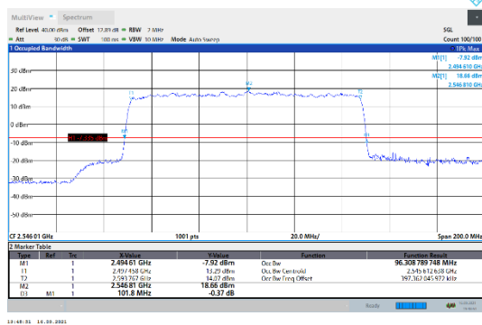
N41-30kHz-100MHz-DFT-16QAM-Low-Outer_Full---PASS
