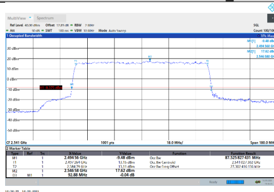
N41-30kHz-90MHz-CP-16QAM-Low-Outer_Full---PASS
