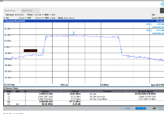
N41-30kHz-40MHz-DFT-16QAM-High-Outer_Full--- PASS
