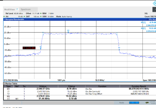
N41-30kHz-90MHz-DFT-QPSK-Mid-Outer_Full---PASS
