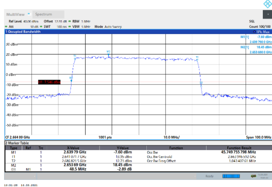
N41-30kHz-50MHz-DFT-16QAM-High-Outer_Full---PASS
