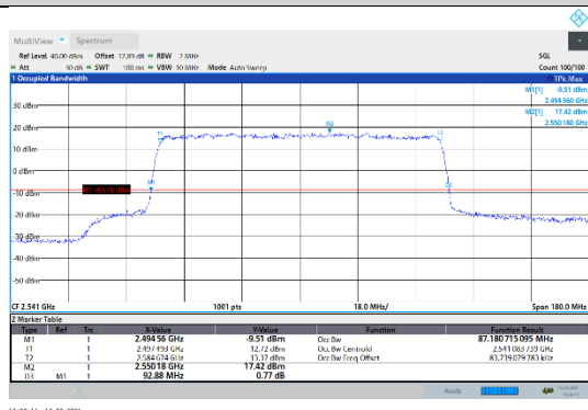
N41-30kHz-90MHz-CP-QPSK-Low-Outer_Full---PASS
