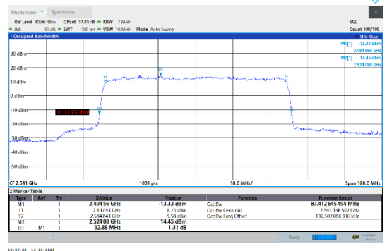
N41-30kHz-90MHz-CP-256QAM-Low-Outer_Full--- PASS
