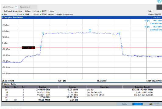
N41-30kHz-90MHz-DFT-64QAM-Low-Outer_Full---PASS
