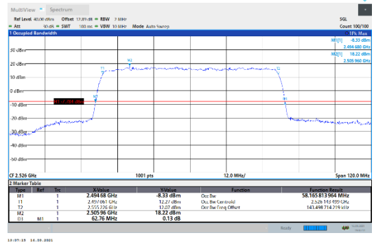
N41-30kHz-60MHz-DFT-256QAM-Low-Outer_Full--- PASS
