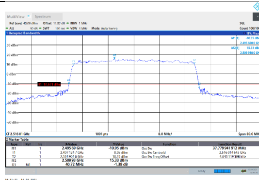
N41-30kHz-40MHz-CP-256QAM-Low-Outer_Full---PASS
