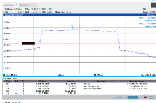
N41-30kHz-90MHz-CP-64QAM-High-Outer_Full--- PASS
