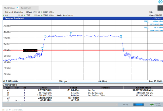
N41-30kHz-40MHz-CP-256QAM-Mid-Outer_Full---PASS
