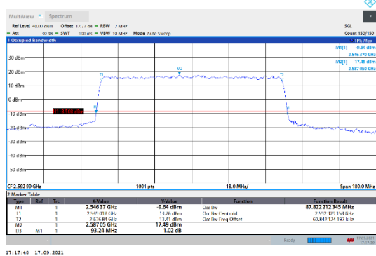
N41-30kHz-90MHz-CP-16QAM-Mid-Outer_Full--- PASS
