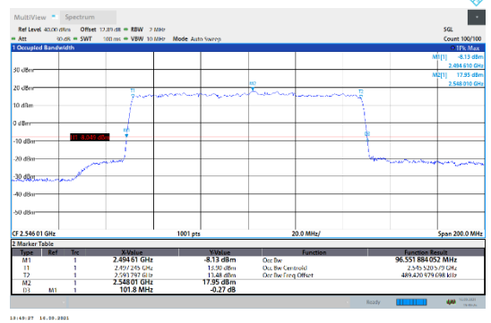
N41-30kHz-100MHz-DFT-64QAM-Low-Outer_Full---PASS
