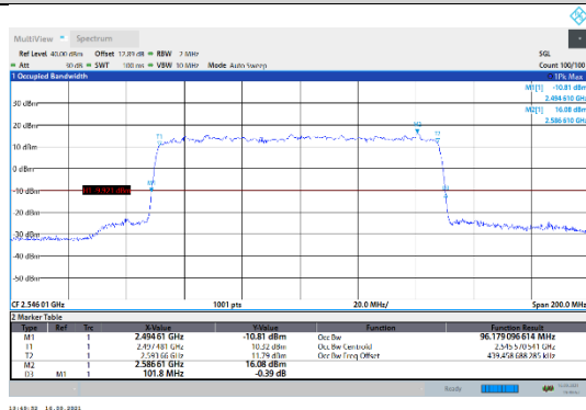
N41-30kHz-100MHz-DFT-256QAM-Low-Outer_Full--- PASS
