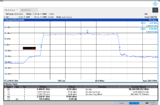
N41-30kHz-100MHz-DFT-QPSK-Low-Outer_Full---PASS
