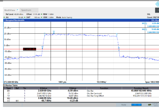
N41-30kHz-50MHz-DFT-QPSK-High-Outer_Full---PASS
