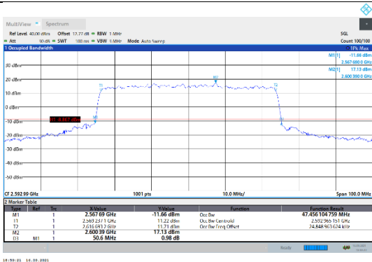
N41-30kHz-50MHz-CP-64QAM-Mid-Outer_Full--- PASS
