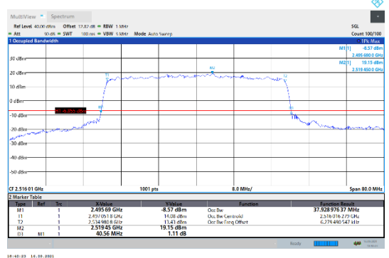
N41-30kHz-40MHz-CP-16QAM-Low-Outer_Full---PASS
