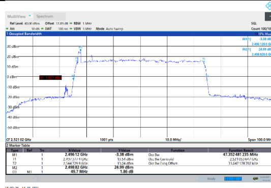
N41-30kHz-50MHz-CP-QPSK-Low-Outer_Full---PASS
