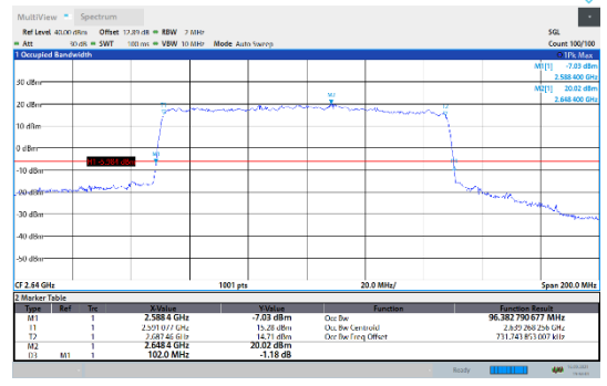
N41-30kHz-100MHz-DFT-QPSK-High-Outer_Full---PASS
