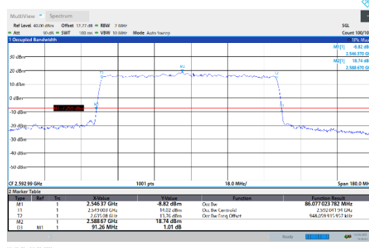
N41-30kHz-90MHz-DFT-64QAM-Mid-Outer_Full---PASS
