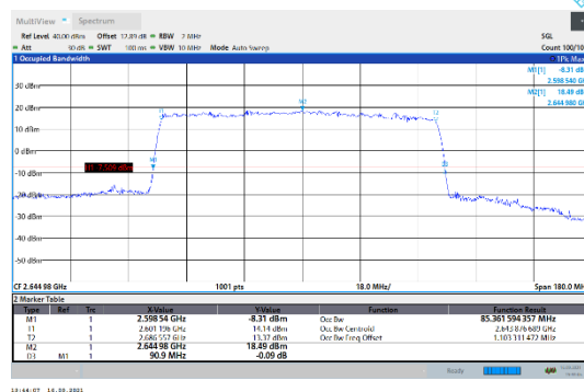
N41-30kHz-90MHz-DFT-16QAM-High-Outer_Full---PASS
