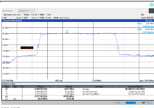
N41-30kHz-60MHz-DFT-QPSK-Low-Outer_Full--- PASS
