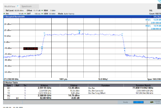
N41-30kHz-80MHz-CP-256QAM-Mid-Outer_Full--- PASS
