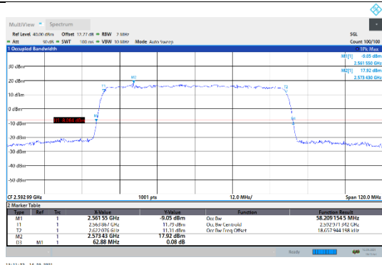
N41-30kHz-60MHz-DFT-256QAM-Mid-Outer_Full---PASS
