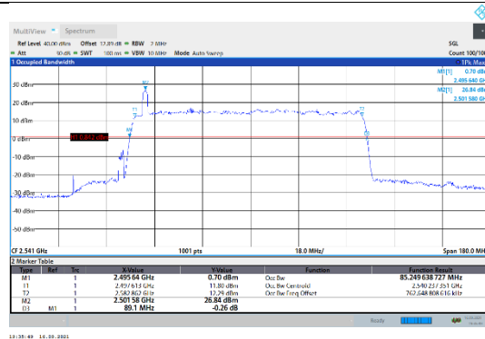
N41-30kHz-90MHz-DFT-256QAM-Low-Outer_Full---PASS
