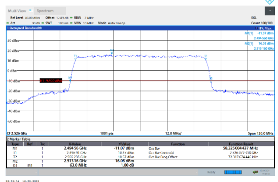
N41-30kHz-60MHz-CP-256QAM-Low-Outer_Full--- PASS
