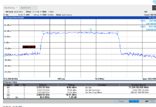
N41-30kHz-80MHz-DFT-16QAM-Mid-Outer_Full---PASS
