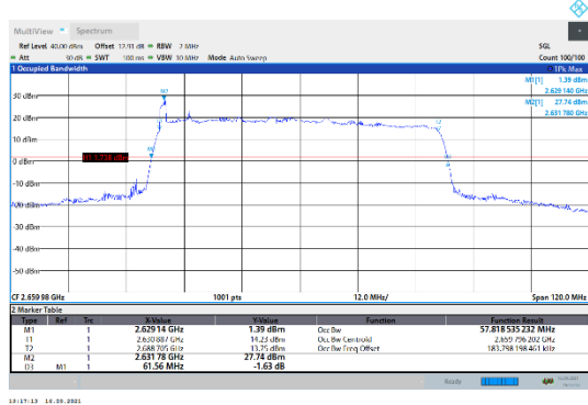
N41-30kHz-60MHz-CP-QPSK-High-Outer_Full---PASS
