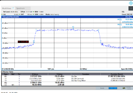
N41-30kHz-40MHz-CP-16QAM-Mid-Outer_Full---PASS
