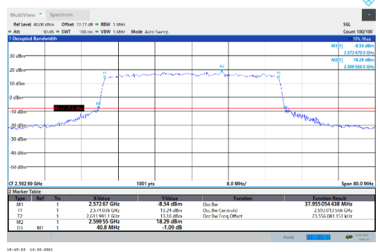
N41-30kHz-40MHz-CP-64QAM-Mid-Outer_Full---PASS
