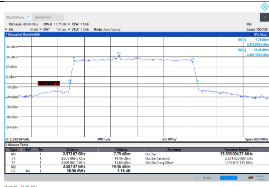
N41-30kHz-40MHz-DFT-16QAM-Mid-Outer_Full--- PASS
