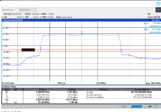
N41-30kHz-90MHz-DFT-QPSK-Low-Outer_Full---PASS
