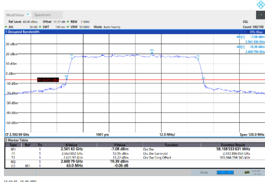
N41-30kHz-60MHz-CP-16QAM-Mid-Outer_Full---PASS
