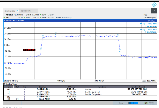
N41-30kHz-100MHz-CP-QPSK-Low-Outer_Full--- PASS
