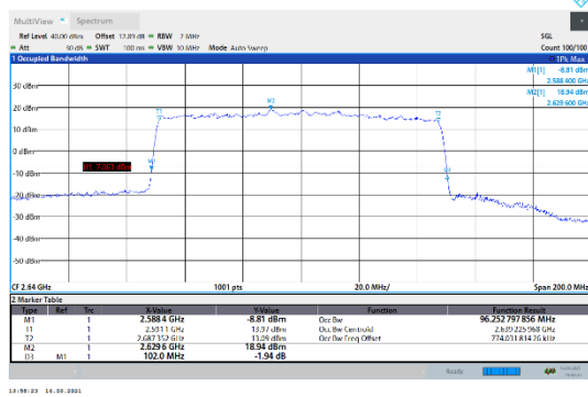
N41-30kHz-100MHz-DFT-16QAM-High-Outer_Full---PASS
