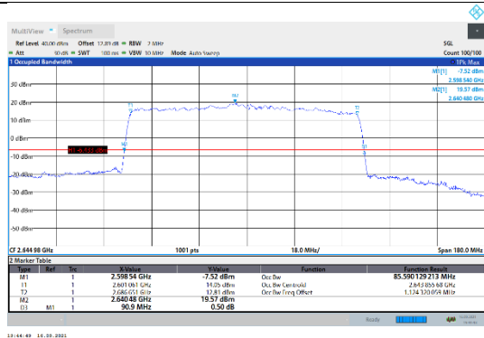
N41-30kHz-90MHz-DFT-64QAM-High-Outer_Full---PASS
