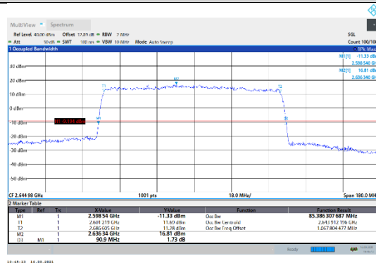
N41-30kHz-90MHz-DFT-256QAM-High-Outer_Full---PASS
