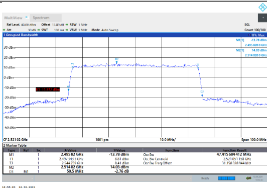
N41-30kHz-50MHz-CP-256QAM-Low-Outer_Full--- PASS
