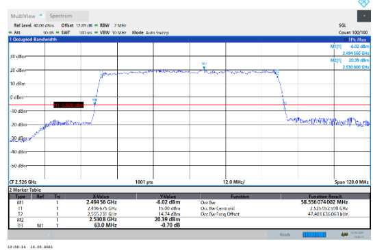
N41-30kHz-60MHz-DFT-16QAM-Low-Outer_Full--- PASS
