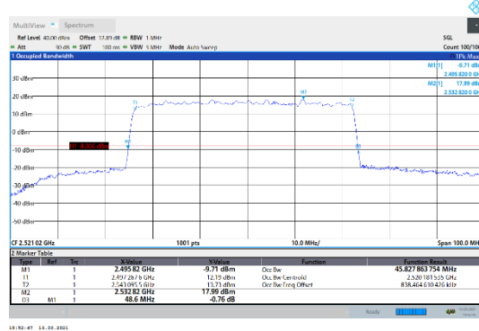
N41-30kHz-50MHz-DFT-64QAM-Low-Outer_Full---PASS
