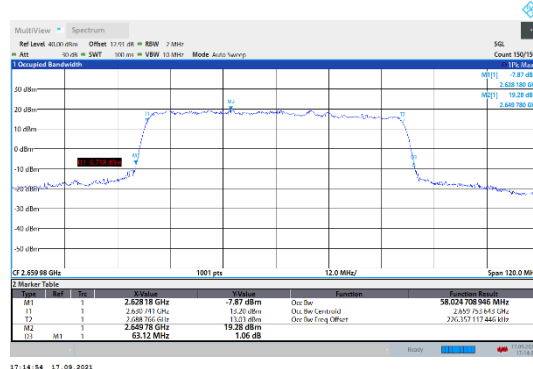
N41-30kHz-60MHz-CP-16QAM-High-Outer_Full---PASS
