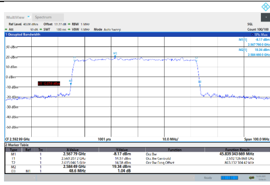
N41-30kHz-50MHz-DFT-QPSK-Mid-Outer_Full---PASS
