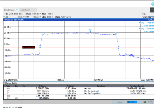
N41-30kHz-80MHz-DFT-QPSK-High-Outer_Full---PASS
