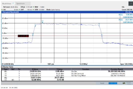
N41-30kHz-60MHz-DFT-64QAM-High-Outer_Full--- PASS
