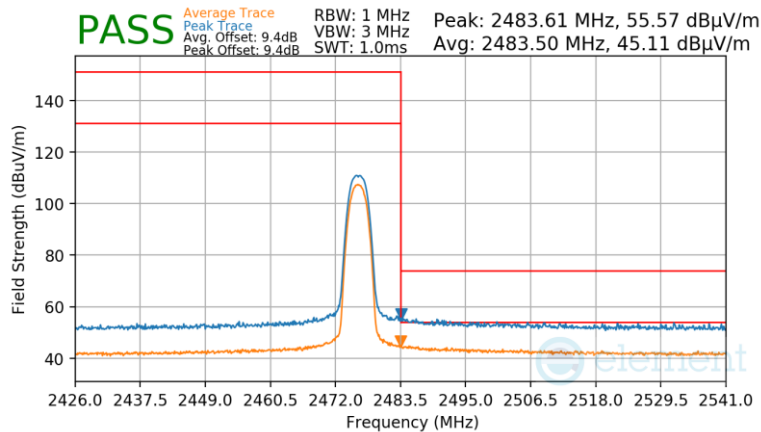
Plot 7-122. Radiated Restricted Upper Band Edge Measurement Antenna WF7
