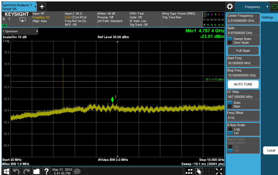
Plot 7-95. Conducted Spurious Plot Antenna WF7 (Bluetooth (HDR4), 4 Mbps, ePA – Ch. 73)
