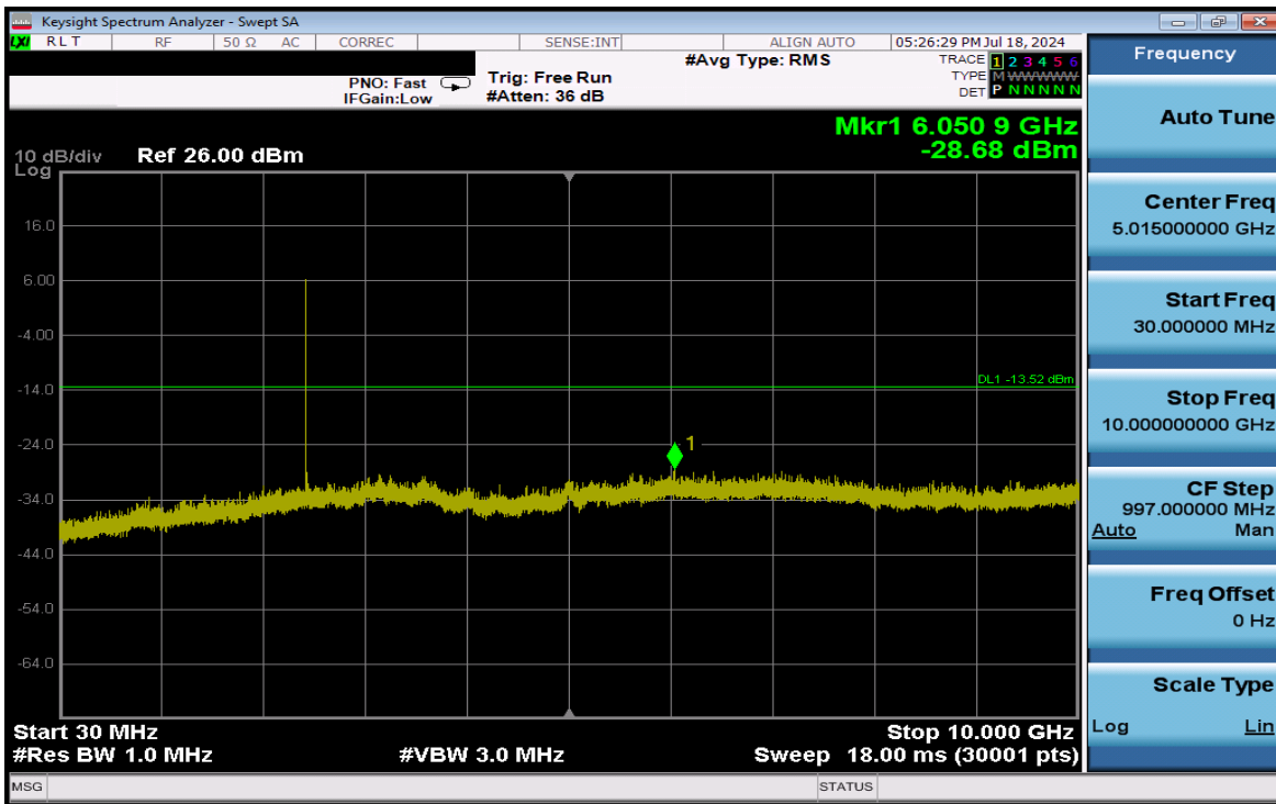
Plot 7-99. Conducted Spurious Plot Antenna WF2 (Bluetooth (HDR4), 4 Mbps, iPA – Ch. 38)
