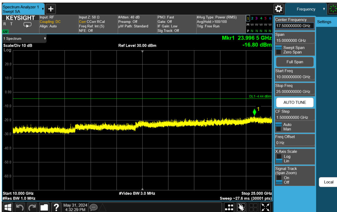
Plot 7-88. Conducted Spurious Plot Antenna WF8 (Bluetooth (HDR4), 4 Mbps, ePA – Ch. 38)
