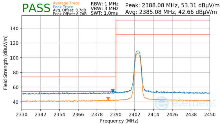
Plot 7-120. Radiated Restricted Lower Band Edge Measurement Antenna WF7
