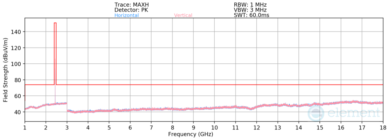
Plot 7-107. Radiated Spurious Emissions 1-18GHz Antenna WF7 (4Mbps, HDR4, ePA – Ch. 38)
