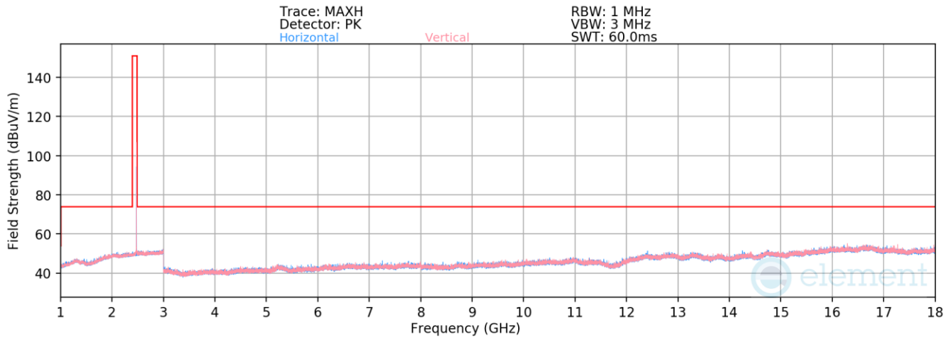
Plot 7-108. Radiated Spurious Emissions 1-18GHz Antenna WF7 (4Mbps, HDR4, ePA – Ch. 73)
