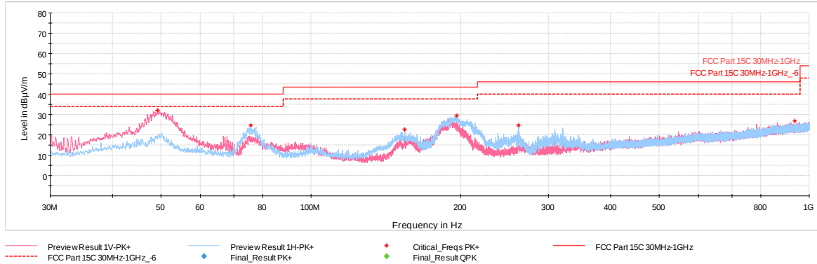
Plot 7-132. Radiated Spurious Emissions Below 1GHz TxBF (4Mbps, ePA – Ch.38 with AC/DC adaptor via USB-C cable with wire charger)
