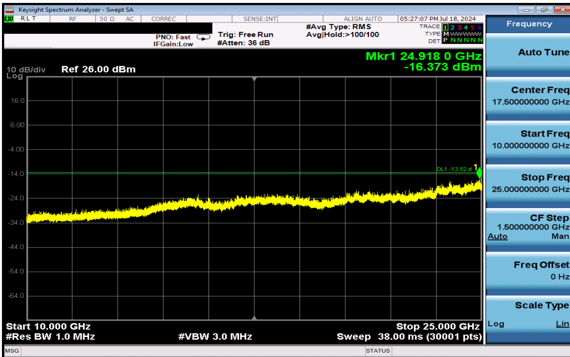
Plot 7-100. Conducted Spurious Plot Antenna WF2 (Bluetooth (HDR4), 4 Mbps, iPA – Ch. 38)
