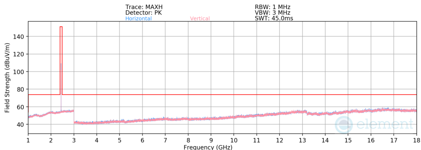
Plot 7-104. Radiated Spurious Emissions 1-18GHz Antenna WF8 (4Mbps, HDR4, ePA – Ch. 38)
