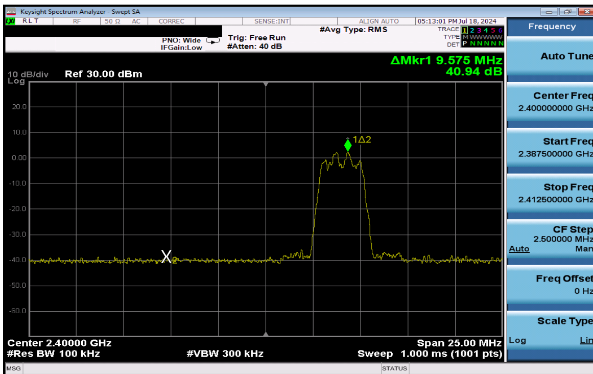
Plot 7-81. Band Edge Plot Antenna WF2 (Bluetooth (HDR4), iPA – Ch. 1)
