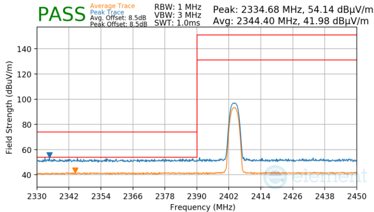
Plot 7-116. Radiated Restricted Lower Band Edge Measurement Antenna WF8
