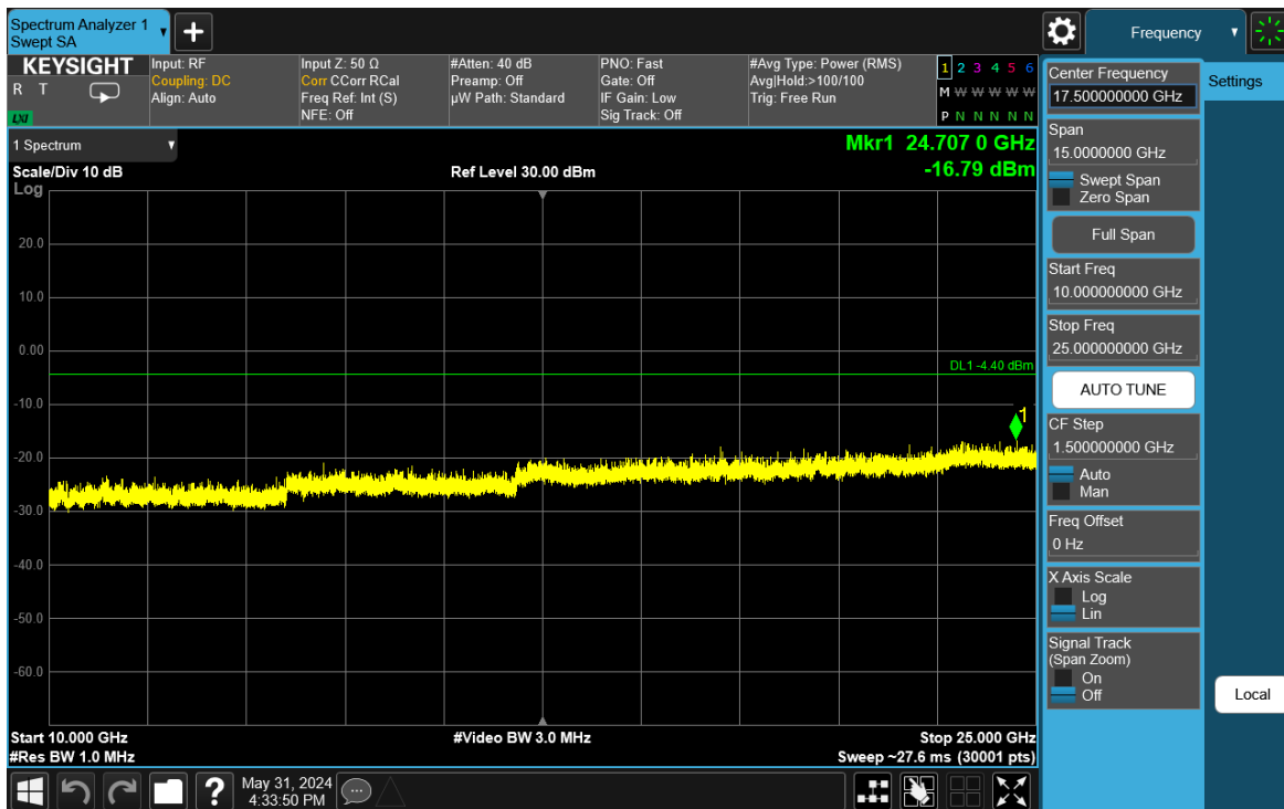
Plot 7-90. Conducted Spurious Plot Antenna WF8 (Bluetooth (HDR4), 4 Mbps, ePA – Ch. 73)
