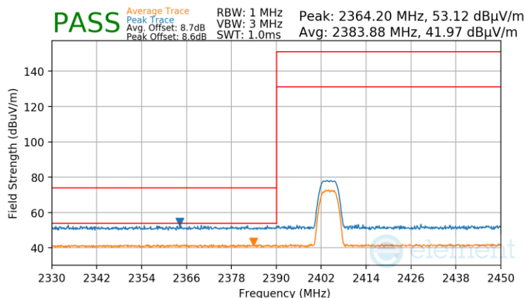
Plot 7-125. Radiated Restricted Lower Band Edge Measurement Antenna WF2
