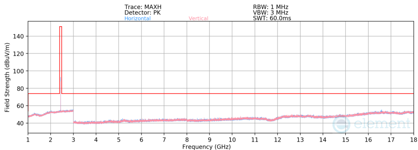
Plot 7-110. Radiated Spurious Emissions 1-18GHz Antenna WF2 (4Mbps, HDR4, iPA – Ch. 38)
