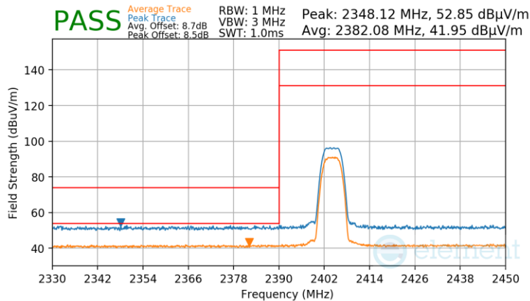
Plot 7-117. Radiated Restricted Lower Band Edge Measurement Antenna WF8
