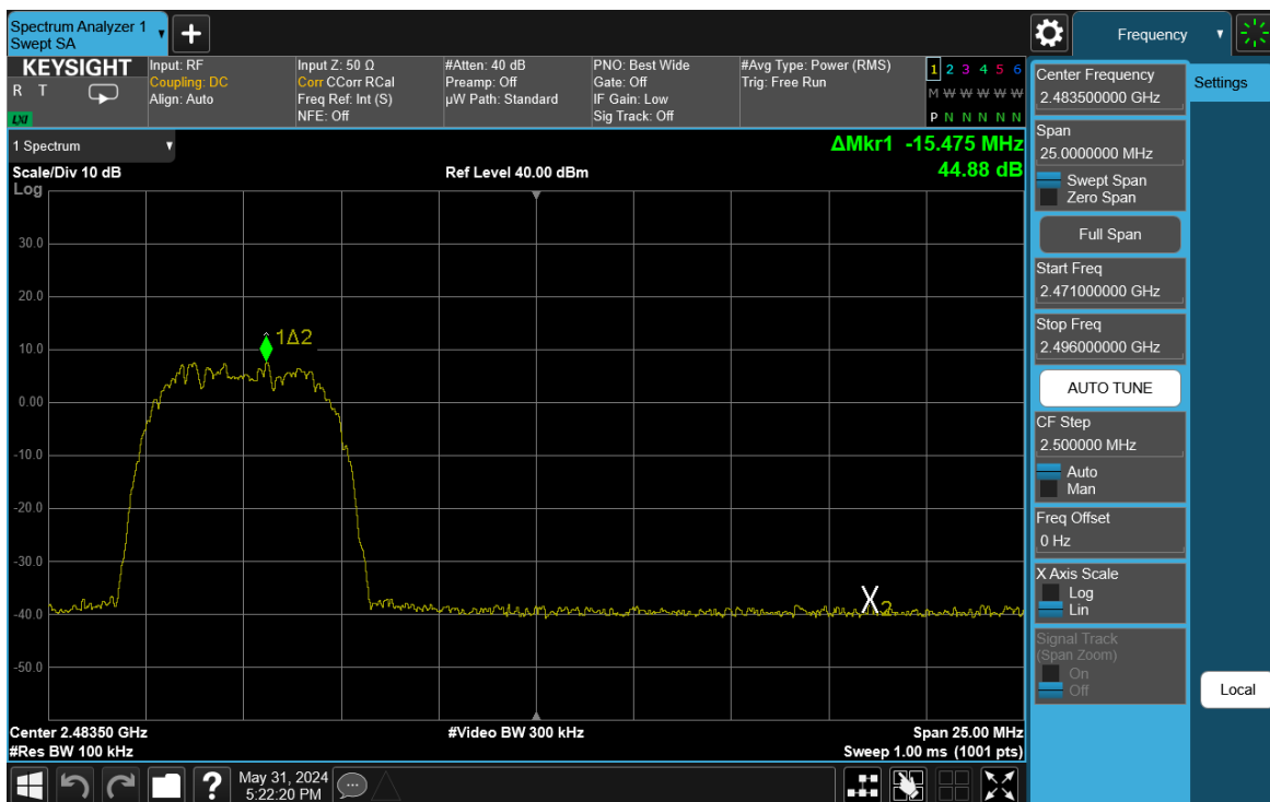
Plot 7-80. Band Edge Plot Antenna WF7 (Bluetooth (HDR8), ePA – Ch. 73)
