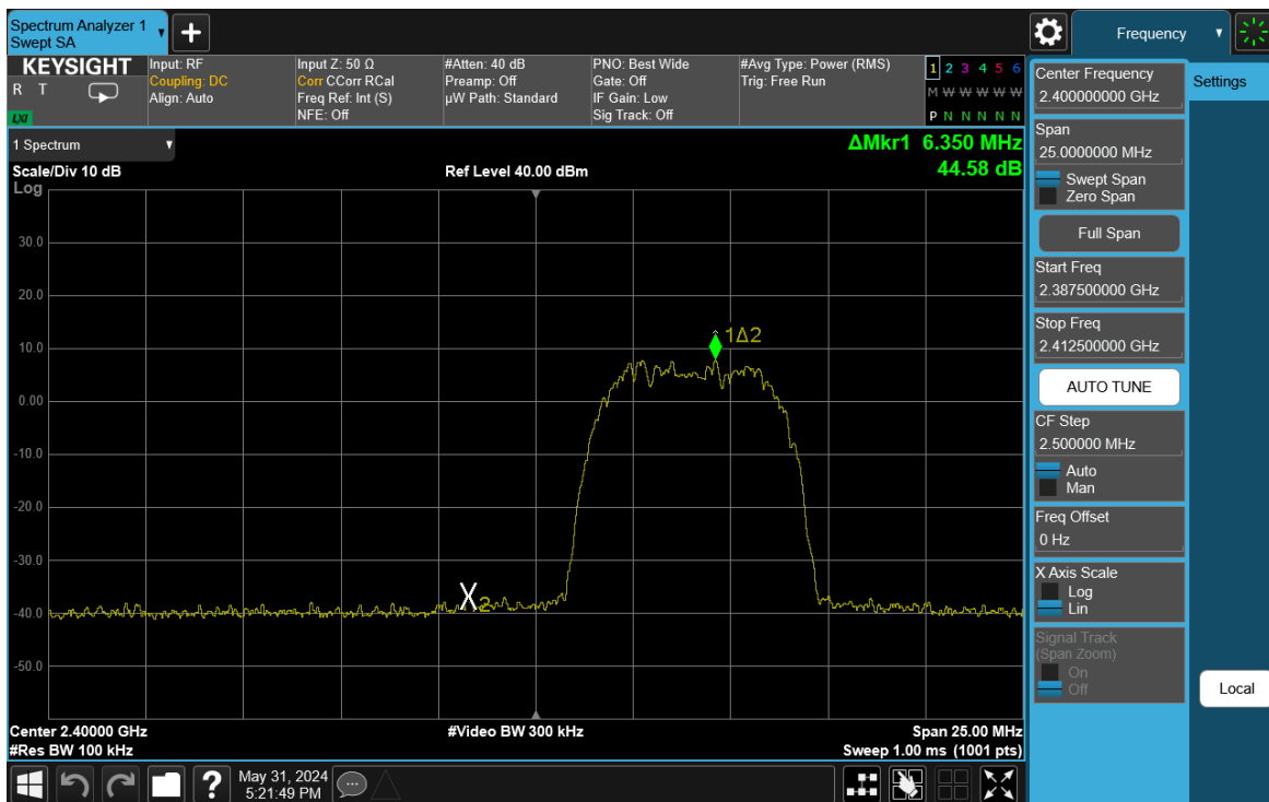
Plot 7-79. Band Edge Plot Antenna WF7 (Bluetooth (HDR8), ePA – Ch. 1)
