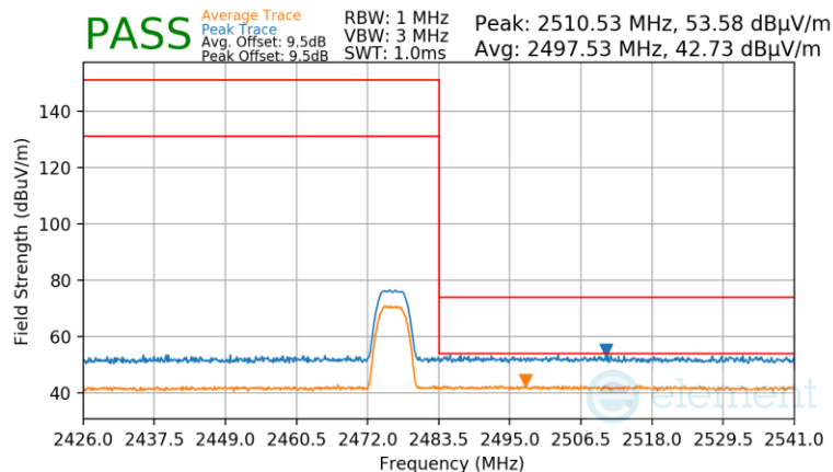
Plot 7-127. Radiated Restricted Upper Band Edge Measurement Antenna WF2
