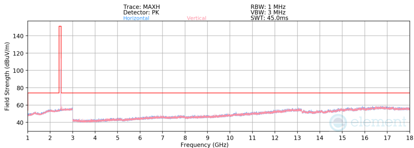
Plot 7-115. Radiated Spurious Emissions 1-18GHz TxBF (4Mbps, HDR4, ePA – Ch. 73)
