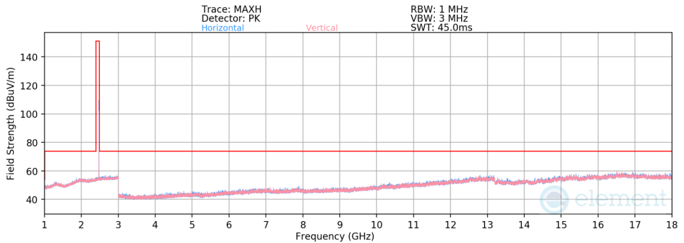
Plot 7-105. Radiated Spurious Emissions 1-18GHz Antenna WF8 (4Mbps, HDR4, ePA – Ch. 73)
