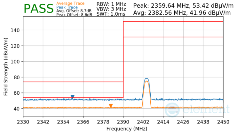
Plot 7-124. Radiated Restricted Lower Band Edge Measurement Antenna WF2
