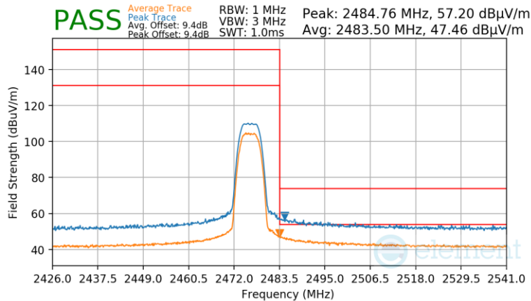
Plot 7-123. Radiated Restricted Upper Band Edge Measurement Antenna WF7
