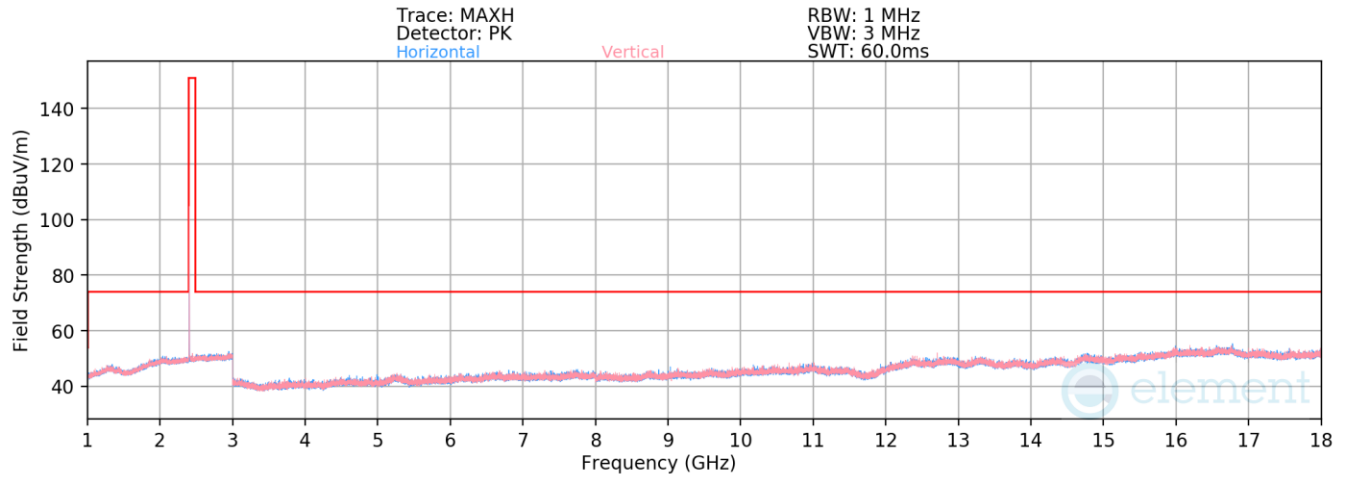
Plot 7-106. Radiated Spurious Emissions 1-18GHz Antenna WF7 (4Mbps, HDR4, ePA – Ch. 1)
