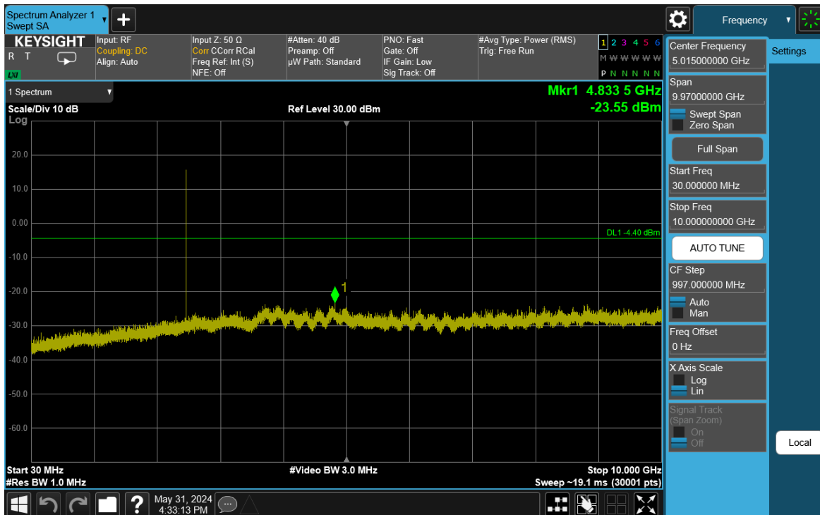
Plot 7-89. Conducted Spurious Plot Antenna WF8 (Bluetooth (HDR4), 4 Mbps, ePA – Ch. 73)
