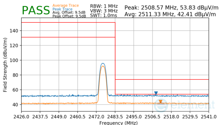
Plot 7-118. Radiated Restricted Upper Band Edge Measurement Antenna WF8
