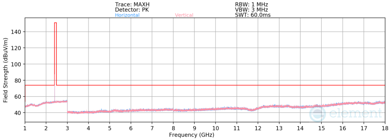
Plot 7-109. Radiated Spurious Emissions 1-18GHz Antenna WF2 (4Mbps, HDR4, iPA – Ch. 1)
