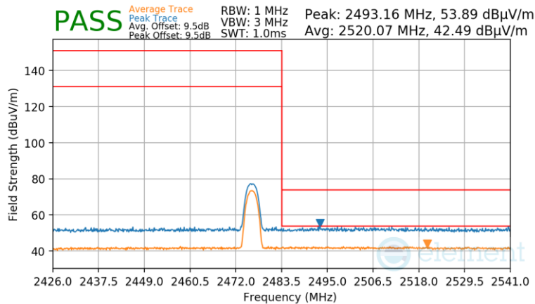
Plot 7-126. Radiated Restricted Upper Band Edge Measurement Antenna WF2
