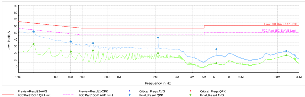
Plot 7-133. AC Line Conducted Plot with Bluetooth HDR Tx BF (L1, 4Mbps ePA - Ch.38 with host PC via USB-C cable with wire charger)
