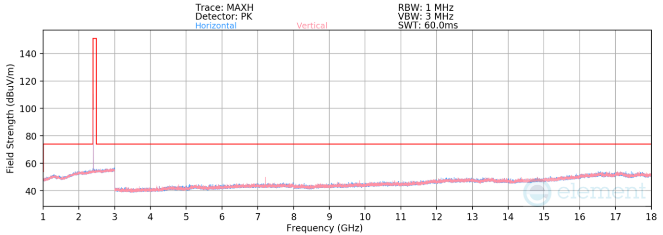
Plot 7-103. Radiated Spurious Emissions 1-18GHz Antenna WF8 (4Mbps, HDR4, ePA – Ch. 1)
