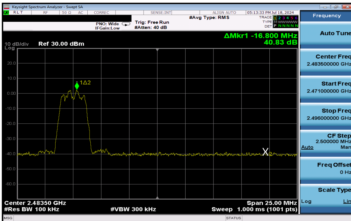
Plot 7-82. Band Edge Plot Antenna WF2 (Bluetooth (HDR4), iPA – Ch. 73)
