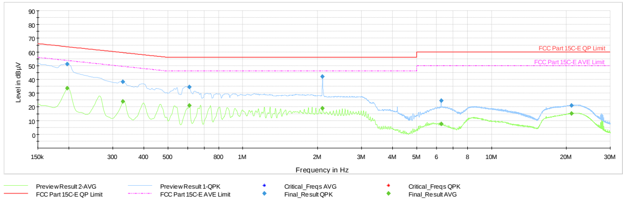
Plot 7-134. AC Line Conducted Plot with Bluetooth HDR Tx BF (N, 4Mbps ePA - Ch.38 with host PC via USB-C cable with wire charger)
