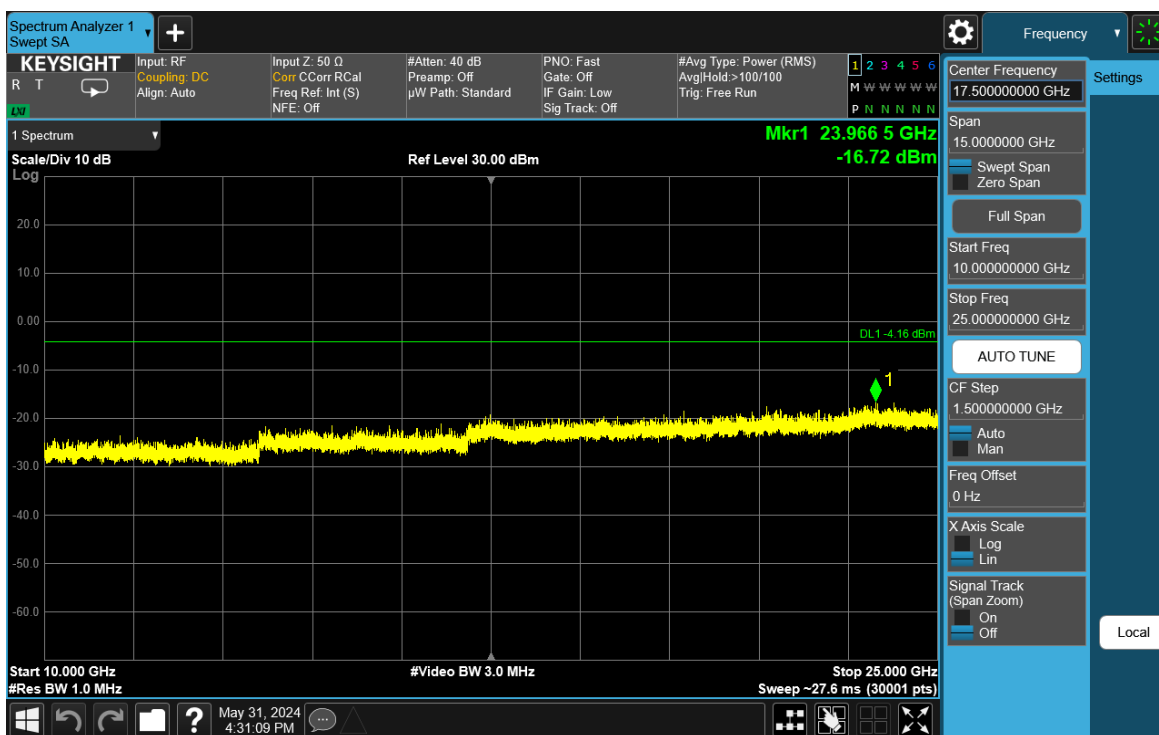
Plot 7-86. Conducted Spurious Plot Antenna WF8 (Bluetooth (HDR4), 4 Mbps, ePA – Ch. 1)
