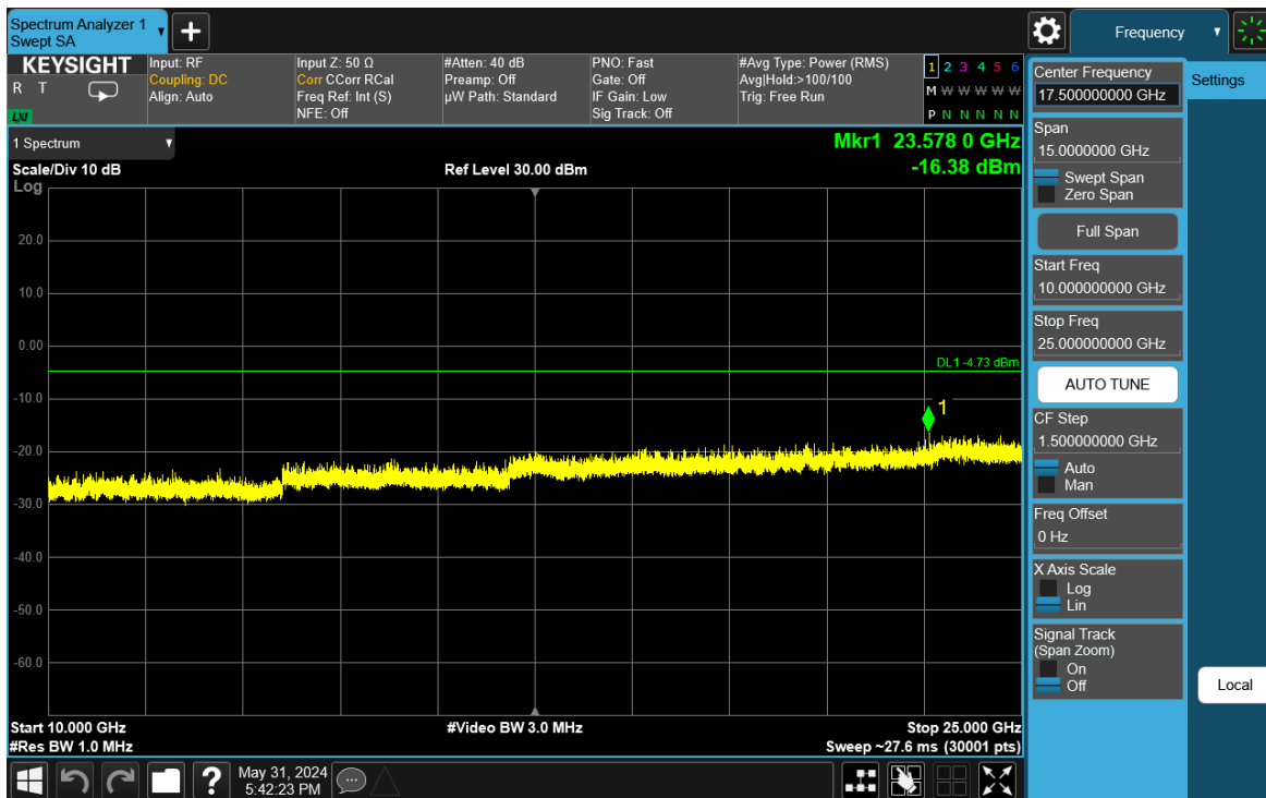
Plot 7-96. Conducted Spurious Plot Antenna WF7 (Bluetooth (HDR4), 4 Mbps, ePA – Ch. 73)
