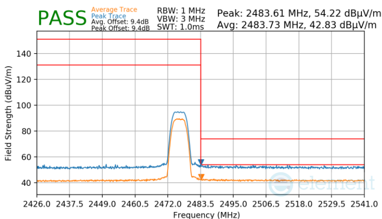
Plot 7-119. Radiated Restricted Upper Band Edge Measurement Antenna WF8
