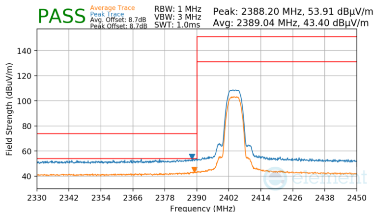
Plot 7-121. Radiated Restricted Lower Band Edge Measurement Antenna WF7
