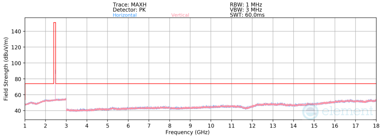
Plot 7-111. Radiated Spurious Emissions 1-18GHz Antenna WF2 (4Mbps, HDR4, iPA – Ch. 73)
