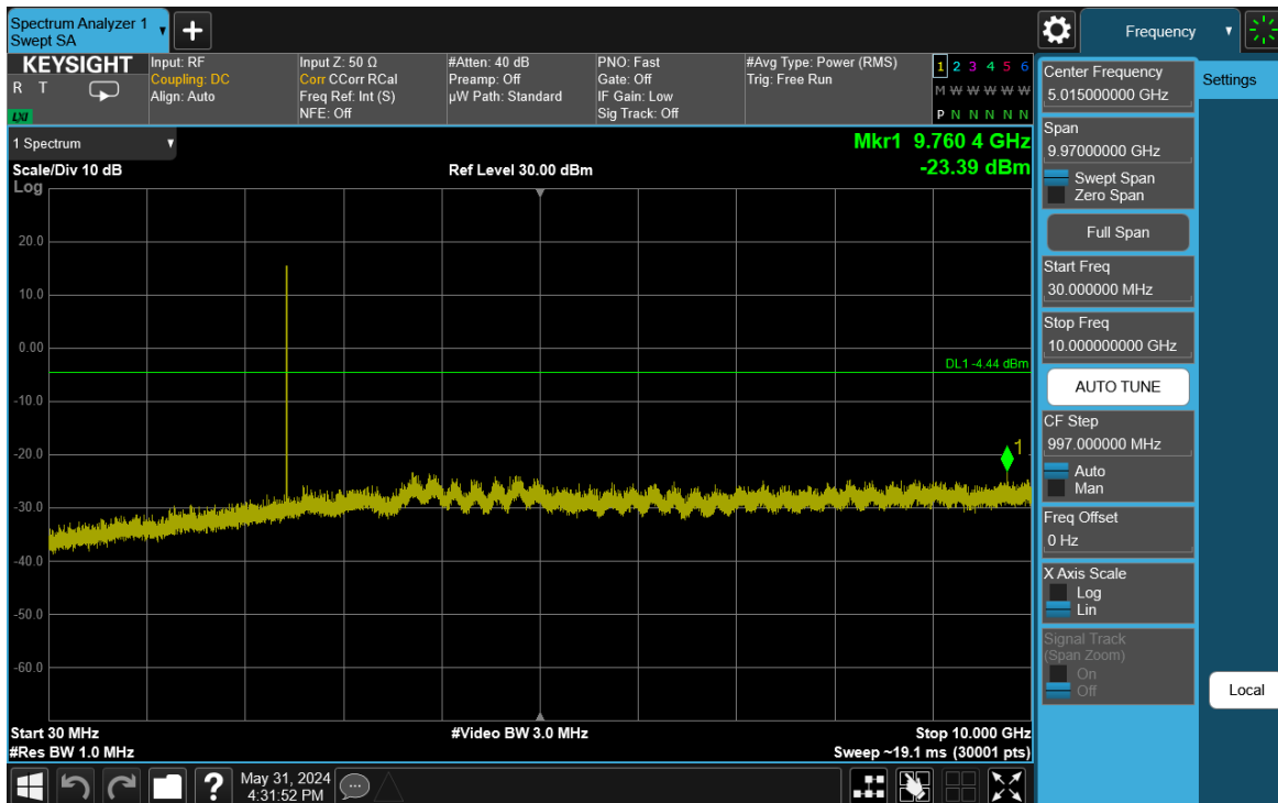
Plot 7-87. Conducted Spurious Plot Antenna WF8 (Bluetooth (HDR4), 4 Mbps, ePA – Ch. 38)
