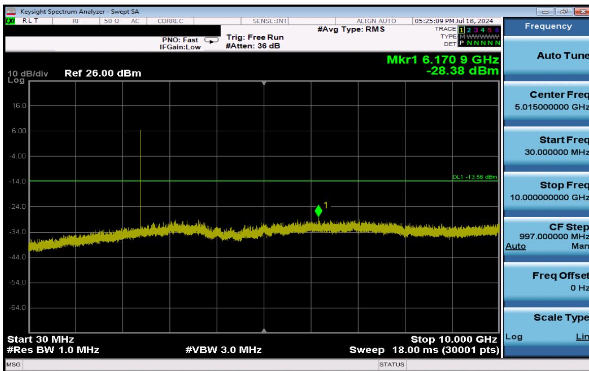
Plot 7-97. Conducted Spurious Plot Antenna WF2 (Bluetooth (HDR4), 4 Mbps, iPA – Ch. 1)
