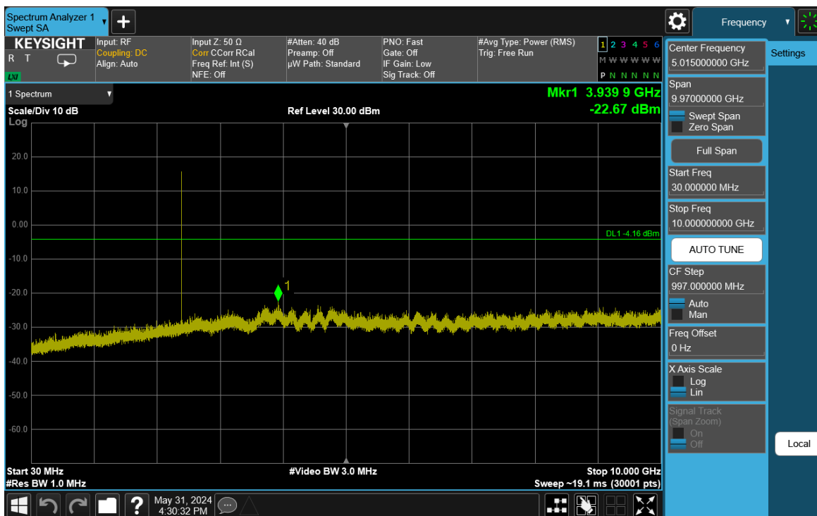
Plot 7-85. Conducted Spurious Plot Antenna WF8 (Bluetooth (HDR4), 4 Mbps, ePA – Ch. 1)
