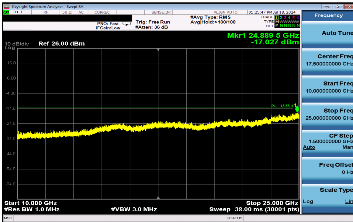
Plot 7-98. Conducted Spurious Plot Antenna WF2 (Bluetooth (HDR4), 4 Mbps, iPA – Ch. 1)
