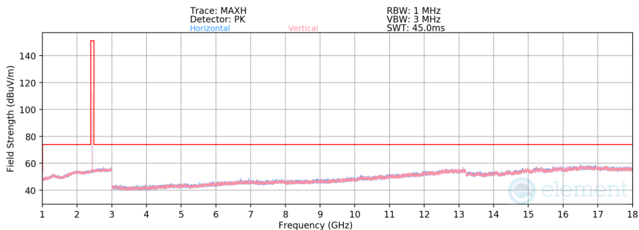
Plot 7-113. Radiated Spurious Emissions 1-18GHz TxBF (4Mbps, HDR4, ePA – Ch. 38)
