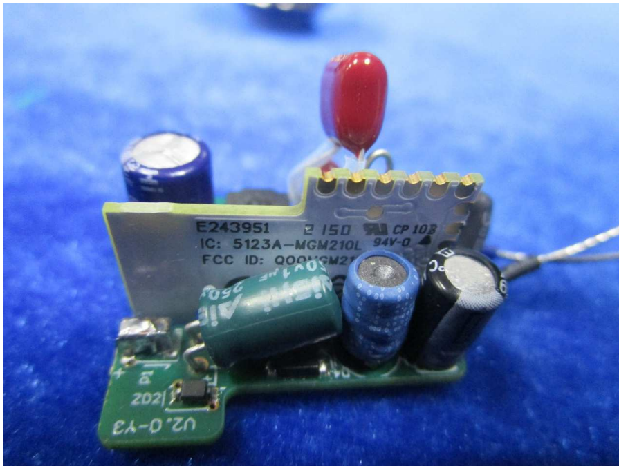
PCB
