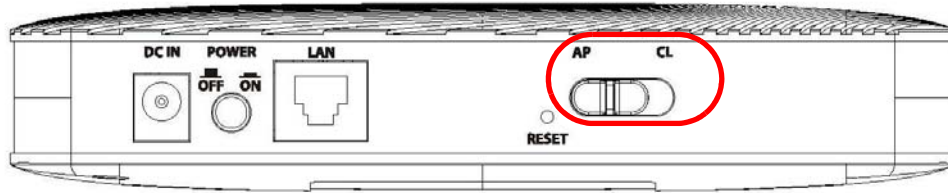
Figure 7 Side Panel
