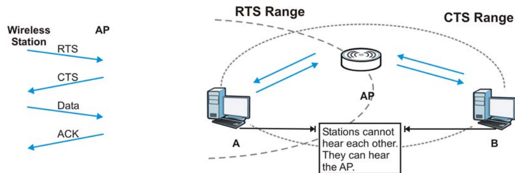
Figure 60 RTS/CTS
