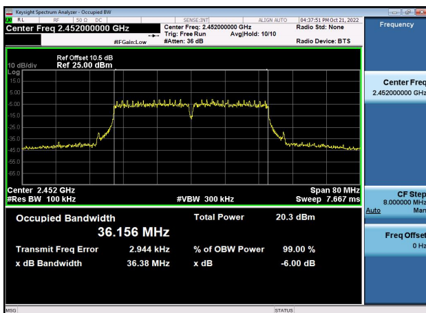
6dB Bandwidth-802.11n(HT40),2452MHz ,Ant0
