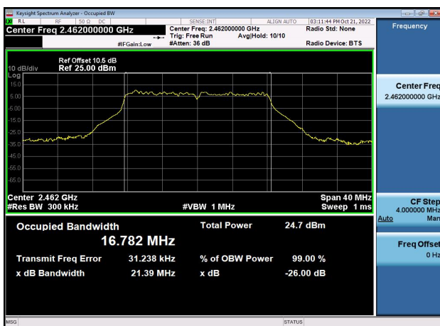
99% Bandwidth-802.11g,2462MHz,Ant0
