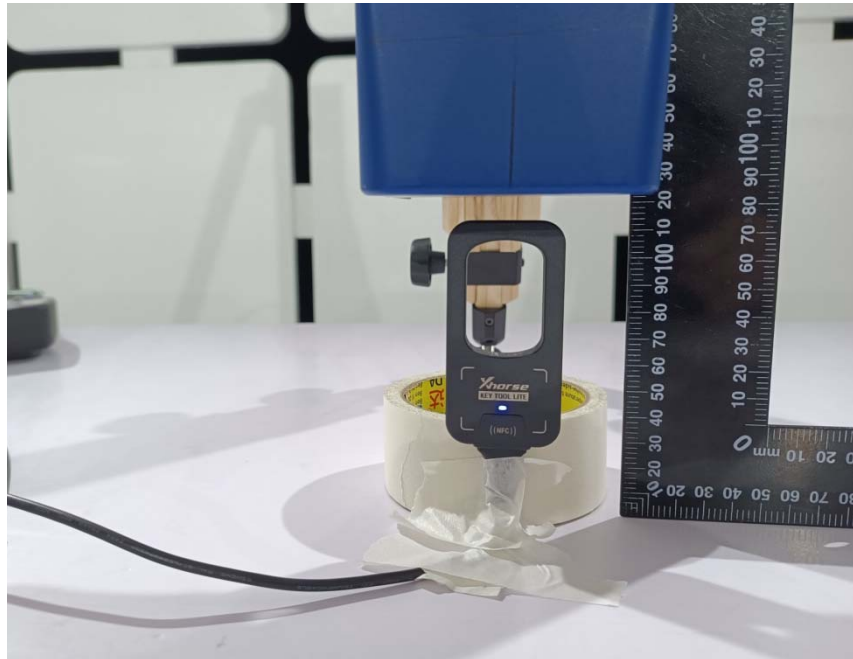
Top Side (Test distance: 10 mm)
