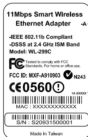
BACK LABEL
