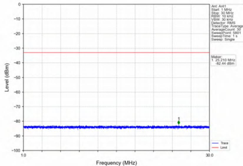
n7_15kHz_SISO_NTNV_25MHz_DFT-s-OFDM PI/2 BPSK_2512.5MHz_Inner_1RB_Left
