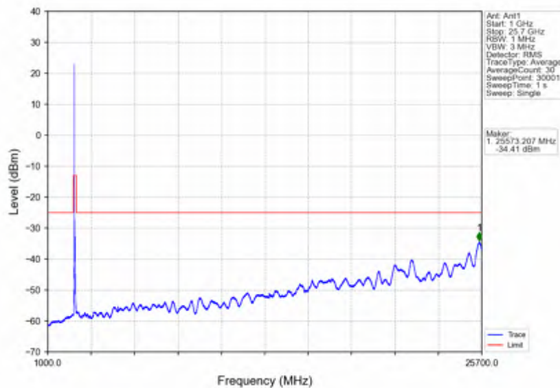
n7_15kHz_SISO_NTNV_50MHz_DFT-s-OFDM PI/2 BPSK_2535MHz_Edge_1RB_Left
