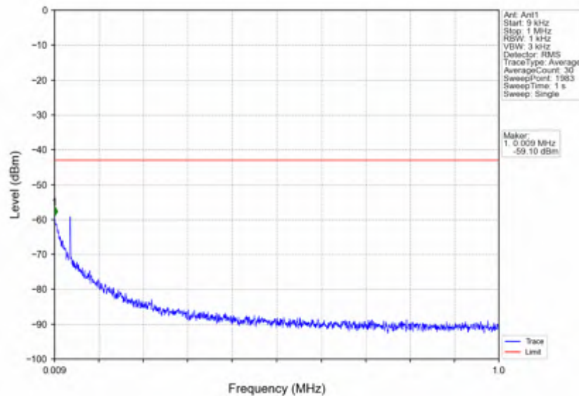
n7_15kHz_SISO_NTNV_40MHz_CP-OFDM_QPSK_2535MHz_Edge_1RB_Left
