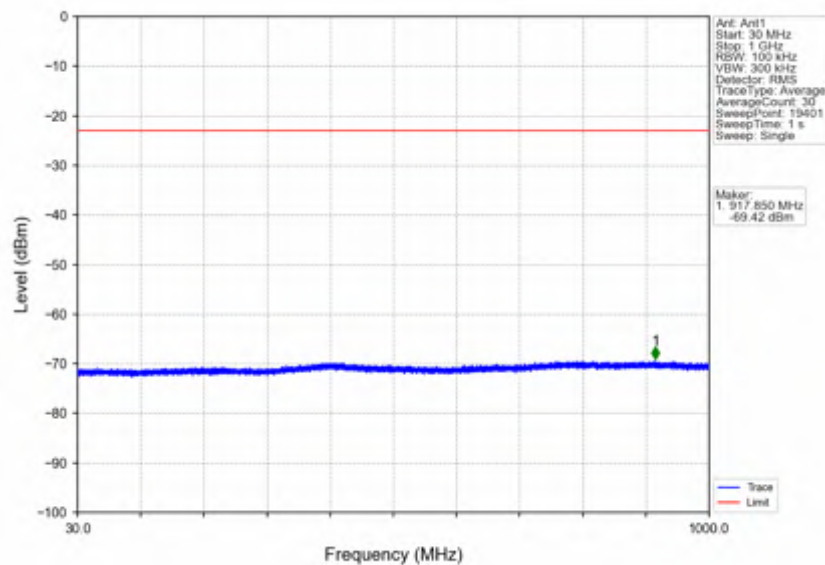
n7_15kHz_SISO_NTNV_40MHz_DFT-s-OFDM_QPSK_2550MHz_Edge_1RB_Right
