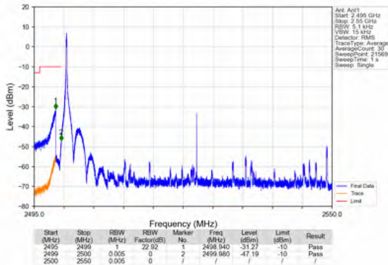
n7_15kHz_SISO_NTNV_50MHz_DFT-s-OFDM_QPSK_2525MHz_Inner_1RB_Left
