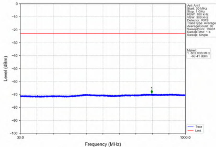
n7_15kHz_SISO_NTNV_40MHz_DFT-s-OFDM PI/2 BPSK_2550MHz_Outer_Full
