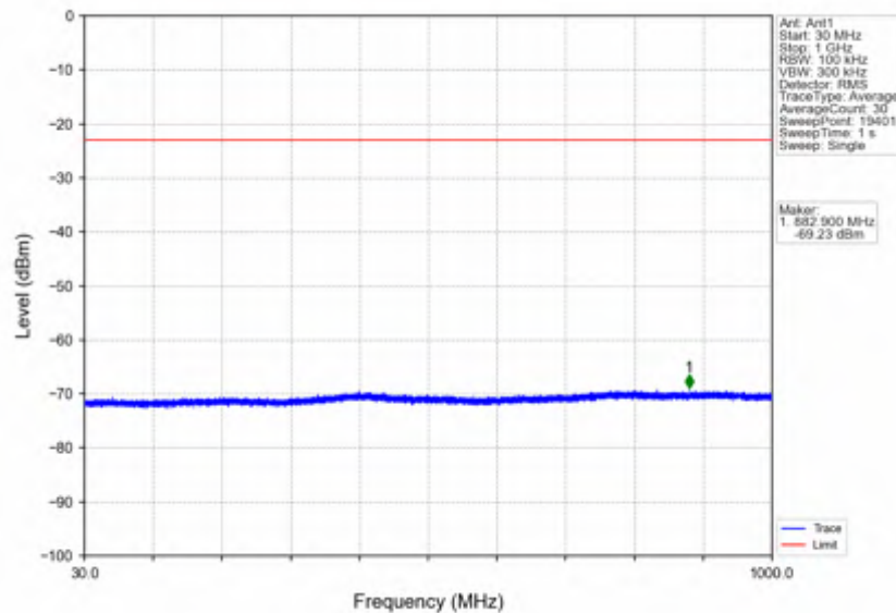
n7_15kHz_SISO_NTNV_50MHz_DFT-s-OFDM PI/2 BPSK_2545MHz_Edge_1RB_Right
