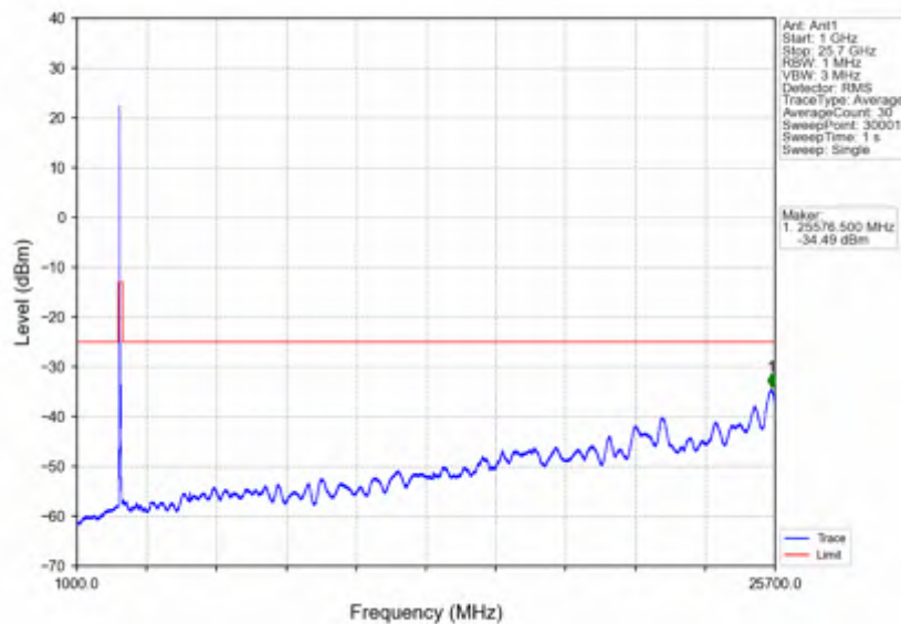
n7_15kHz_SISO_NTNV_40MHz_DFT-s-OFDM PI/2 BPSK_2535MHz_Edge_1RB_Left
