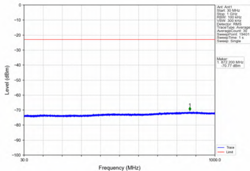
n7 15kHz SISO NTN 25MHz DFT-s-OFDM QPSK 2512.5MHz Inner 1RB Left
