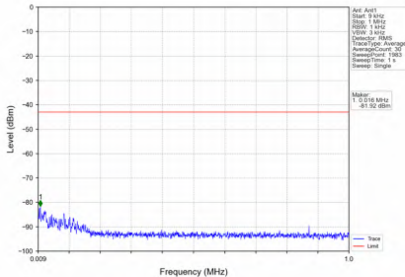
n7_15kHz_SISO_NTNV_25MHz_CP-OFDM QPSK_2535MHz_Edge_1RB_Left
