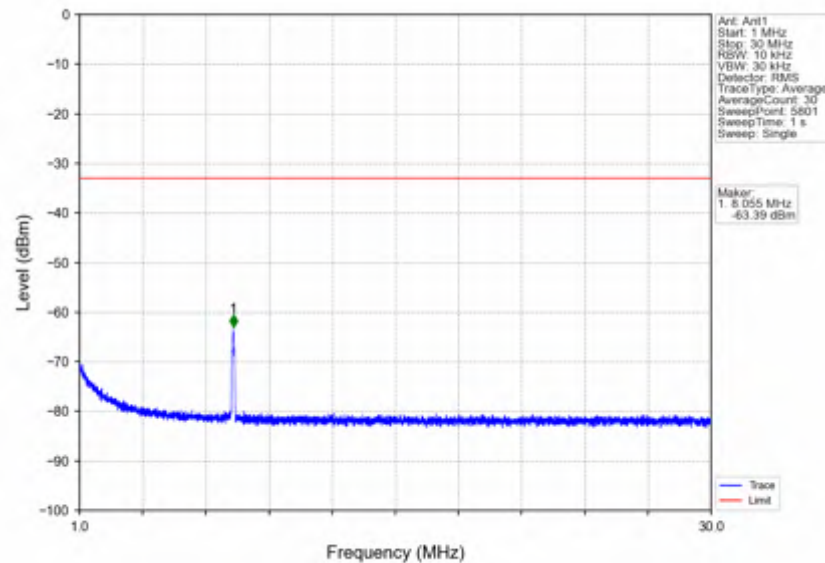
n7_15kHz_SISO_NTNV_30MHz_CP-OFDM_QPSK_2555MHz_Edge_1RB_Right
