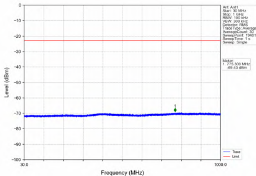
n7_15kHz_SISO_NTNV_40MHz_CP-OFDM_QPSK_2520MHz_Outer_Full
