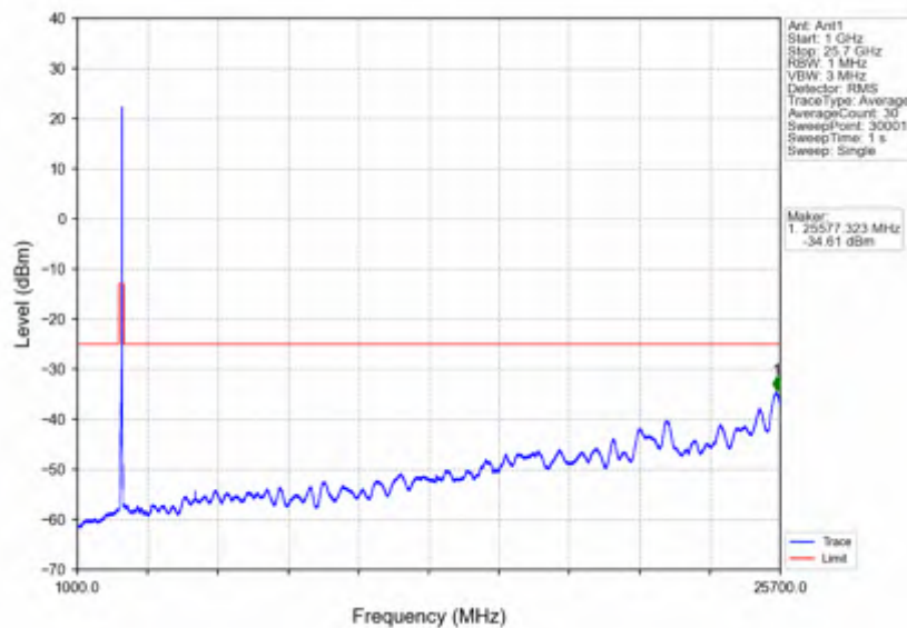
n7_15kHz_SISO_NTNV_50MHz_DFT-s-OFDM PI/2 BPSK_2545MHz_Outer_Full
