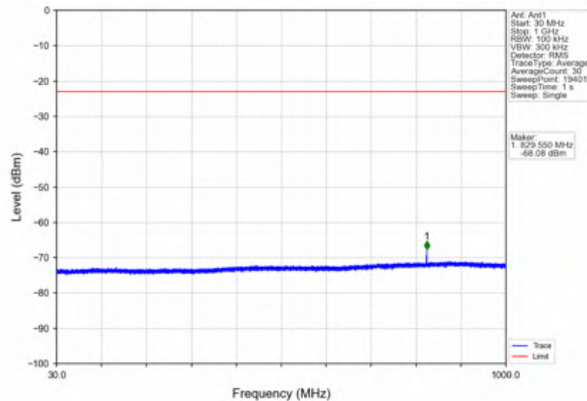
n7_15kHz_SISO_NTNV_25MHz_DFT-s-OFDM PI/2 BPSK_2512.5MHz_Edge_1RB_Left
