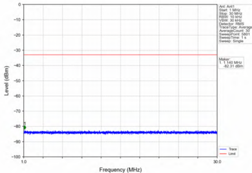
n7_15kHz_SISO_NTNV_30MHz_DFT-s-OFDM PI/2 BPSK_2515MHz_Edge_1RB_Left
