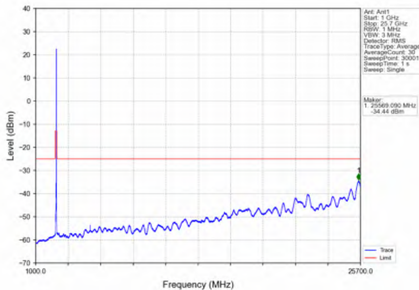
n7_15kHz_SISO_NTNV_30MHz_DFT-s-OFDM QPSK_2515MHz_Edge_1RB_Left
