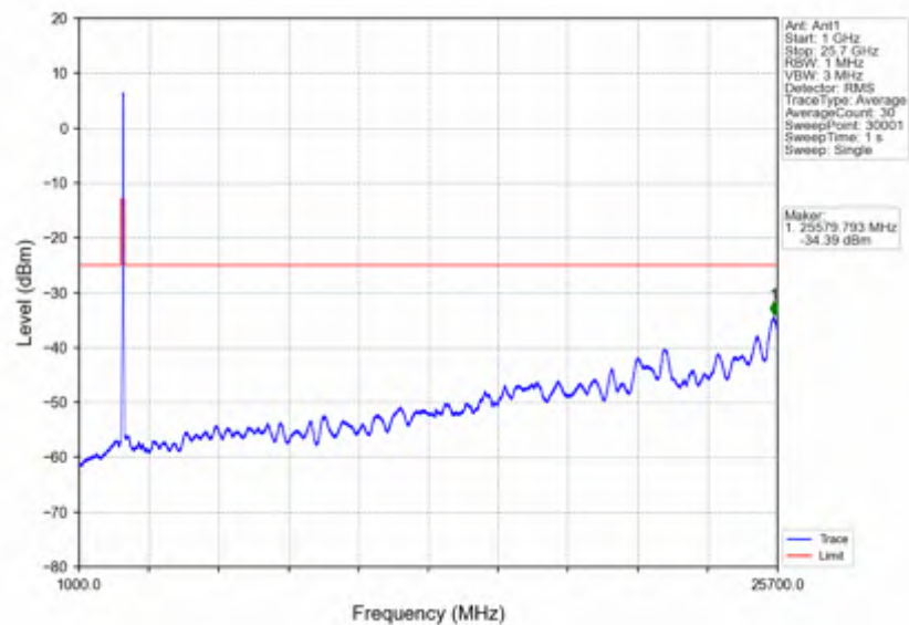
n7_15kHz_SISO_NTNV_30MHz_CP-OFDM_QPSK_2555MHz_Outer_Full
