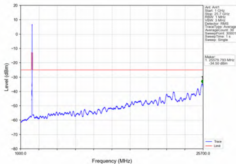
n7 15kHz SISO NTNV 50MHz DFT-s-OFDM PI/2 BPSK 2545MHz Outer Full
