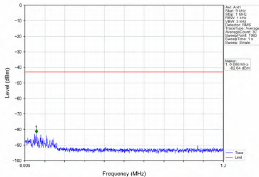
n7_15kHz_SISO_NTNV_30MHz_DFT-s-OFDM QPSK_2515MHz_Edge_1RB_Left
