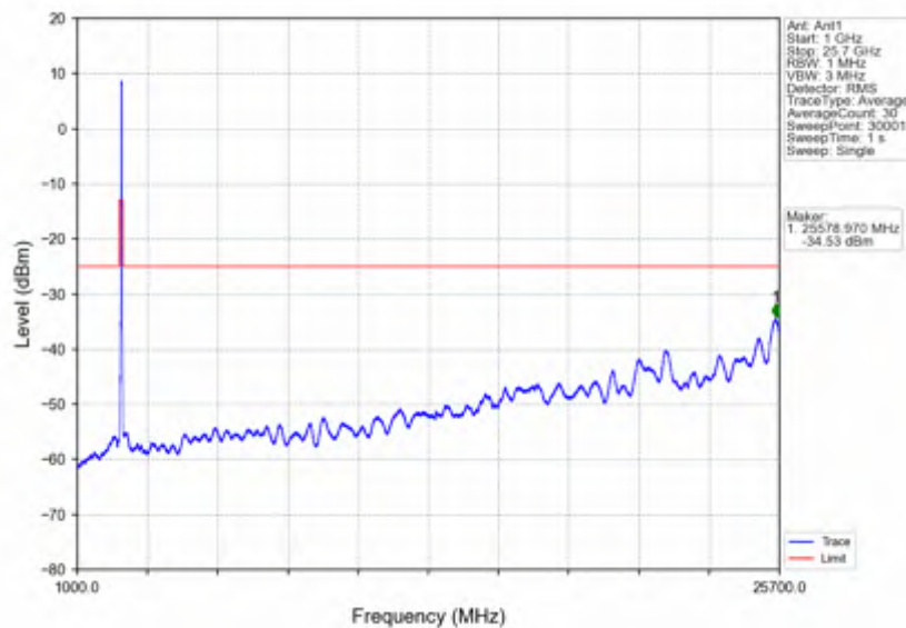
n7_15kHz_SISO_NTNV_30MHz_DFT-s-OFDM QPSK_2555MHz_Inner_1RB_Right
