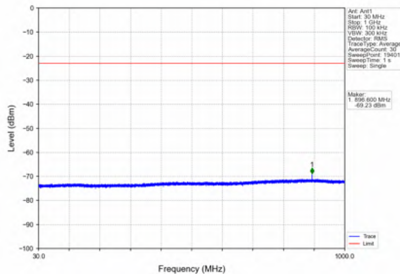
n7_15kHz_SISO_NTNV_25MHz_CP-OFDM QPSK_2557.5MHz_Inner_1RB_Right
