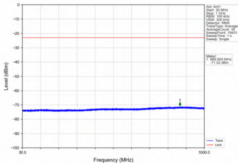
n7_15kHz_SISO_NTNV_25MHz_CP-OFDM QPSK_2535MHz_Edge_1RB_Left
