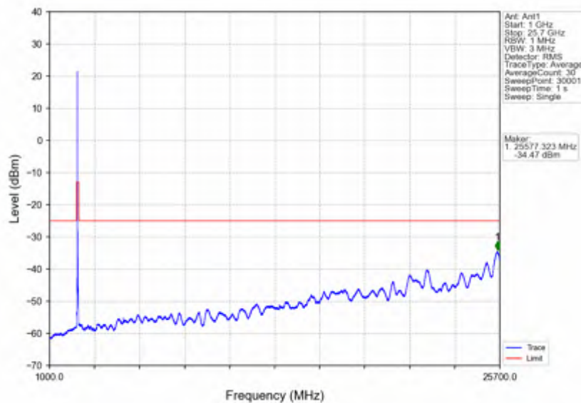
n7_15kHz_SISO_NTNV_30MHz_DFT-s-OFDM QPSK_2555MHz_Edge_1RB_Right
