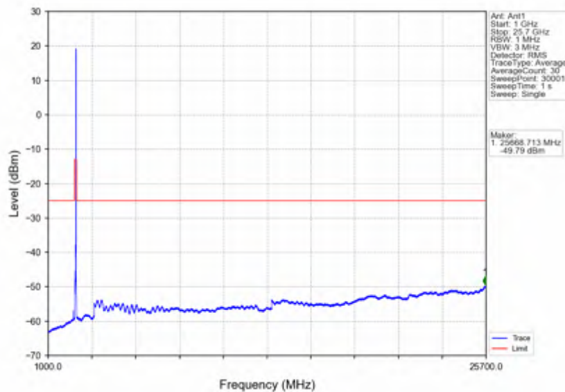
n7_15kHz_SISO_NTNV_25MHz_CP-OFDM QPSK_2557.5MHz_Outer_Full
