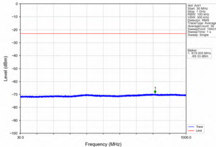
n7_15kHz_SISO_NTNV_50MHz_DFT-s-OFDM PI/2 BPSK_2525MHz_Edge_1RB_Left
