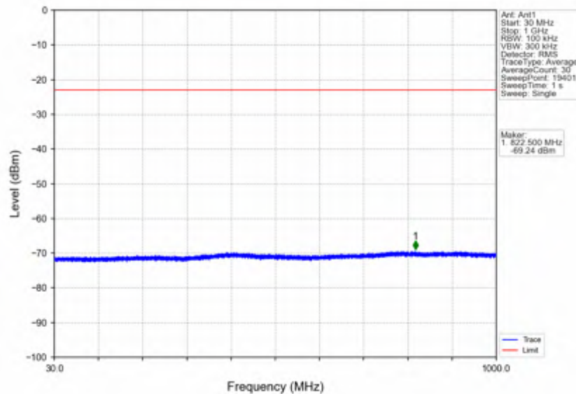
n7_15kHz_SISO_NTNV_40MHz_DFT-s-OFDM PI/2 BPSK_2520MHz_Edge_1RB_Left
