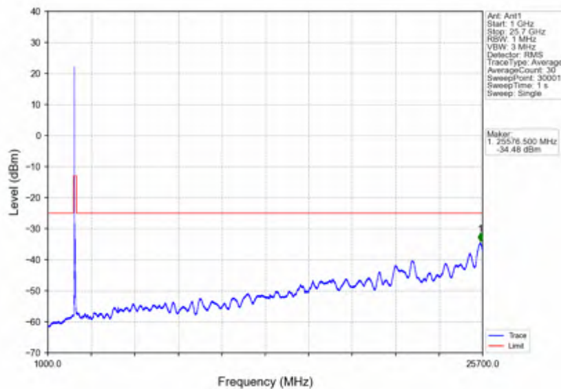
n7_15kHz_SISO_NTNV_50MHz_DFT-s-OFDM PI/2 BPSK 2525MHz_Outer_Full
