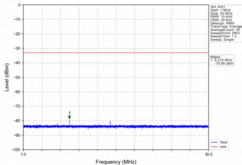
n7_15kHz_SISO_NTNV_25MHz_DFT-s-OFDM QPSK_2512.5MHz_Outer_Full
