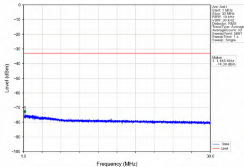
n7_15kHz_SISO_NTNV_25MHz_DFT-s-OFDM QPSK_2557.5MHz_Outer_Full
