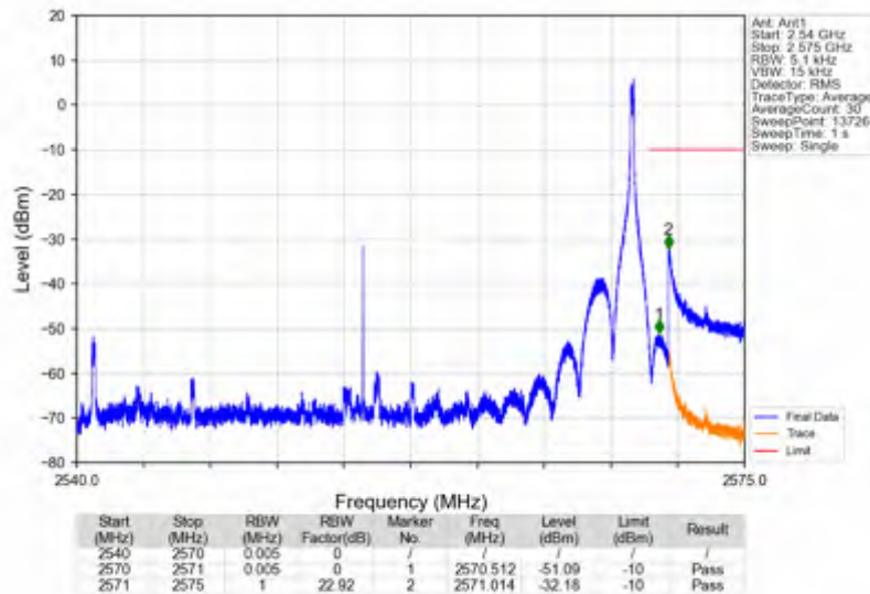
n7_15kHz_SISO_NTNV_30MHz_DFT-s-OFDM QPSK_2555MHz_Inner_1RB_Right
