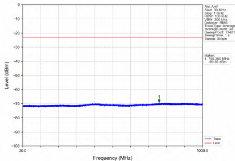
n7_15kHz_SISO_NTNV_40MHz_DFT-s-OFDM PI/2 BPSK_2550MHz_Edge_1RB_Right
