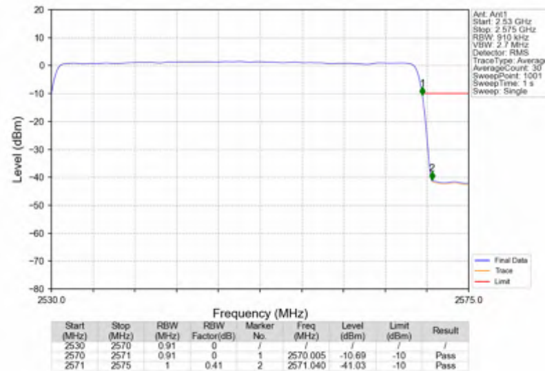
n7_15kHz_SISO_NTNV_40MHz_DFT-s-OFDM_QPSK_2550MHz_Outer_Full
