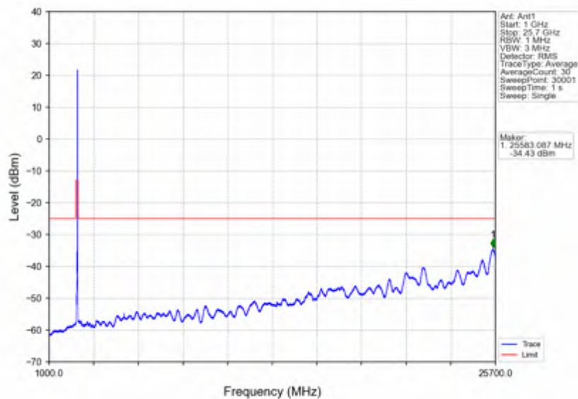
n7_15kHz_SISO_NTNV_30MHz_DFT-s-OFDM QPSK_2555MHz_Edge_1RB_Right
