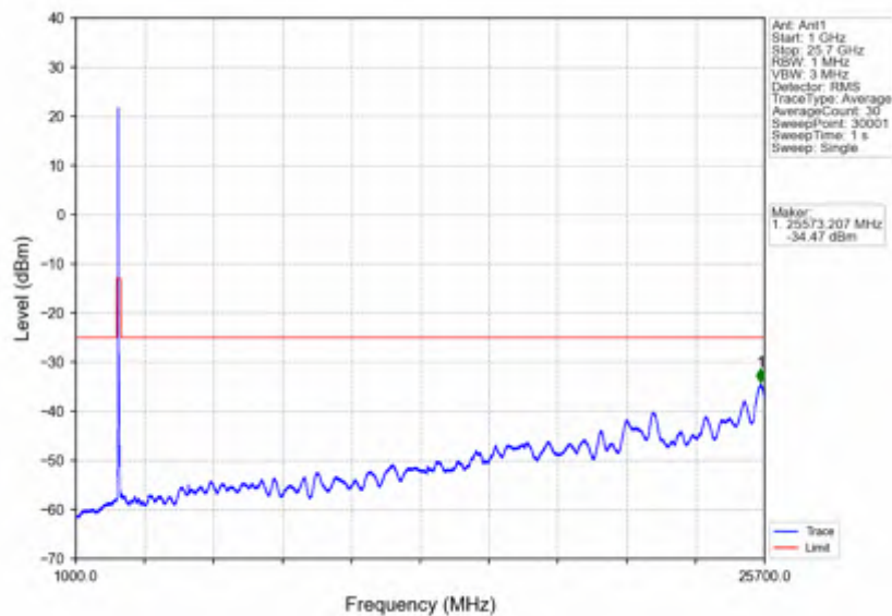
n7_15kHz_SISO_NTNV_40MHz_DFT-s-OFDM_PI/2_BPSK_2535MHz_Edge_1RB_Left
