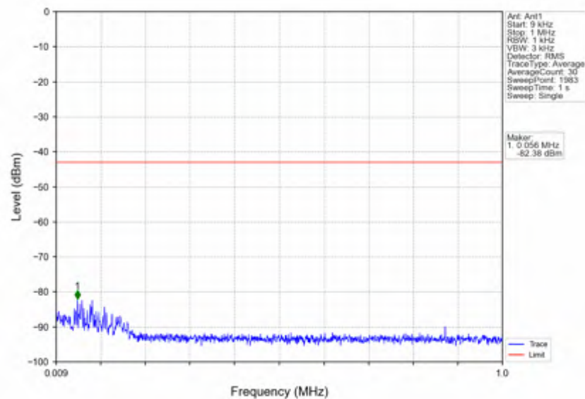
n7_15kHz_SISO_NTNV_25MHz_DFT-s-OFDM QPSK_2512.5MHz_Edge_1RB_Left
