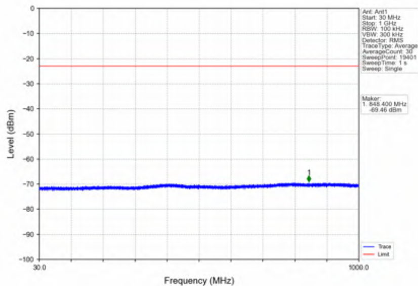
n7_15kHz_SISO_NTNV_50MHz_DFT-s-OFDM_PI/2_BPSK_2535MHz_Edge_1RB_Left
