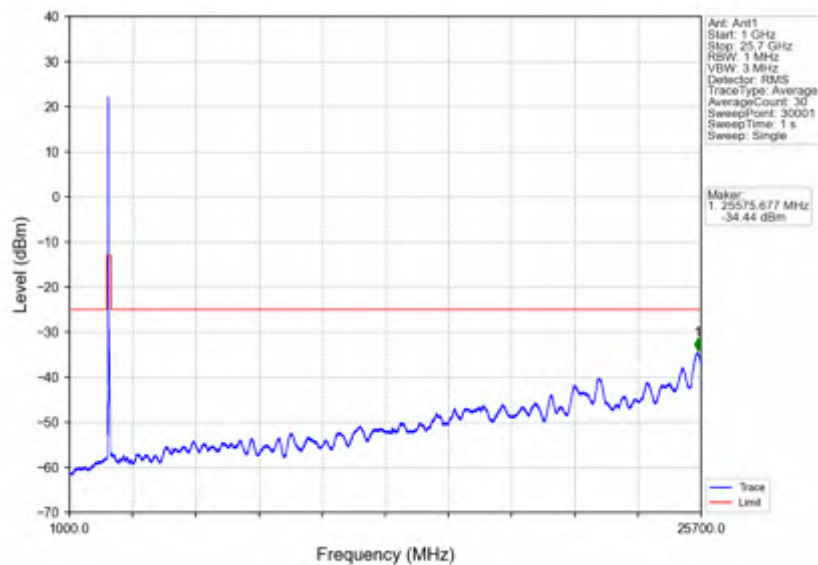
n7_15kHz_SISO_NTNV_50MHz_DFT-s-OFDM_PI/2_BPSK_2535MHz_Edge_1RB_Left
