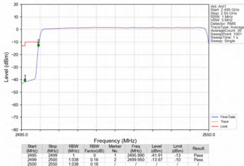
n7_15kHz_SISO_NTNV_50MHz_DFT-s-OFDM PI/2 BPSK 2525MHz_Outer_Full
