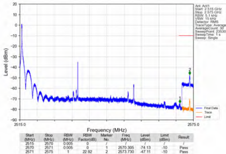
n7_15kHz_SISO_NTNV_40MHz_CP-OFDM QPSK_2535MHz_Edge_1RB_Left
