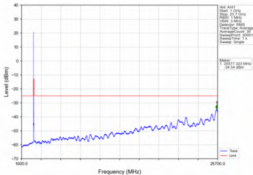
n7_15kHz_SISO_NTNV_30MHz_CP-OFDM QPSK_2535MHz_Edge_1RB_Left
