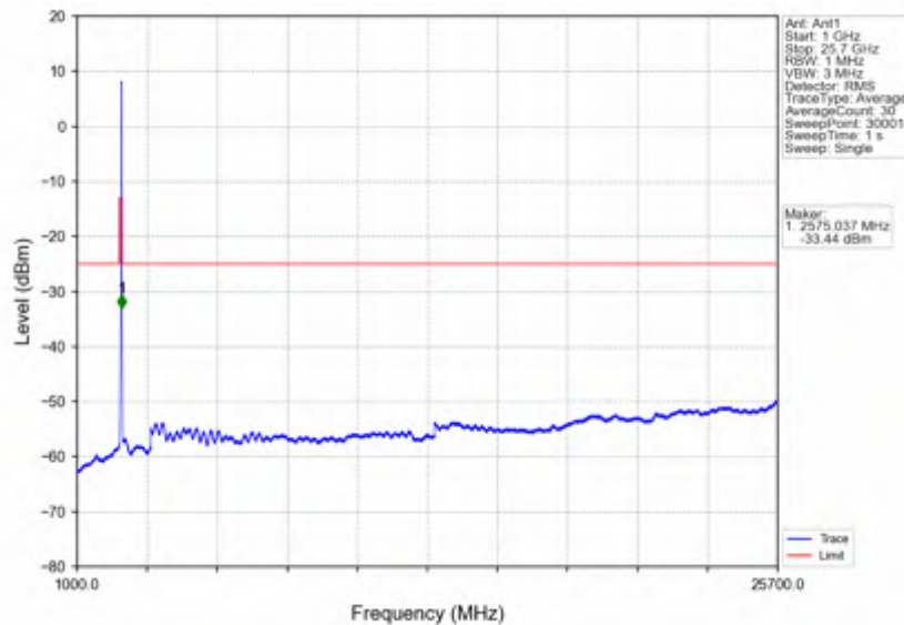
n7_15kHz_SISO_NTNV_20MHz_CP-OFDM_QPSK_2560MHz_Outer_Full
