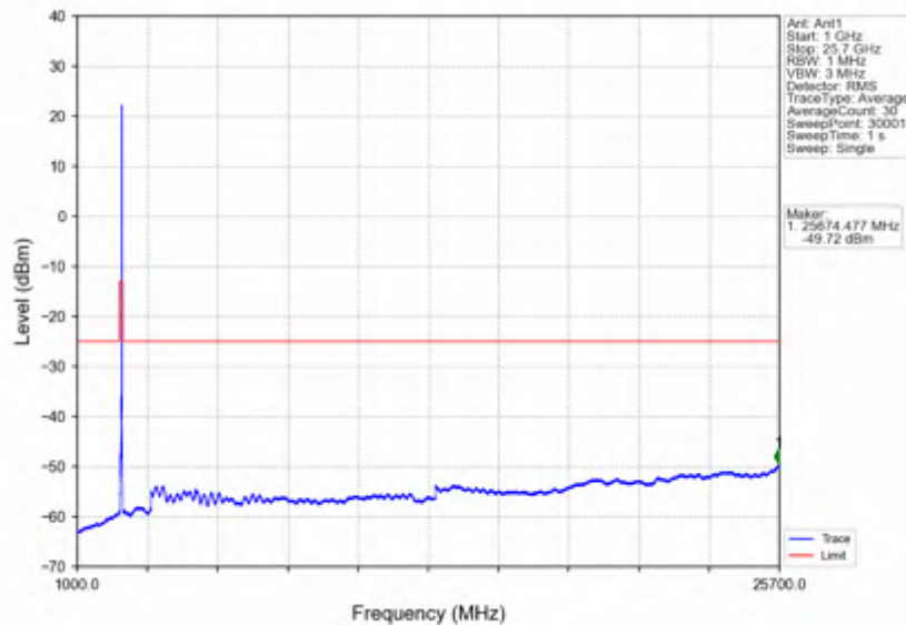
n7_15kHz_SISO_NTNV_25MHz_DFT-s-OFDM QPSK_2557.5MHz_Inner_1RB_Right
