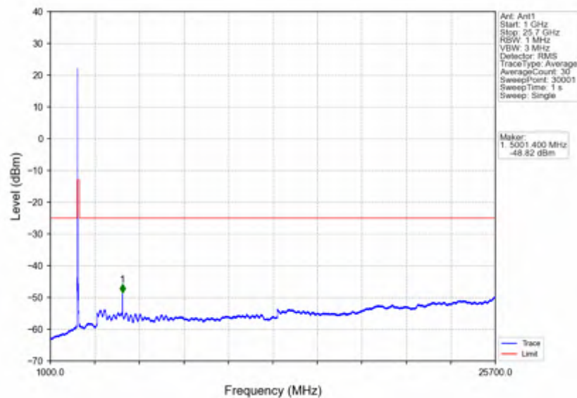
n7 15kHz SISO NTN 25MHz DFT-s-OFDM QPSK 2512.5MHz Inner 1RB Left
