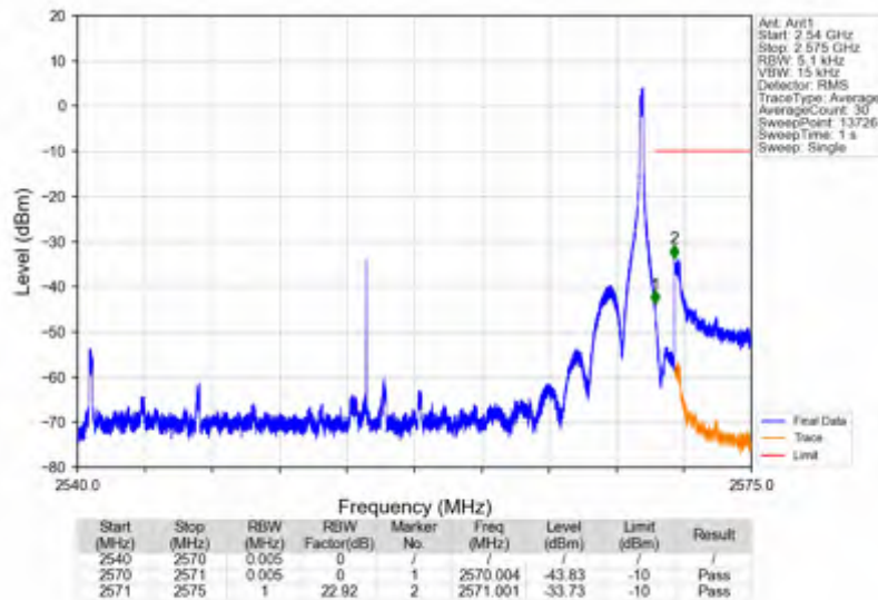
n7_15kHz_SISO_NTNV_30MHz_DFT-s-OFDM QPSK_2555MHz_Edge_1RB_Right
