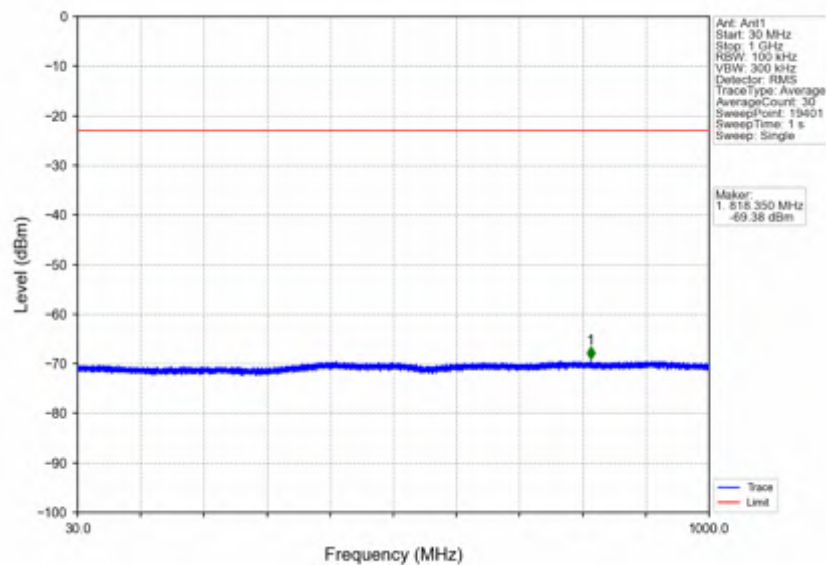
n7_15kHz_SISO_NTNV_30MHz_DFT-s-OFDM_QPSK_2555MHz_Outer_Full
