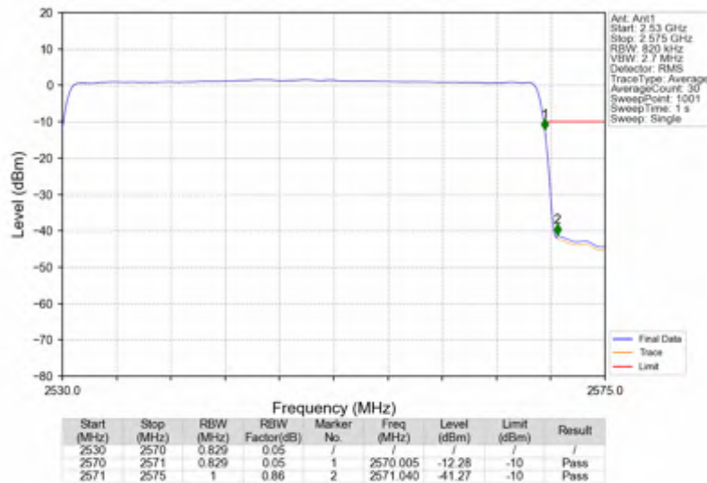
n7_15kHz_SISO_NTNV_40MHz_DFT-s-OFDM PI/2 BPSK_2550MHz_Outer_Full
