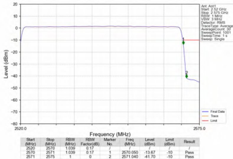
n7_15kHz_SISO_NTNV_50MHz_DFT-s-OFDM PI/2 BPSK_2545MHz_Outer_Full
