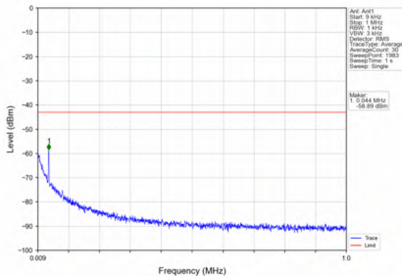
n7_15kHz_SISO_NTNV_50MHz_DFT-s-OFDM_QPSK_2525MHz_Outer_Full
