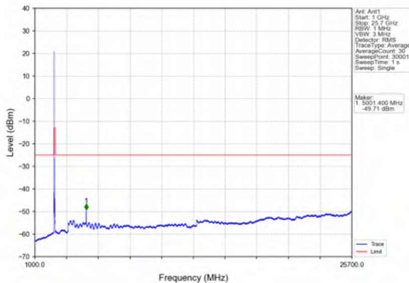
n7_15kHz_SISO_NTNV_25MHz_DFT-s-OFDM PI/2 BPSK_2512.5MHz_Outer_Full
