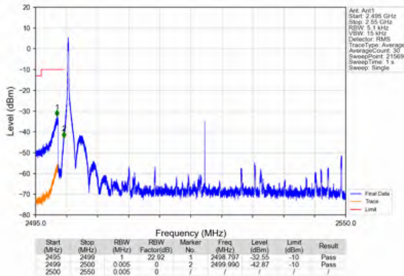
n7_15kHz_SISO_NTNV_50MHz_DFT-s-OFDM QPSK_2525MHz_Edge_1RB_Left
