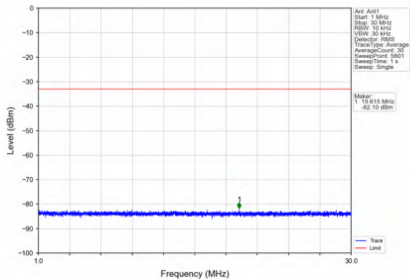
n7_15kHz_SISO_NTNV_25MHz_CP-OFDM QPSK_2512.5MHz_Outer_Full
