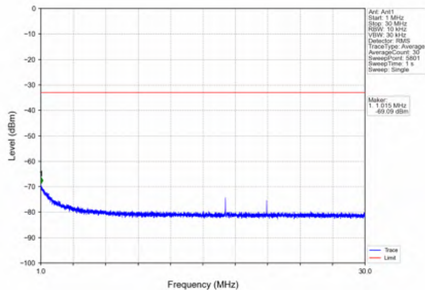
n7_15kHz_SISO_NTNV_40MHz_DFT-s-OFDM_QPSK_2550MHz_Outer_Full
