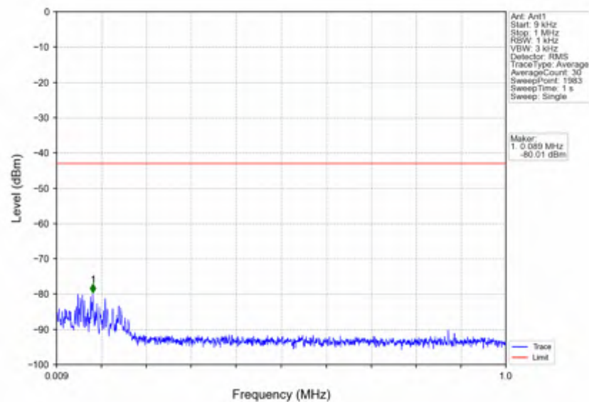
n7_15kHz_SISO_NTNV_25MHz_DFT-s-OFDM_QPSK_2512.5MHz_Inner_1RB_Left
