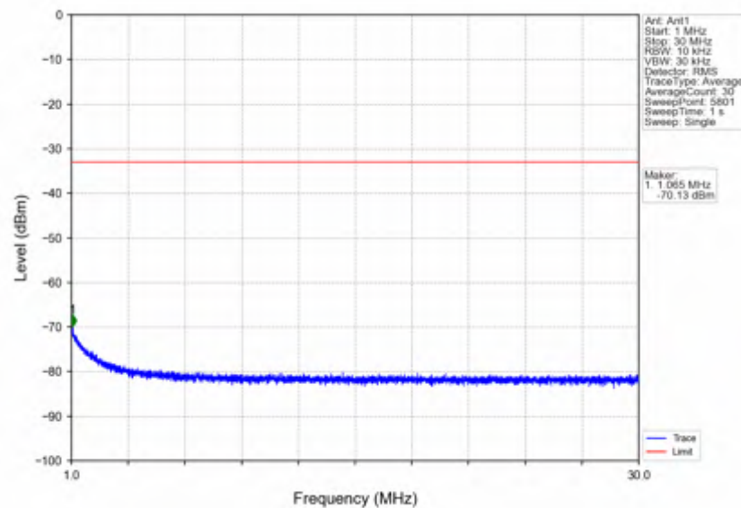
n7_15kHz_SISO_NTNV_50MHz_DFT-s-OFDM_QPSK_2525MHz_Edge_1RB_Left
