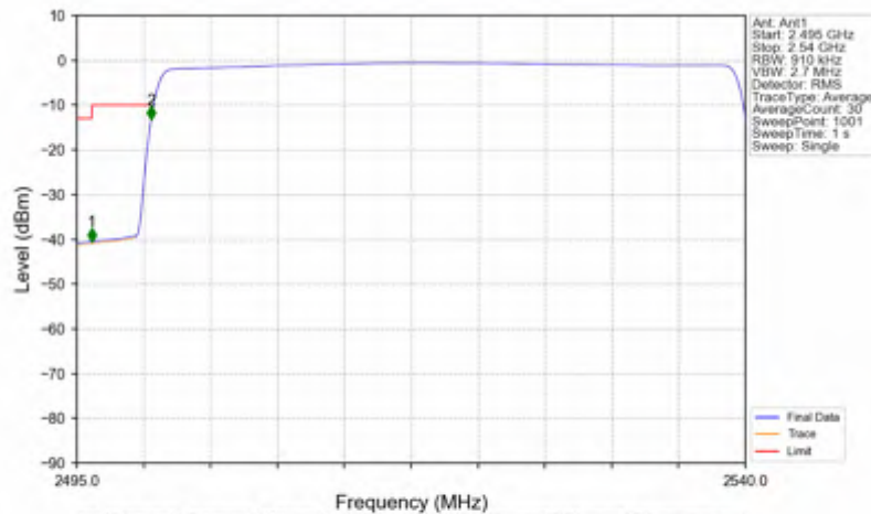
n7_15kHz_SISO_NTNV_40MHz_CP-OFDM_QPSK_2520MHz_Outer_Full
