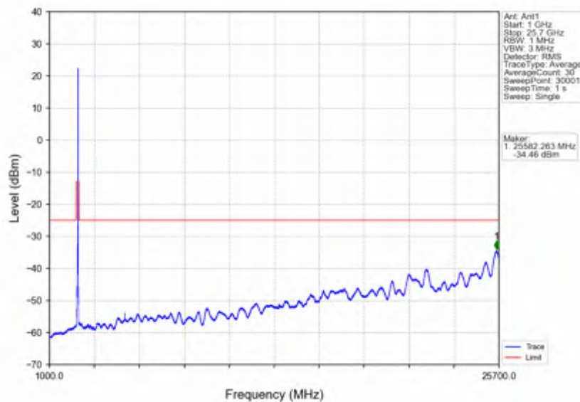
n7_15kHz_SISO_NTNV_40MHz_DFT-s-OFDM_QPSK_2550MHz_Inner_1RB_Right
