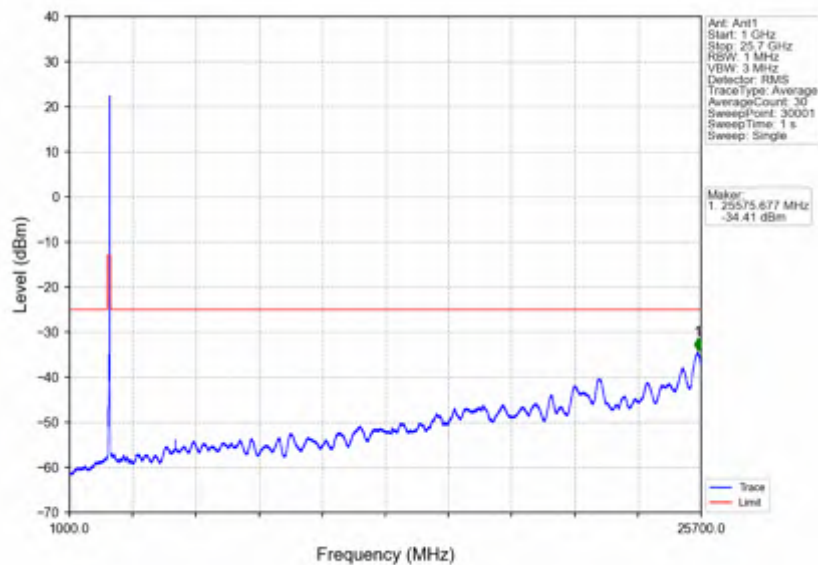
n7_15kHz_SISO_NTNV_30MHz_DFT-s-OFDM_QPSK_2555MHz_Inner_1RB_Right
