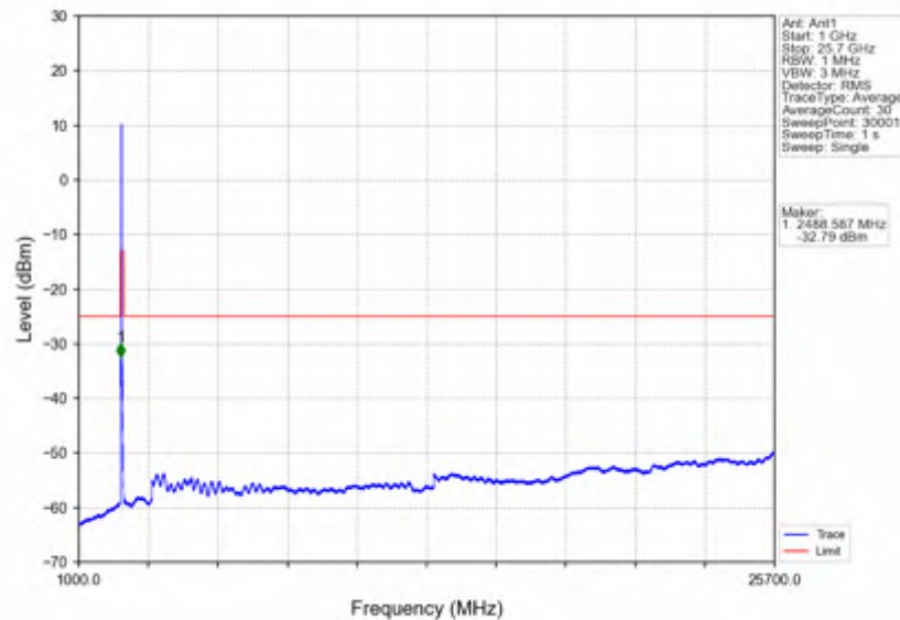
n7_15kHz_SISO_NTNV_25MHz_DFT-s-OFDM_PI/2_BPSK_2512.5MHz_Outer_Full
