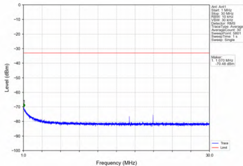
n7_15kHz_SISO_NTNV_40MHz_DFT-s-OFDM_QPSK_2520MHz_Outer_Full
