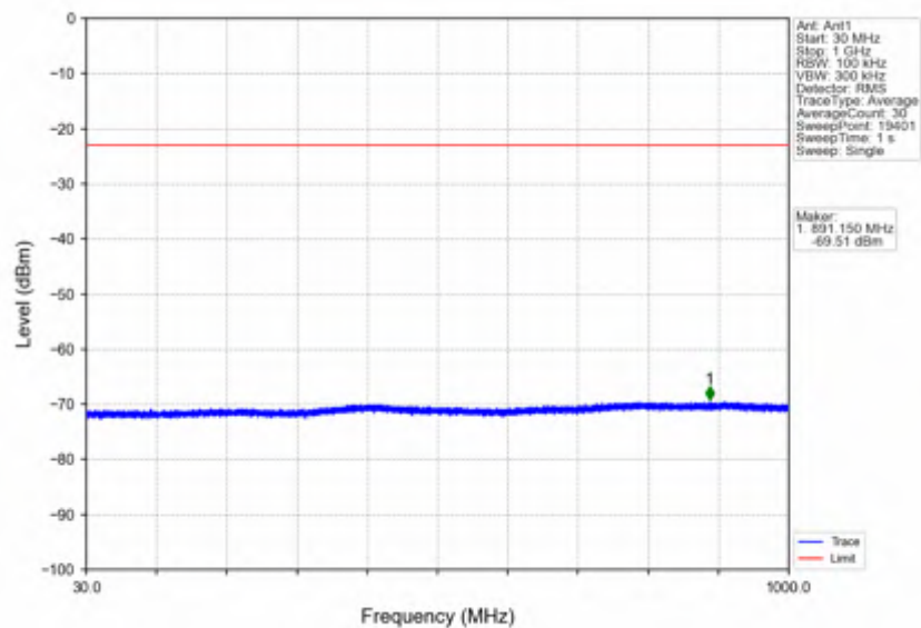
n7_15kHz_SISO_NTNV_30MHz_CP-OFDM_QPSK_2515MHz_Outer_Full
