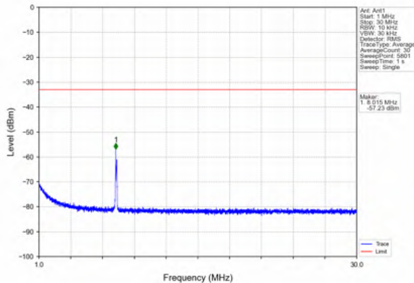
n7_15kHz_SISO_NTNV_30MHz_DFT-s-OFDM PI/2 BPSK_2555MHz_Edge_1RB_Right
