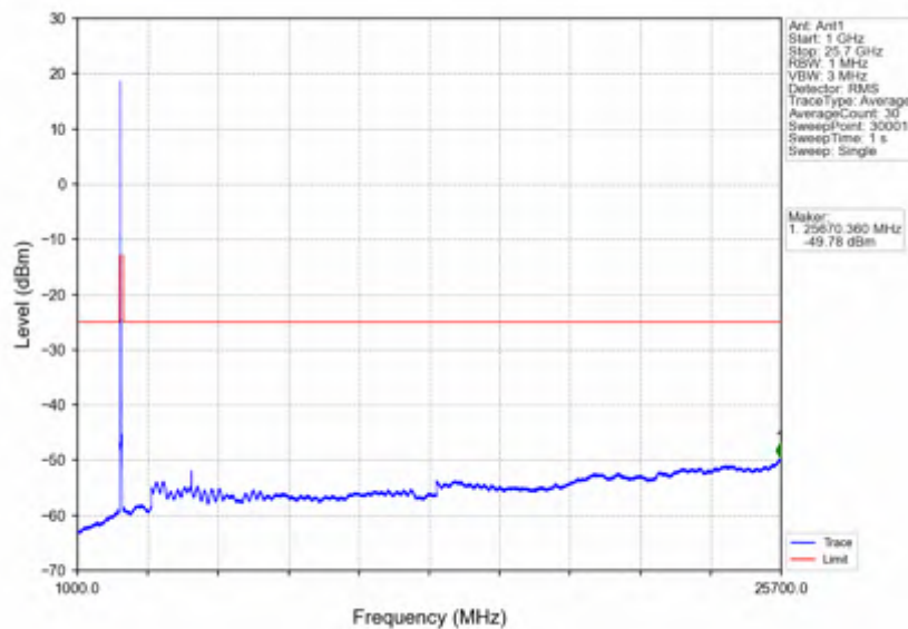
n7_15kHz_SISO_NTNV_30MHz_CP-OFDM QPSK_2515MHz_Outer_Full
