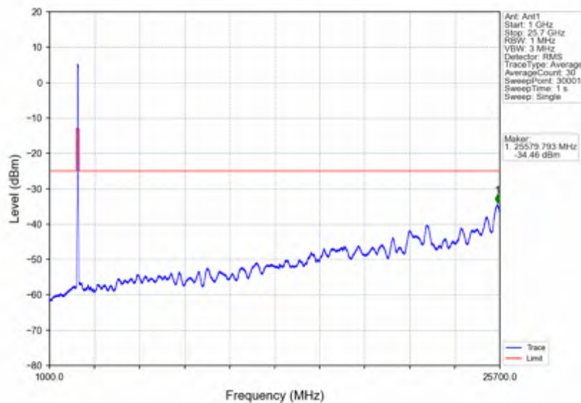
n7_15kHz_SISO_NTNV_40MHz_CP-OFDM_QPSK_2550MHz_Outer_Full
