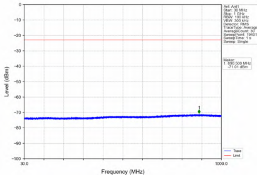
n7_15kHz_SISO_NTNV_25MHz_DFT-s-OFDM QPSK_2557.5MHz_Inner_1RB_Right
