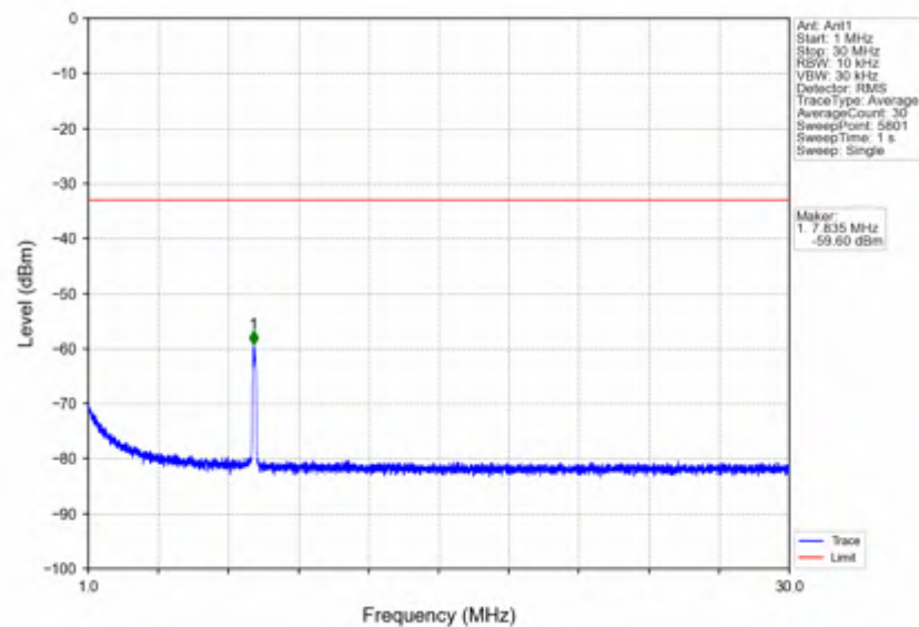
n7_15kHz_SISO_NTNV_30MHz_DFT-s-OFDM QPSK_2555MHz_Inner_1RB_Right
