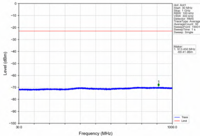
n7_15kHz_SISO_NTNV_30MHz_CP-OFDM QPSK_2535MHz_Edge_1RB_Left
