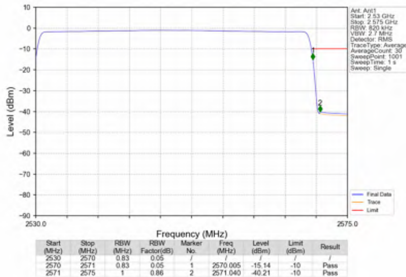
n7_15kHz_SISO_NTNV_40MHz_CP-OFDM QPSK_2550MHz_Outer_Full
