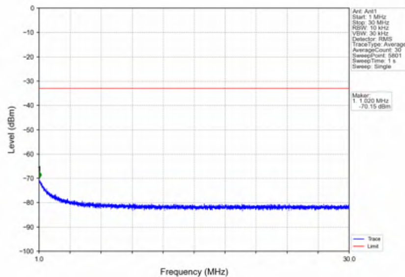
n7_15kHz_SISO_NTNV_40MHz_DFT-s-OFDM QPSK_2535MHz_Edge_1RB_Left
