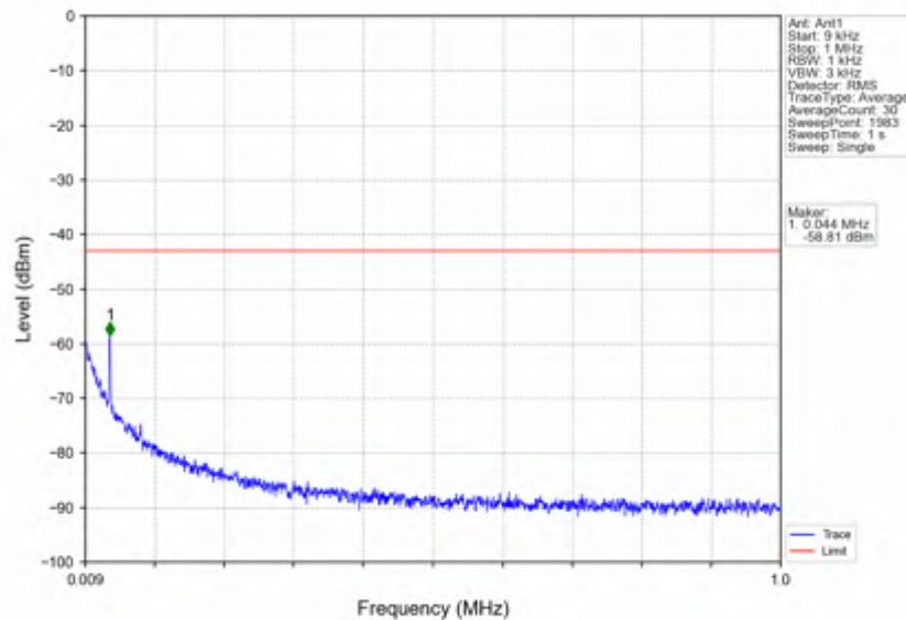
n7_15kHz_SISO_NTNV_40MHz_CP-OFDM_QPSK_2550MHz_Outer_Full
