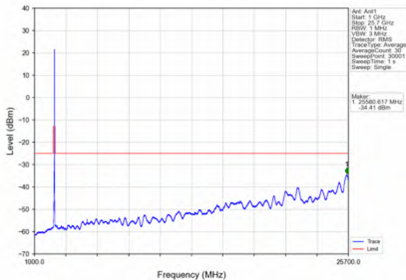
n7_15kHz_SISO_NTNV_40MHz_DFT-s-OFDM_QPSK_2550MHz_Edge_1RB_Right
