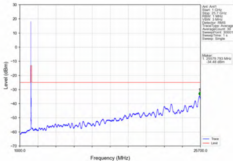
n7_15kHz_SISO_NTNV_40MHz_CP-OFDM_QPSK_2520MHz_Outer_Full
