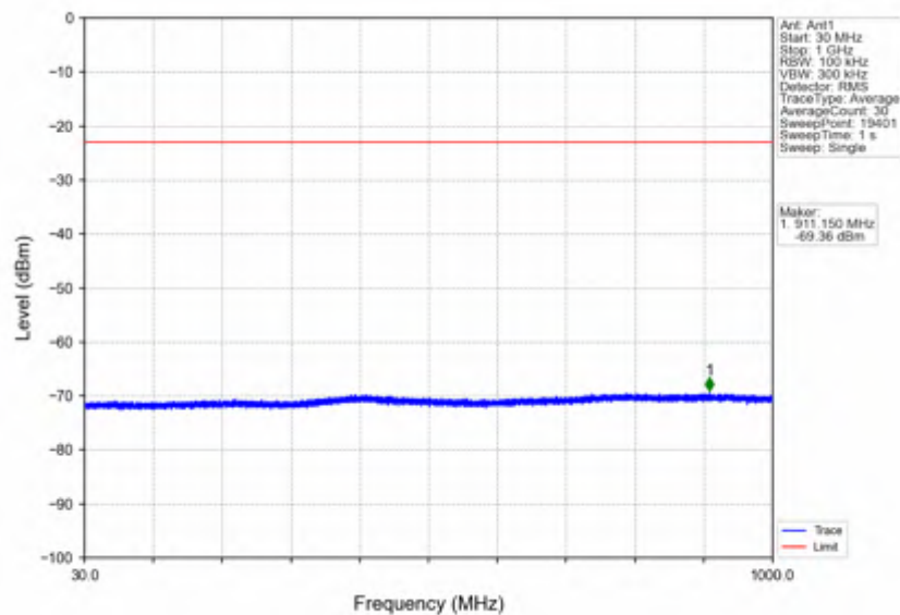
n7_15kHz_SISO_NTNV_30MHz_DFT-s-OFDM QPSK_2555MHz_Edge_1RB_Right
