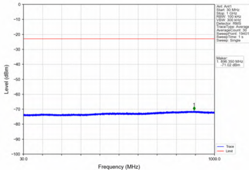
n7_15kHz_SISO_NTNV_30MHz_DFT-s-OFDM_QPSK_2515MHz_Inner_1RB_Left
