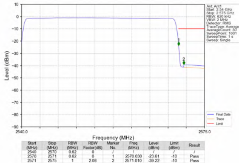
n7_15kHz_SISO_NTNV_30MHz_CP-OFDM QPSK_2555MHz_Outer_Full
