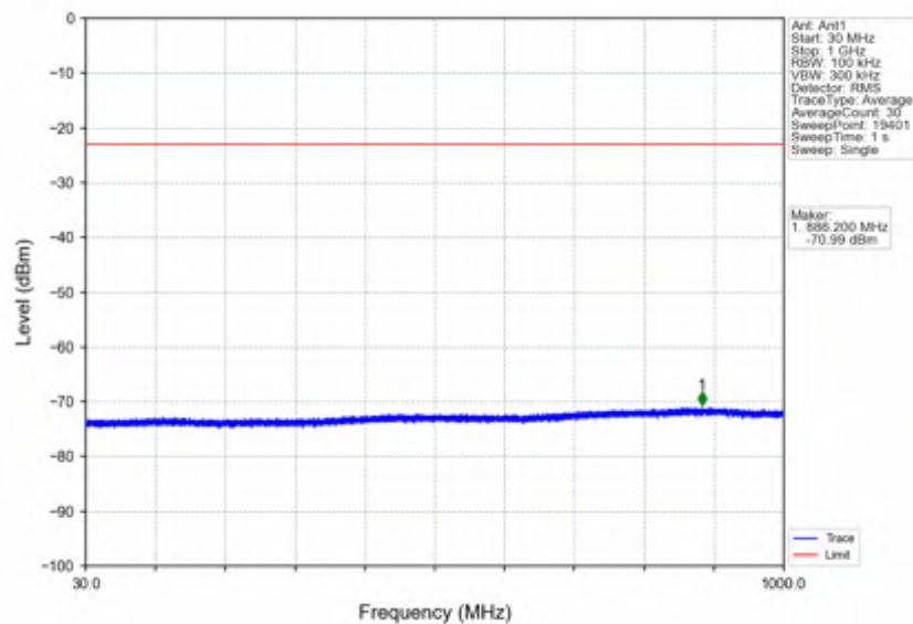
n7_15kHz_SISO_NTNV_25MHz_DFT-s-OFDM_PI/2_BPSK_2535MHz_Edge_1RB_Left
