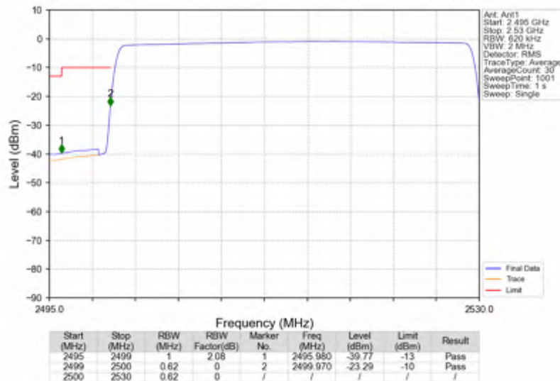
n7_15kHz_SISO_NTNV_30MHz_CP-OFDM QPSK_2515MHz_Outer_Full
