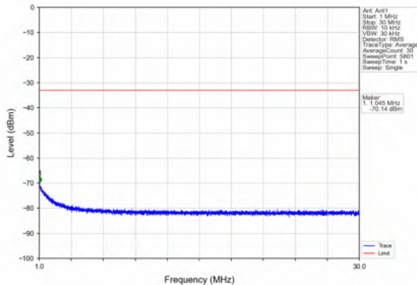
n7_15kHz_SISO_NTNV_30MHz_DFT-s-OFDM QPSK_2535MHz_Edge_1RB_Left
