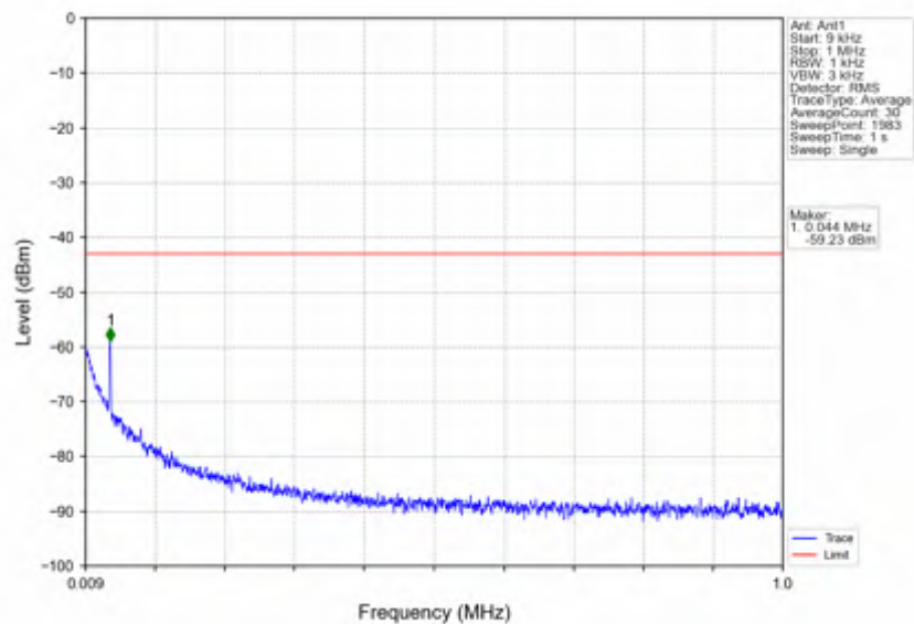
n7_15kHz_SISO_NTNV_30MHz_CP-OFDM_QPSK_2555MHz_Outer_Full
