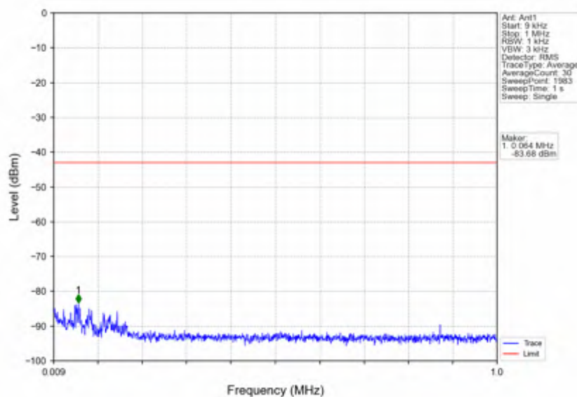
n7_15kHz_SISO_NTNV_30MHz_DFT-s-OFDM_PI/2_BPSK_2515MHz_Edge_1RB_Left
