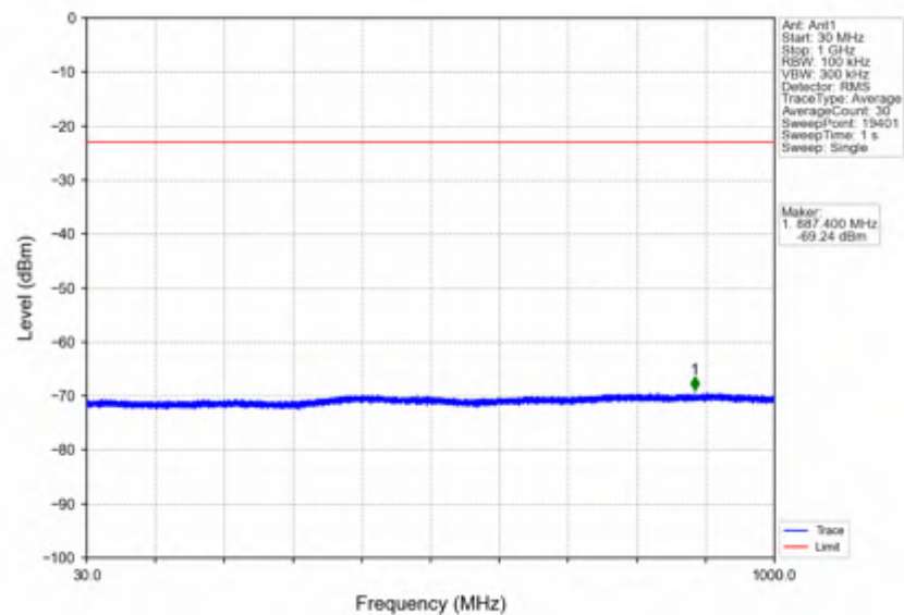
n7_15kHz_SISO_NTNV_30MHz_CP-OFDM_QPSK_2555MHz_Outer_Full
