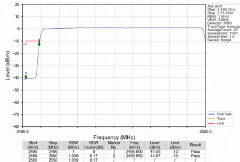
n7_15kHz_SISO_NTNV_50MHz_DFT-s-OFDM_QPSK_2525MHz_Outer_Full
