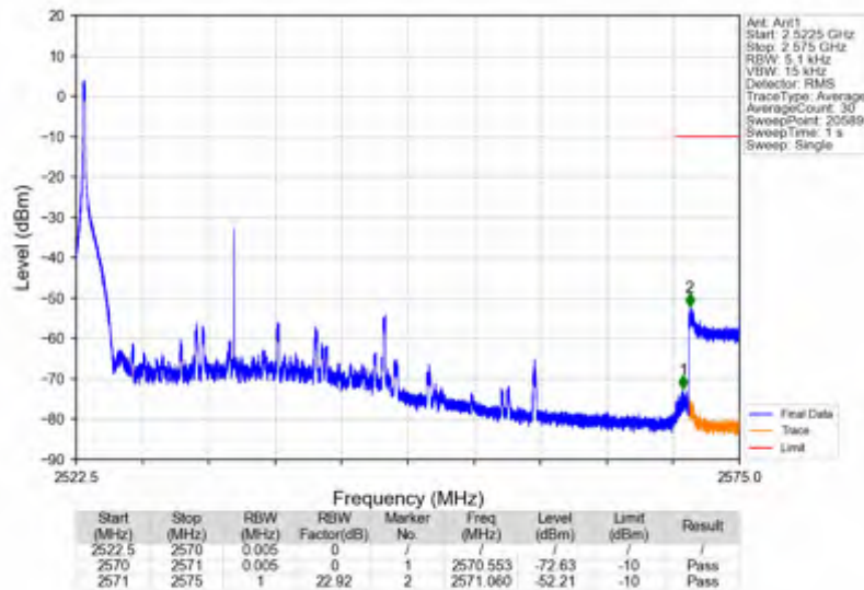
n7_15kHz_SISO_NTNV_25MHz_DFT-s-OFDM QPSK_2535MHz_Edge_1RB_Left
