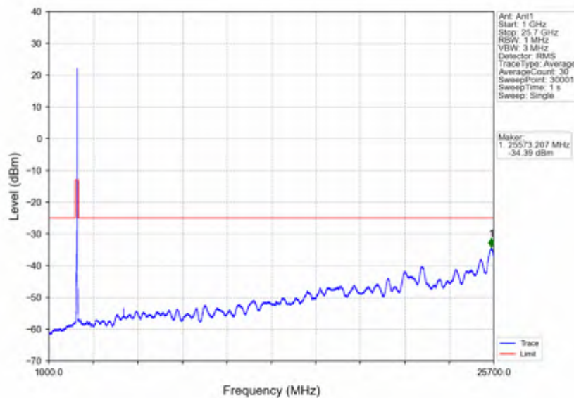
n7_15kHz_SISO_NTNV_50MHz_DFT-s-OFDM QPSK_2525MHz_Edge_1RB_Left
