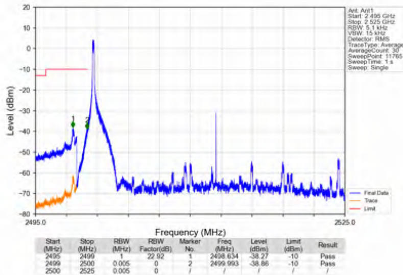
n7_15kHz_SISO_NTNV_25MHz_DFT-s-OFDM QPSK 2512.5MHz_Edge_1RB_Left
