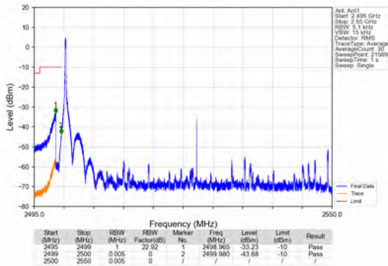
n7_15kHz_SISO_NTNV_50MHz_DFT-s-OFDM_PI/2_BPSK_2525MHz_Edge_1RB_Left
