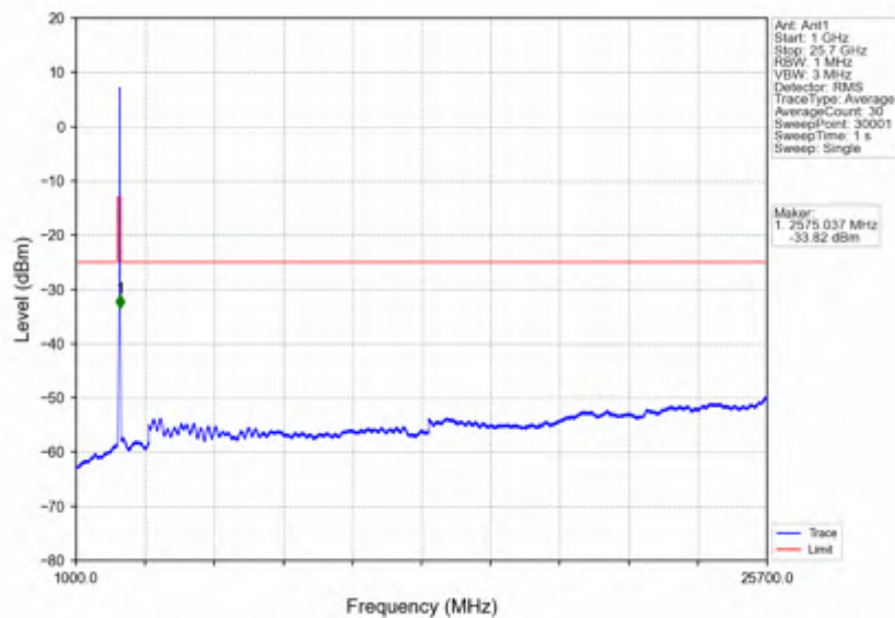
n7_15kHz_SISO_NTNV_25MHz_CP-OFDM QPSK_2557.5MHz_Outer_Full
