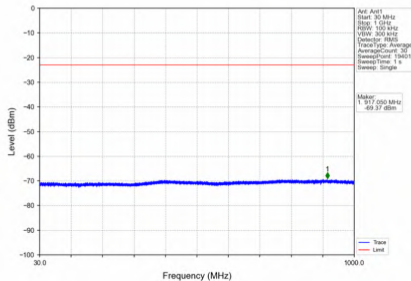
n7 15kHz SISO NTNV 50MHz DFT-s-OFDM PI/2 BPSK 2545MHz Outer Full
