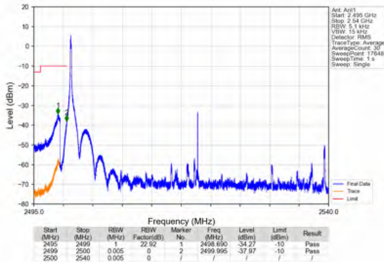
n7_15kHz_SISO_NTNV_40MHz_DFT-s-OFDM QPSK_2520MHz_Edge_1RB_Left
