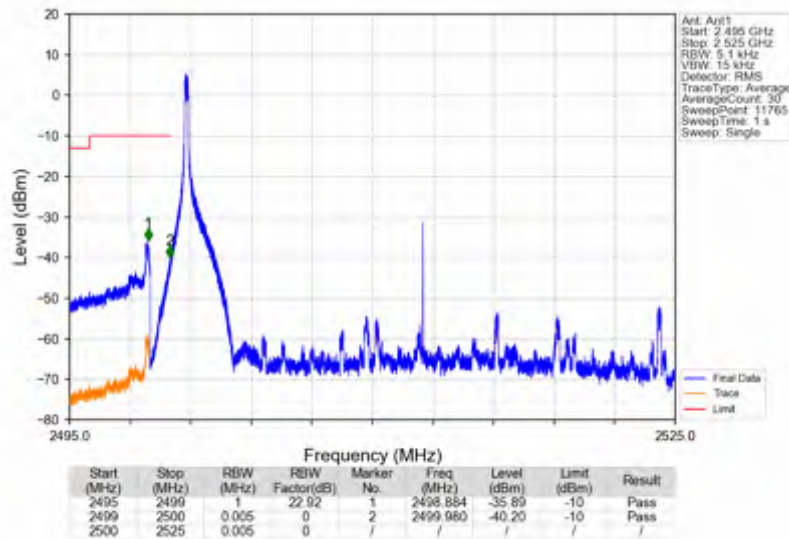
n7_15kHz_SISO_NTNV_25MHz_DFT-s-OFDM QPSK_2512.5MHz_Inner_1RB_Left
