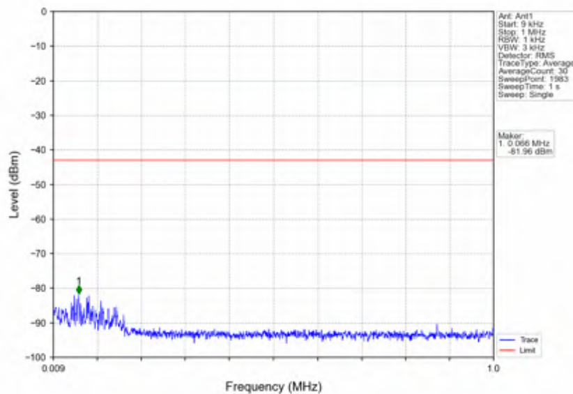
n7_15kHz_SISO_NTNV_25MHz_DFT-s-OFDM QPSK_2535MHz_Edge_1RB_Left
