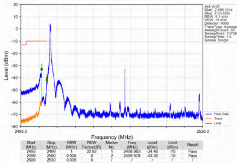
n7_15kHz_SISO_NTNV_30MHz_DFT-s-OFDM_PI/2_BPSK_2515MHz_Edge_1RB_Left
