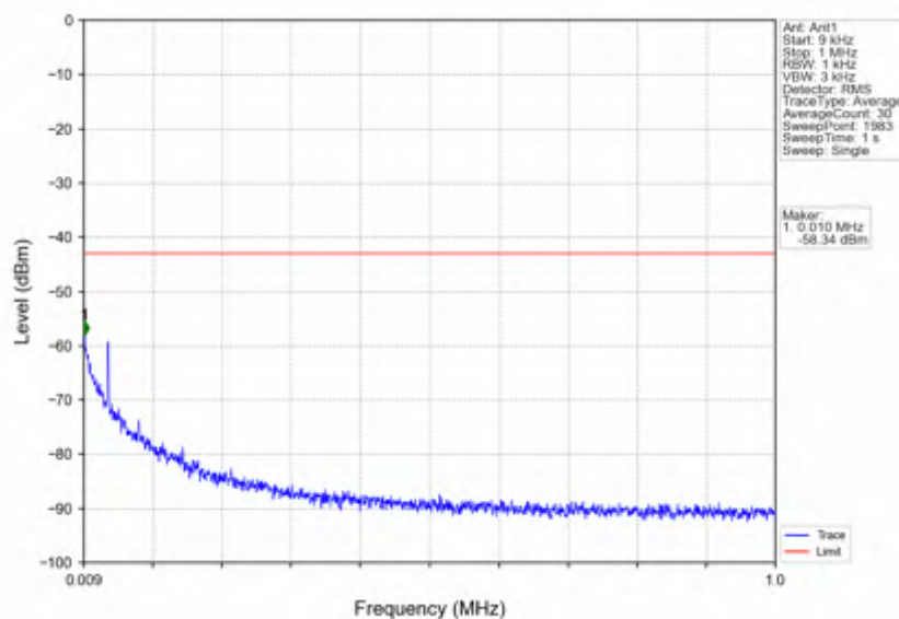
n7_15kHz_SISO_NTNV_50MHz_DFT-s-OFDM_PI/2_BPSK_2525MHz_Edge_1RB_Left
