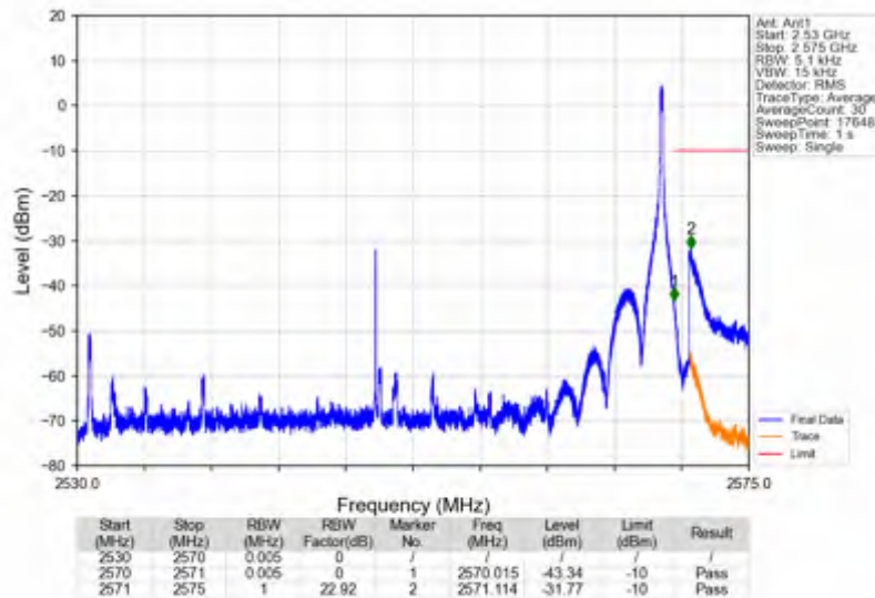
n7_15kHz_SISO_NTNV_40MHz_DFT-s-OFDM QPSK_2550MHz_Inner_1RB_Right
