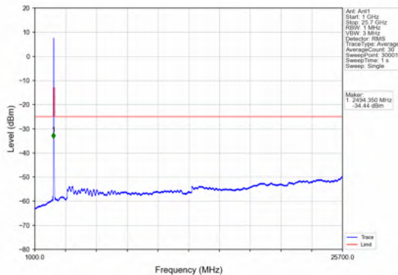
n7_15kHz_SISO_NTNV_25MHz_CP-OFDM QPSK_2512.5MHz_Outer_Full
