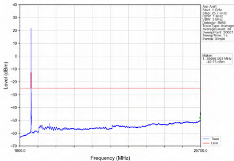
n7_15kHz_SISO_NTNV_25MHz_DFT-s-OFDM_PI/2_BPSK_2535MHz_Edge_1RB_Left
