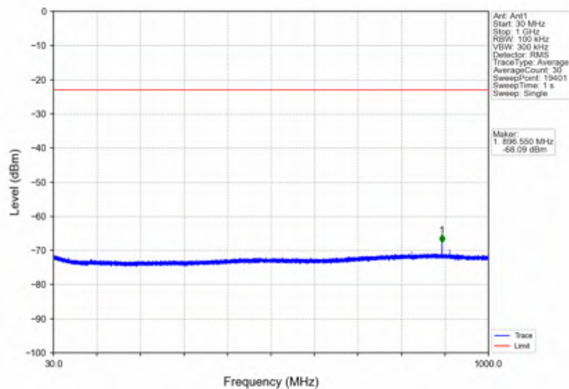
n7_15kHz_SISO_NTNV_25MHz_CP-OFDM QPSK_2557.5MHz_Outer_Full
