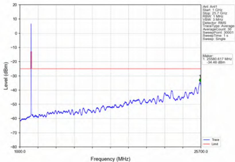
n7_15kHz_SISO_NTNV_30MHz_CP-OFDM_QPSK_2515MHz_Outer_Full
