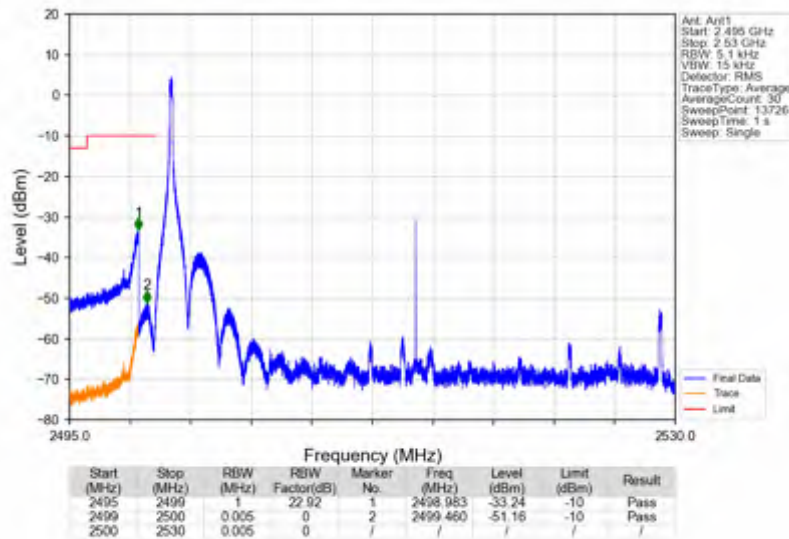
n7_15kHz_SISO_NTNV_30MHz_DFT-s-OFDM_QPSK_2515MHz_Inner_1RB_Left
