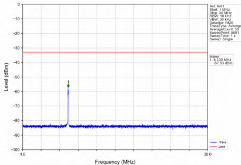
n7_15kHz_SISO_NTNV_25MHz_DFT-s-OFDM_QPSK_2557.5MHz_Edge_1RB_Right
