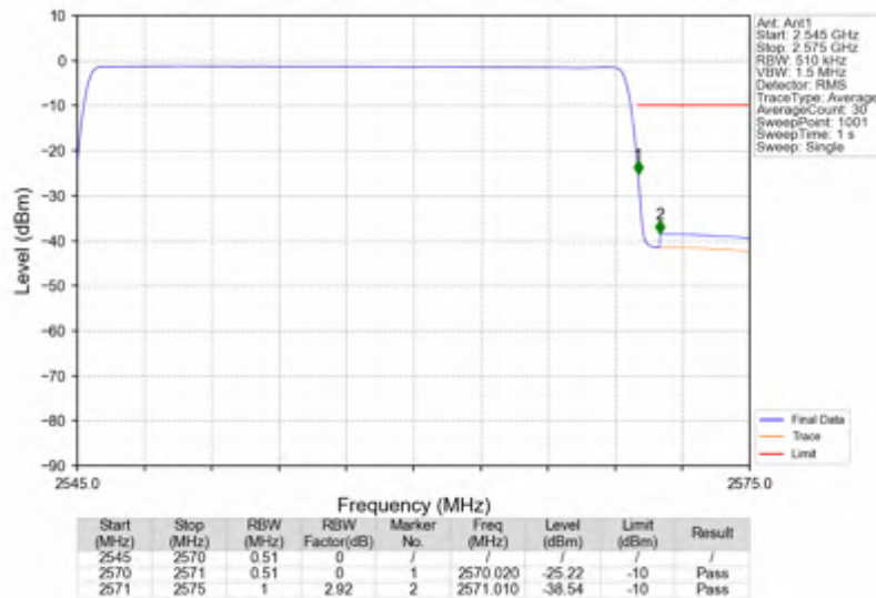
n7_15kHz_SISO_NTNV_25MHz_CP-OFDM QPSK_2557.5MHz_Outer_Full
