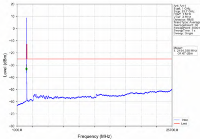
n7_15kHz_SISO_NTNV_30MHz_DFT-s-OFDM_QPSK_2515MHz_Inner_1RB_Left
