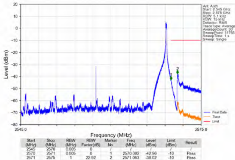
n7_15kHz_SISO_NTNV_25MHz_DFT-s-OFDM QPSK_2557.5MHz_Inner_1RB_Right
