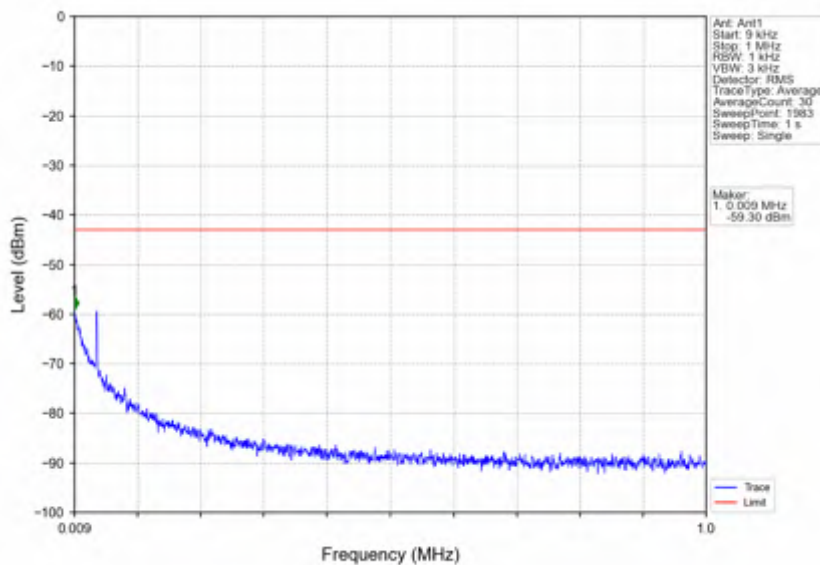
n7_15kHz_SISO_NTNV_40MHz_DFT-s-OFDM_QPSK_2550MHz_Outer_Full
