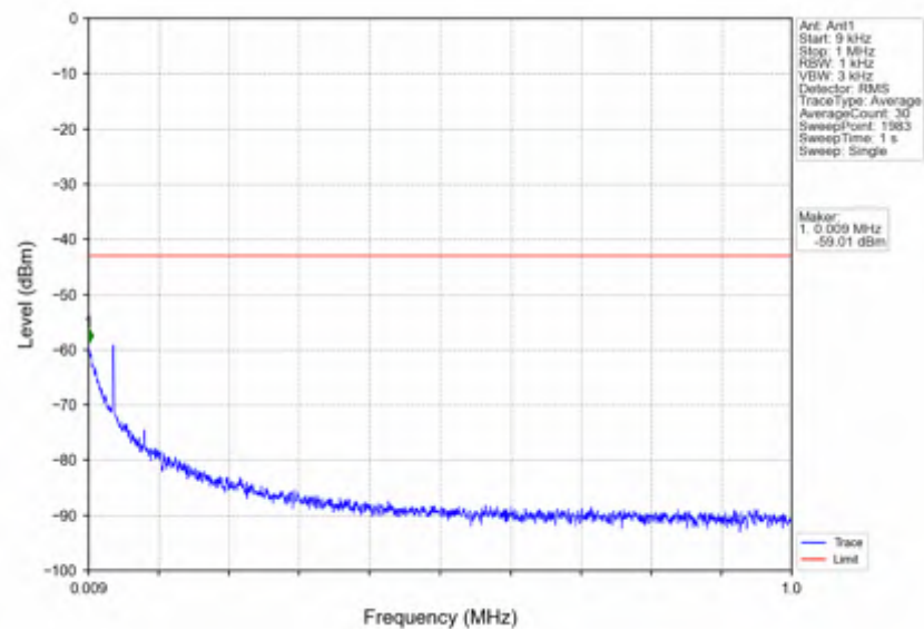
n7 15kHz SISO NTN 40MHz CP-OFDM QPSK 2520MHz Outer Full
