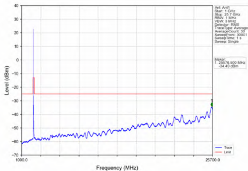
n7 15kHz SISO NTNV 50MHz DFT-s-OFDM QPSK 2525MHz Inner 1RB Left
