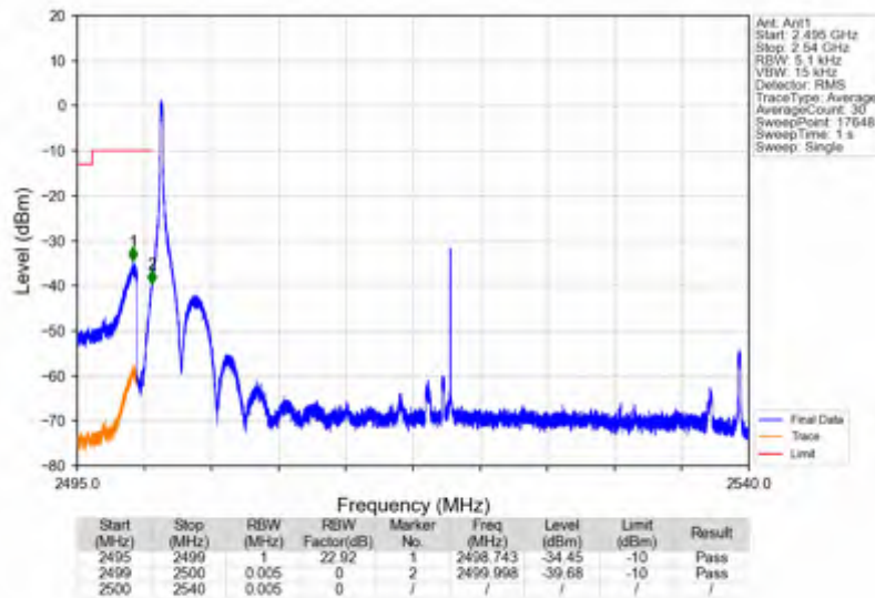
n7_15kHz_SISO_NTNV_40MHz_CP-OFDM QPSK_2520MHz_Edge_1RB_Left
