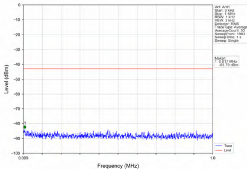
n7_15kHz_SISO_NTNV_25MHz_CP-OFDM QPSK_2557.5MHz_Outer_Full
