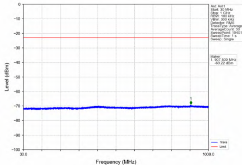
n7_15kHz_SISO_NTNV_30MHz_CP-OFDM_QPSK_2515MHz_Inner_1RB_Left
