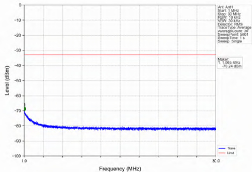
n7_15kHz_SISO_NTNV_30MHz_CP-OFDM QPSK_2515MHz_Outer_Full
