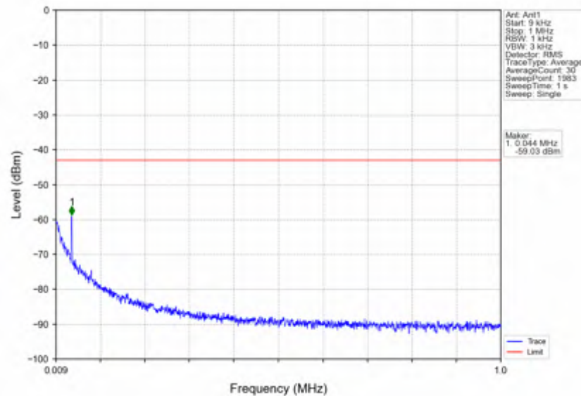
n7_15kHz_SISO_NTNV_50MHz_DFT-s-OFDM PI/2 BPSK_2525MHz_Outer_Full
