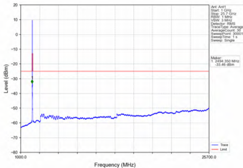
n7_15kHz_SISO_NTNV_25MHz_DFT-s-OFDM QPSK_2512.5MHz_Inner_1RB_Left
