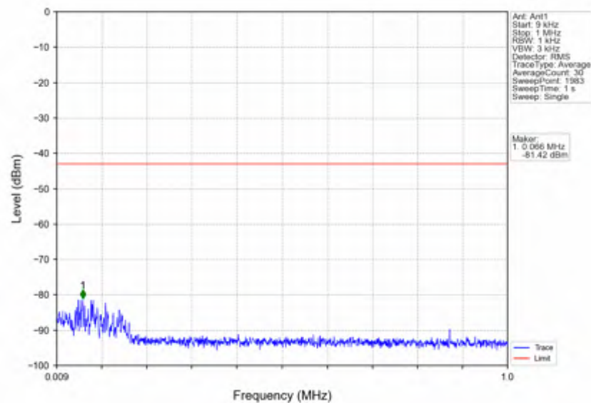
n7_15kHz_SISO_NTNV_25MHz_DFT-s-OFDM QPSK_2557.5MHz_Inner_1RB_Right
