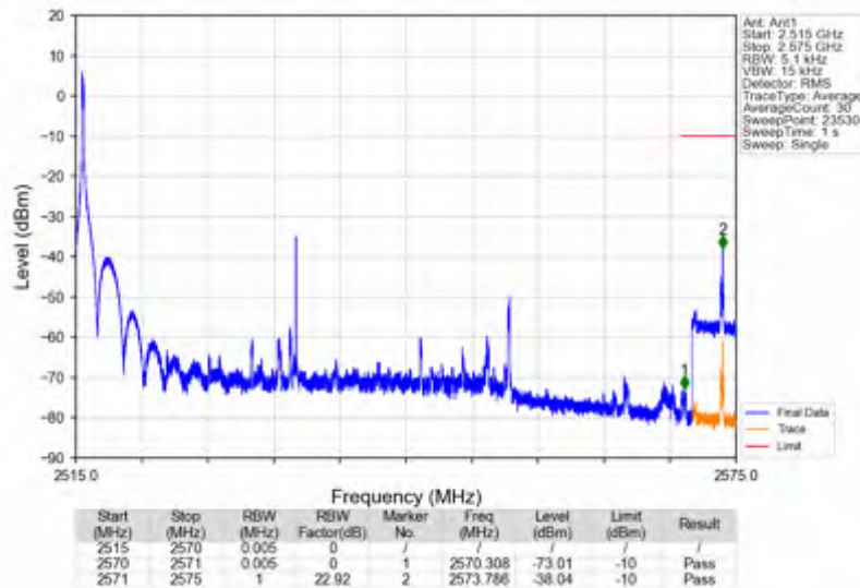
n7_15kHz_SISO_NTNV_40MHz_DFT-s-OFDM PI/2 BPSK_2535MHz_Edge_1RB_Left
