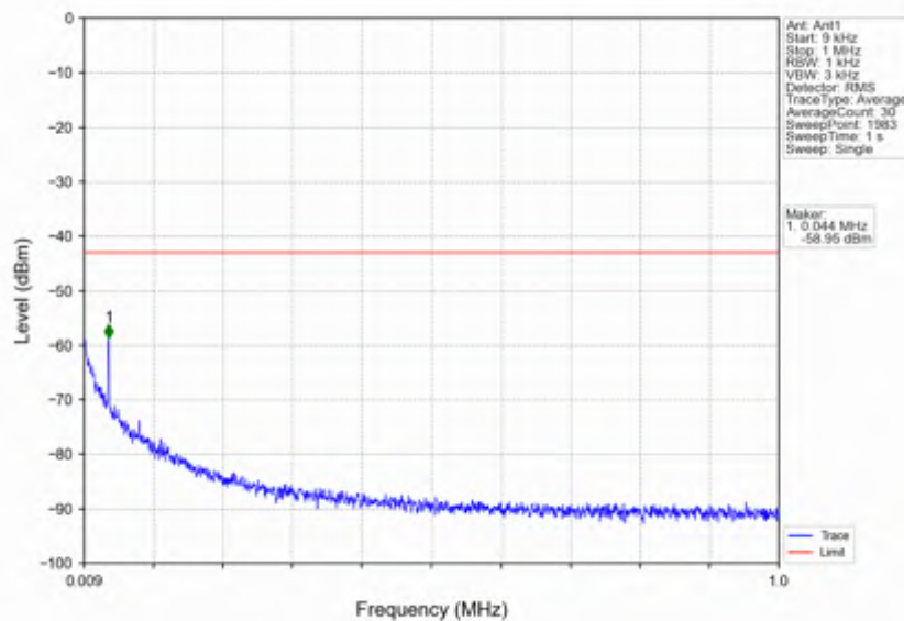
n7_15kHz_SISO_NTNV_40MHz_CP-OFDM QPSK_2520MHz_Edge_1RB_Left
