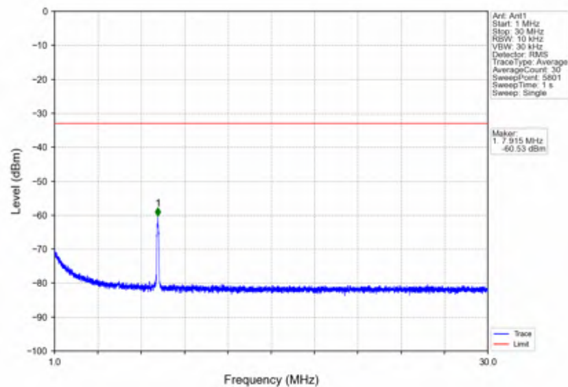
n7_15kHz_SISO_NTNV_40MHz_CP-OFDM_QPSK_2550MHz_Inner_1RB_Right
