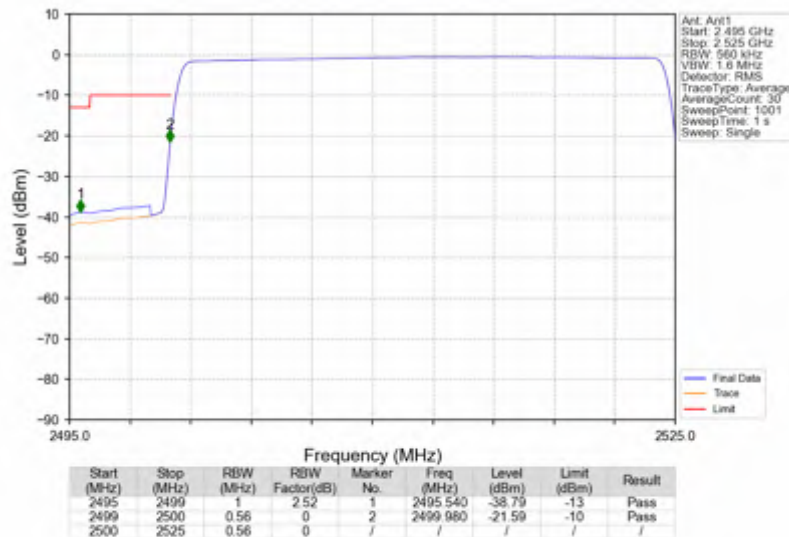
n7_15kHz_SISO_NTNV_25MHz_CP-OFDM QPSK_2512.5MHz_Outer_Full
