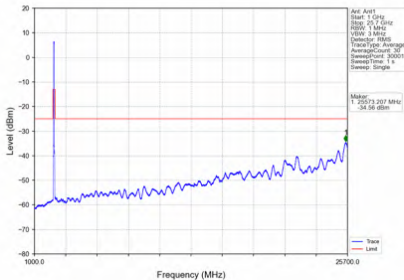
n7_15kHz_SISO_NTNV_50MHz_DFT-s-OFDM_QPSK_2525MHz_Inner_1RB_Left
