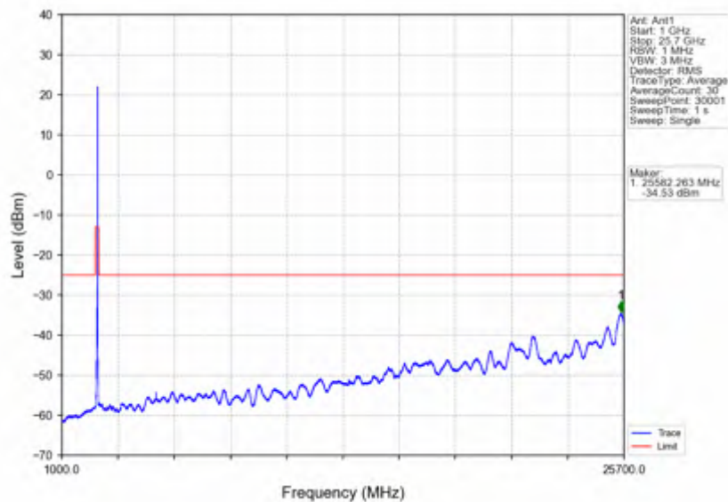
n7_15kHz_SISO_NTNV_40MHz_DFT-s-OFDM PI/2 BPSK_2550MHz_Outer_Full
