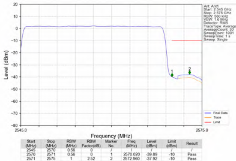
n7_15kHz_SISO_NTNV_25MHz_DFT-s-OFDM PI/2 BPSK_2557.5MHz_Outer_Full
