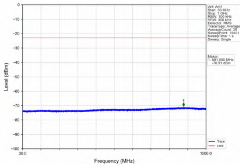
n7_15kHz_SISO_NTNV_25MHz_CP-OFDM QPSK_2557.5MHz_Edge_1RB_Right
