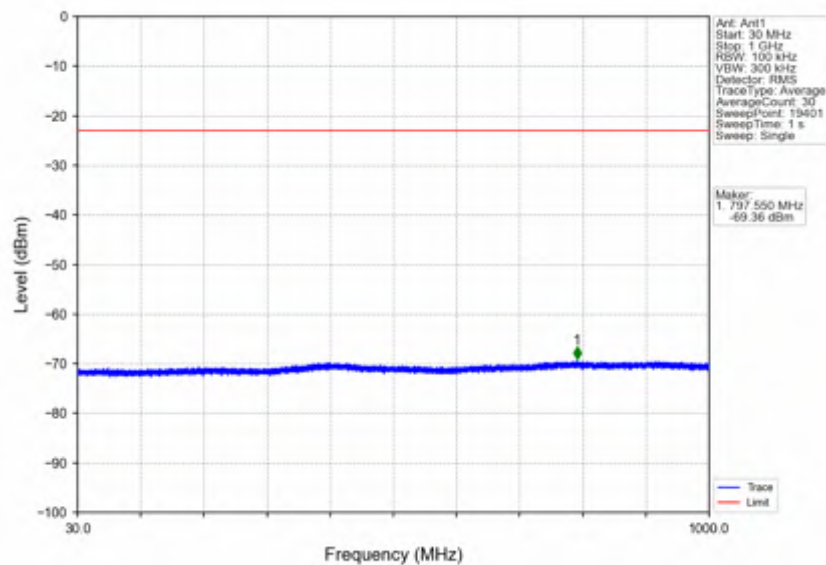
n7_15kHz_SISO_NTNV_40MHz_DFT-s-OFDM_PI/2_BPSK_2535MHz_Edge_1RB_Left
