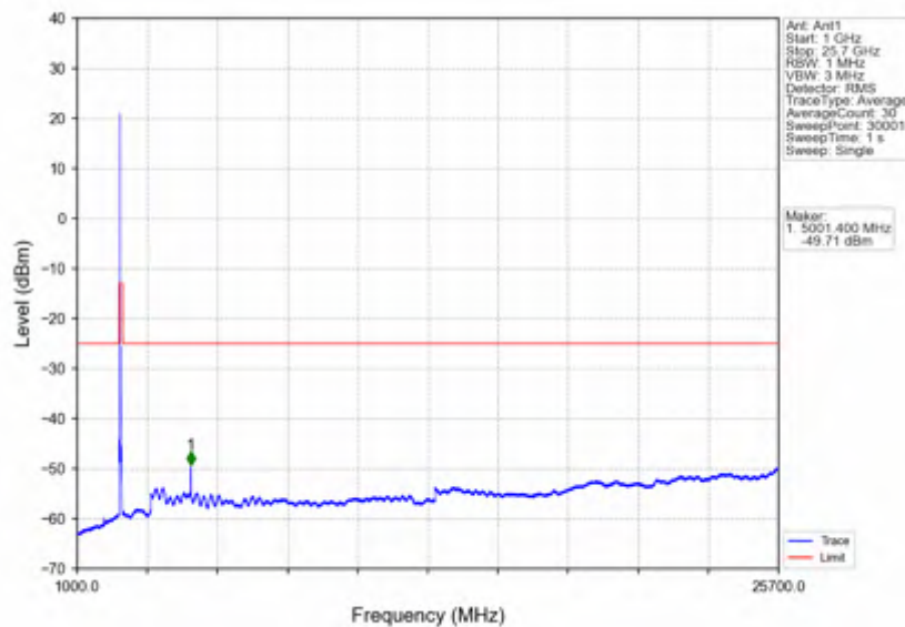
n7_15kHz_SISO_NTNV_30MHz_DFT-s-OFDM PI/2 BPSK_2515MHz_Outer_Full
