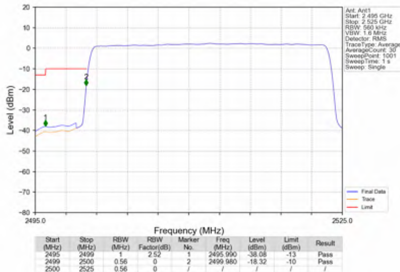
n7_15kHz_SISO_NTNV_25MHz_DFT-s-OFDM PI/2 BPSK_2512.5MHz_Outer_Full
