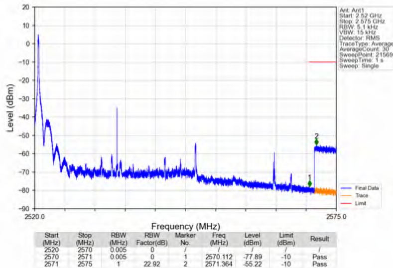
n7_15kHz_SISO_NTNV_30MHz_DFT-s-OFDM PI/2 BPSK_2535MHz_Edge_1RB_Left
