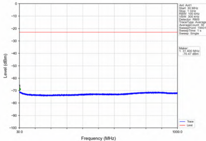
n7_15kHz_SISO_NTNV_20MHz_CP-OFDM_QPSK_2560MHz_Outer_Full
