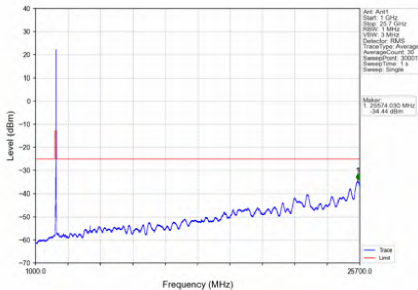
n7_15kHz_SISO_NTNV_40MHz_DFT-s-OFDM QPSK_2520MHz_Edge_1RB_Left
