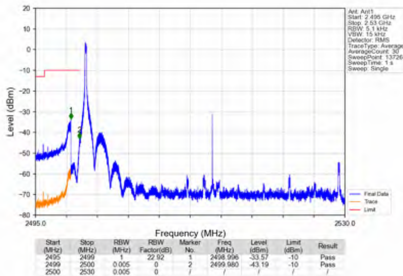
n7_15kHz_SISO_NTNV_30MHz_DFT-s-OFDM QPSK_2515MHz_Edge_1RB_Left
