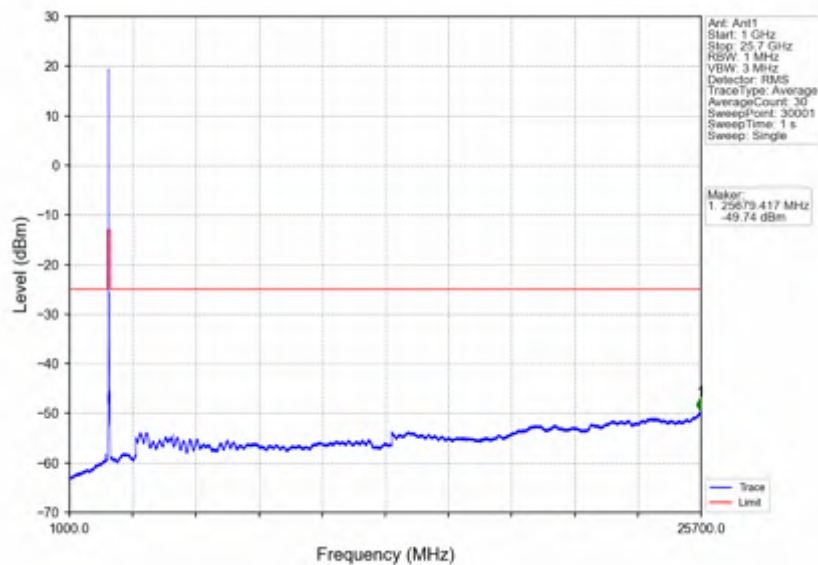
n7_15kHz_SISO_NTNV_25MHz_CP-OFDM QPSK_2535MHz_Edge_1RB_Left
