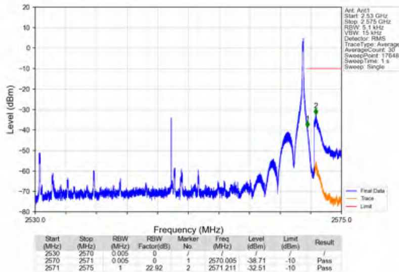
n7_15kHz_SISO_NTNV_40MHz_DFT-s-OFDM QPSK_2550MHz_Edge_1RB_Right
