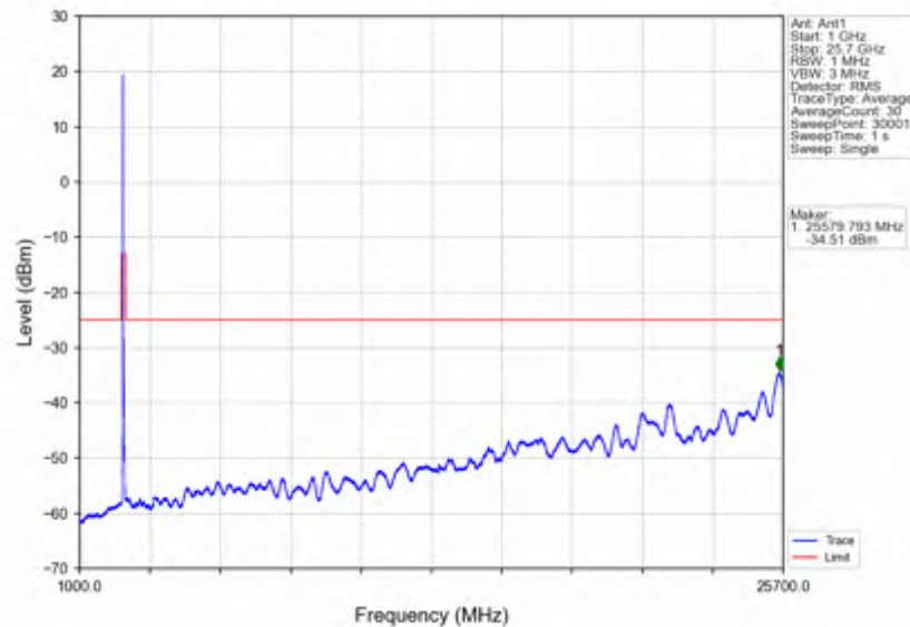
n7_15kHz_SISO_NTNV_40MHz_CP-OFDM QPSK_2535MHz_Edge_1RB_Left
