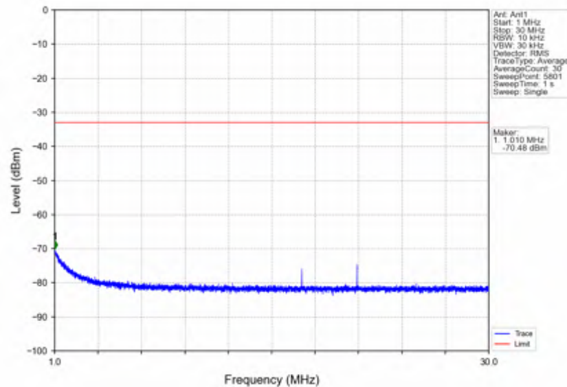
n7_15kHz_SISO_NTNV_40MHz_DFT-s-OFDM PI/2 BPSK_2520MHz_Outer_Full
