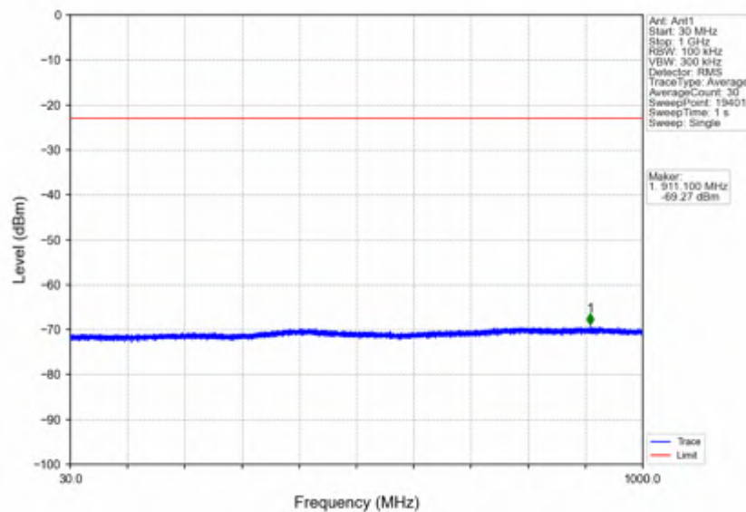
n7_15kHz_SISO_NTNV_40MHz_DFT-s-OFDM_QPSK_2550MHz_Inner_1RB_Right
