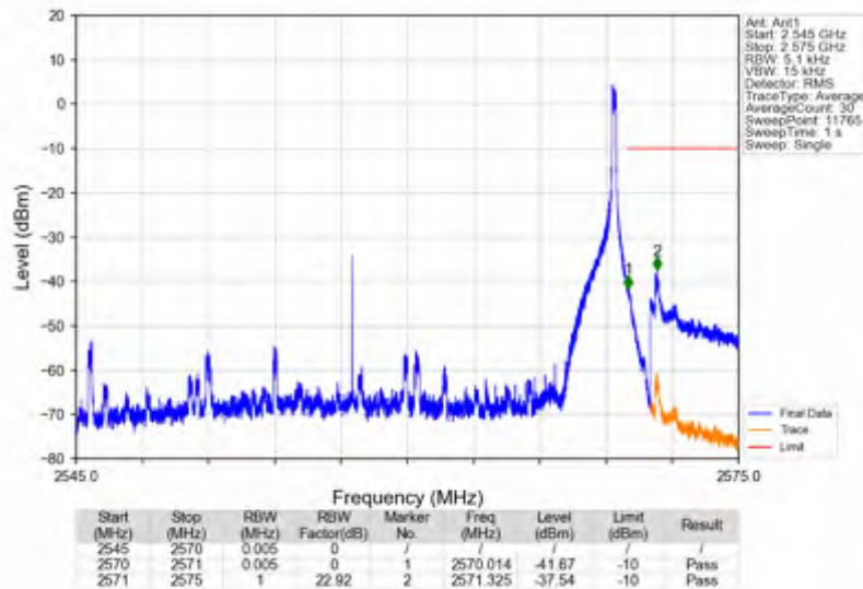
n7_15kHz_SISO_NTNV_25MHz_DFT-s-OFDM QPSK_2557.5MHz_Edge_1RB_Right
