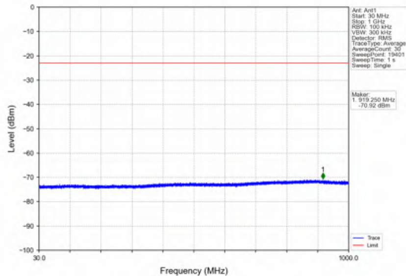
n7_15kHz_SISO_NTNV_25MHz_CP-OFDM_QPSK_2512.5MHz_Inner_1RB_Left
