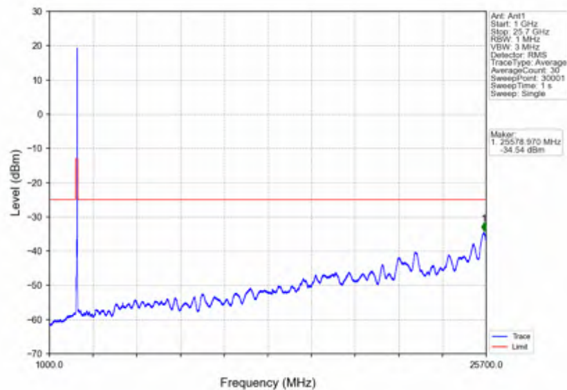
n7_15kHz_SISO_NTNV_30MHz_CP-OFDM QPSK_2555MHz_Outer_Full
