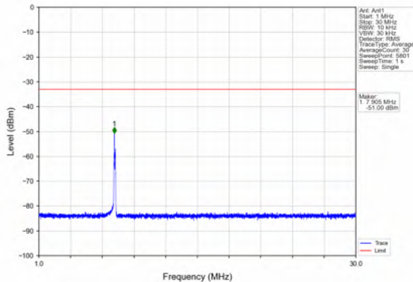
n7_15kHz_SISO_NTNV_25MHz_DFT-s-OFDM PI/2 BPSK_2557.5MHz_Inner_1RB_Right
