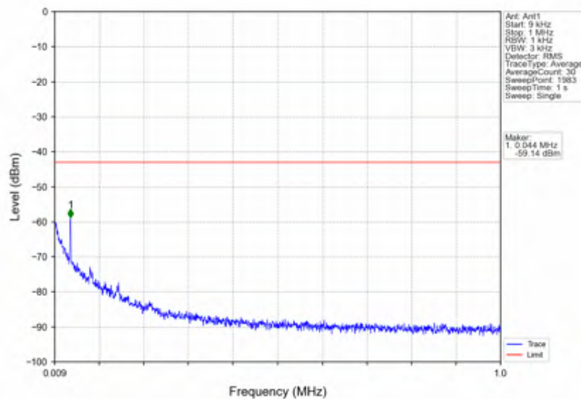
n7 15kHz SISO NTNV 50MHz DFT-s-OFDM QPSK 2525MHz Inner 1RB Left
