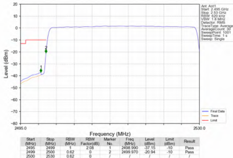
n7_15kHz_SISO_NTNV_30MHz_DFT-s-OFDM PI/2 BPSK_2515MHz_Outer_Full
