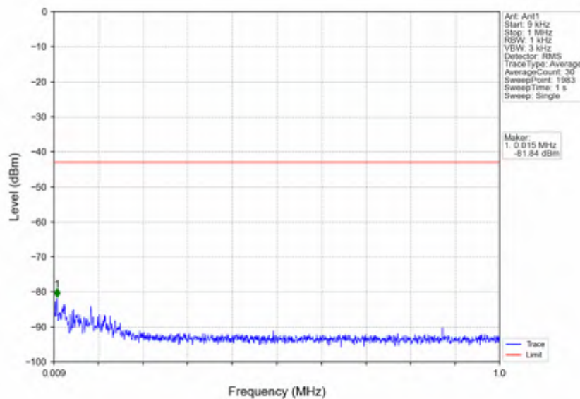
n7_15kHz_SISO_NTNV_25MHz_CP-OFDM_QPSK_2512.5MHz_Edge_1RB_Left
