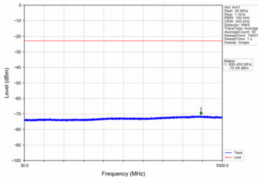
n7_15kHz_SISO_NTNV_25MHz_CP-OFDM QPSK_2512.5MHz_Outer_Full
