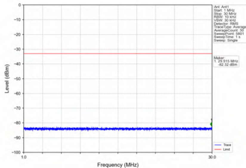
n7_15kHz_SISO_NTNV_30MHz_CP-OFDM QPSK_2515MHz_Edge_1RB_Left
