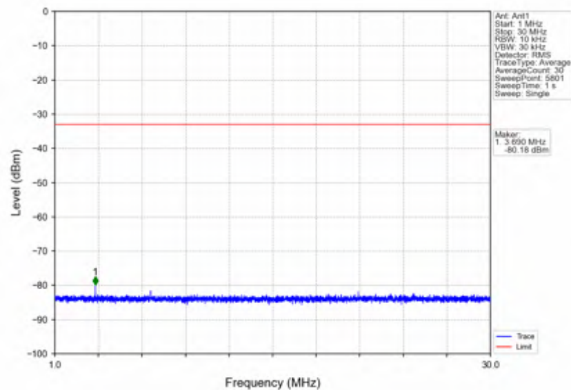
n7_15kHz_SISO_NTNV_30MHz_DFT-s-OFDM_PI/2_BPSK_2515MHz_Outer_Full
