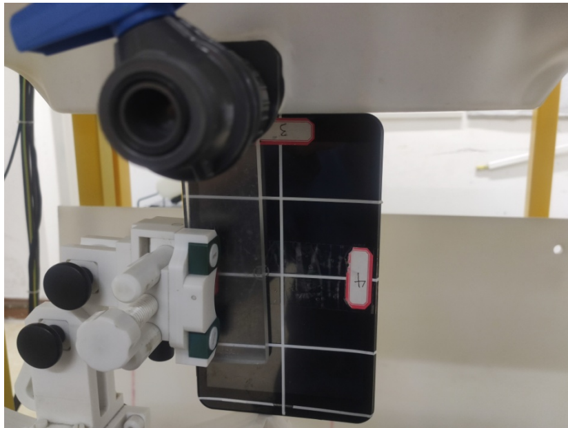
Edge 3 for WWAN (Test distance: 0mm)
