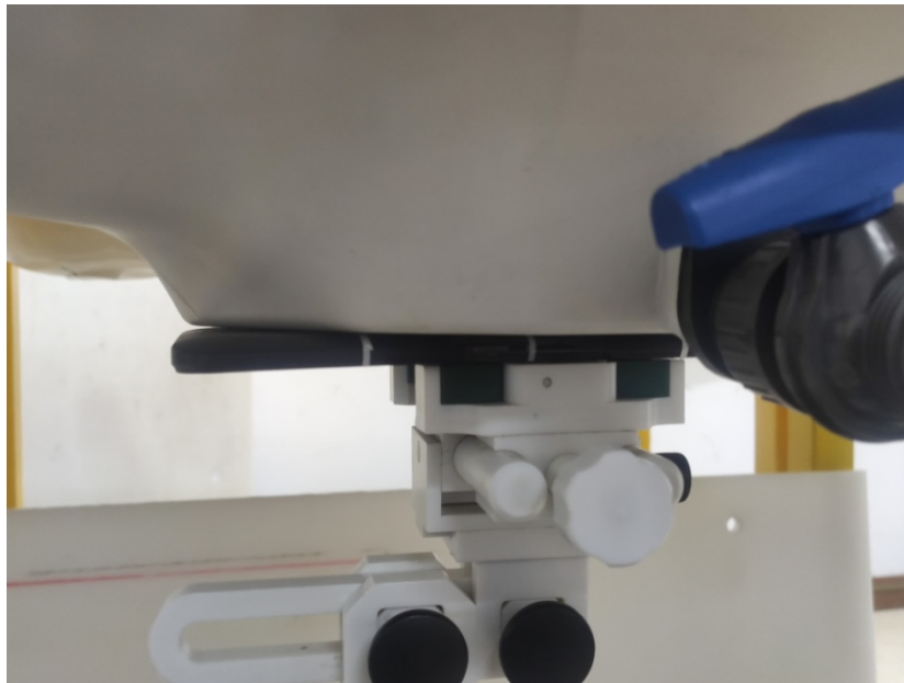
Bottom Face for WLAN (Test distance: 0mm)
