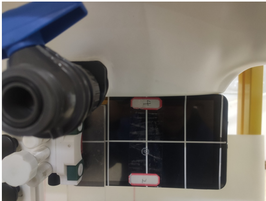
Edge 4 for WWAN (Test distance: 0mm)
