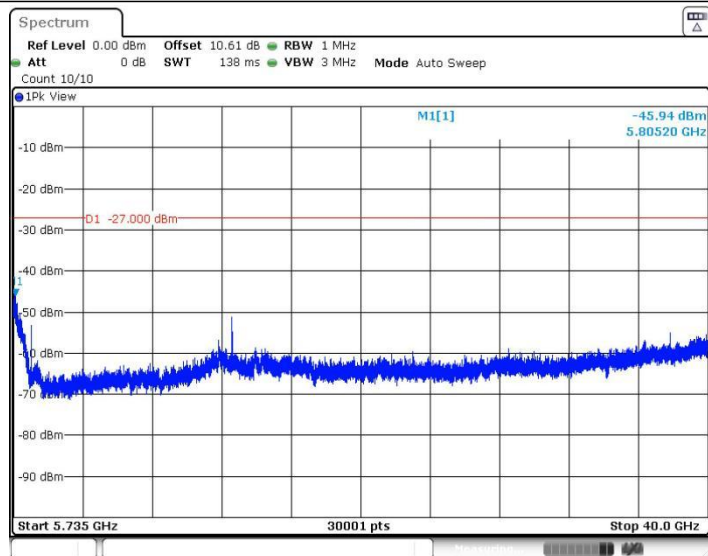
11AC20SISO_Ant1_5500_5735~40000
