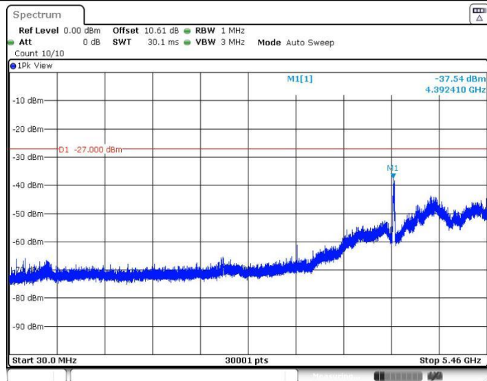
11AC20SISO_Ant1_5500_30~5460
