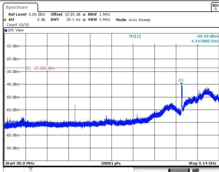
11AX20SISO_Ant1_5320_30~5140
