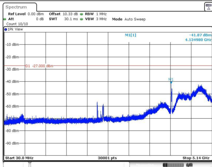
11AX20SISO_Ant1_5180_30~5140
