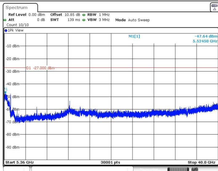
11AX20SISO_Ant1_5320_5360~40000
