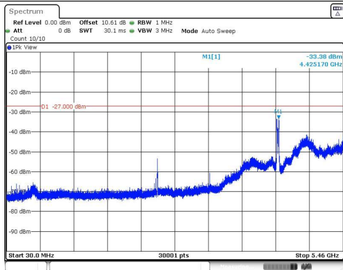
11AC40SISO_Ant1_5510_30~5460
