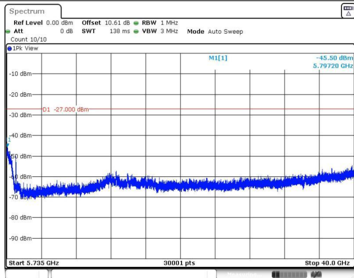
11AC40SISO_Ant1_5510_5735~40000
