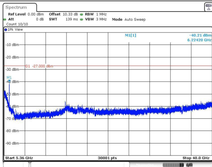
11AX20SISO_Ant1_5180_5360~40000
