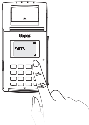
Fig. 2.2 - Setting Menu
