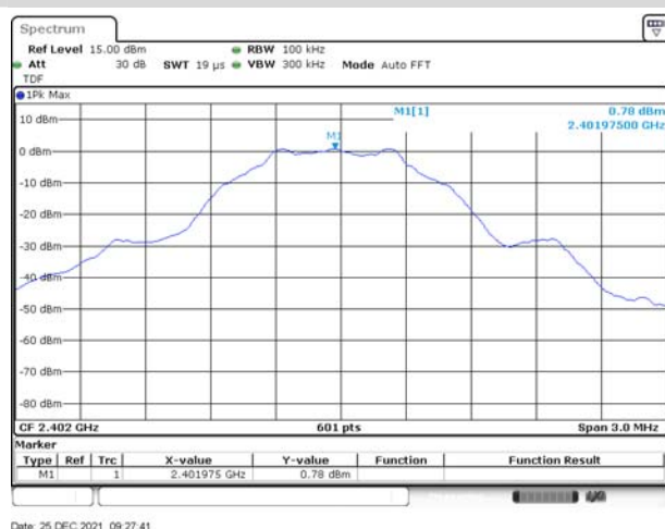
GFSK (BLE 1Mbps) LOW CHANNEL, CARRIER LEVEL
