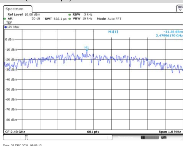
GFSK (BLE 1Mbps) HIGH CHANNEL
