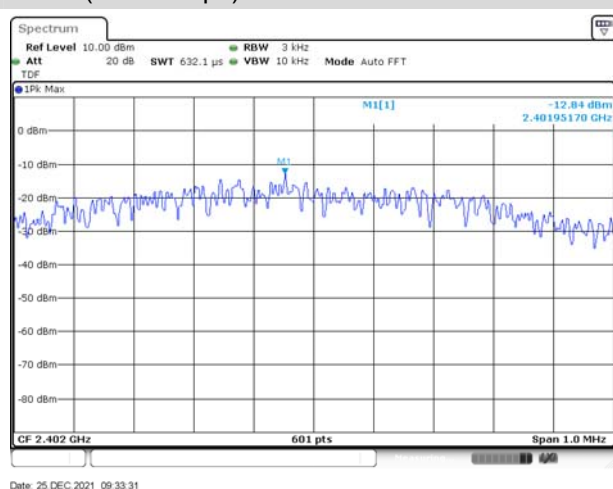
GFSK (BLE 1Mbps) LOW CHANNEL
