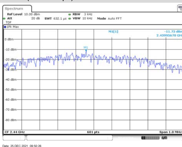
GFSK (BLE 1Mbps) MIDDLE CHANNEL
