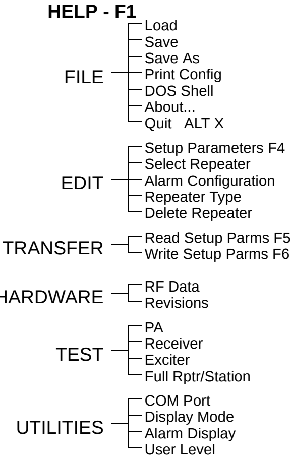
Figure 3-2 PROGRAMMING FLOWCHART
