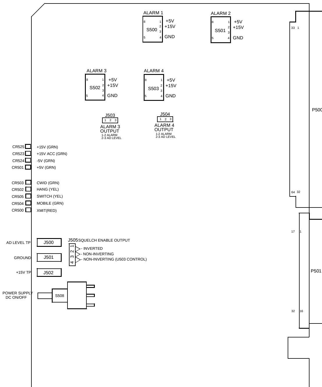
Figure 7-14 INTERFACE ALARM CARD ALIGNMENT POINTS
