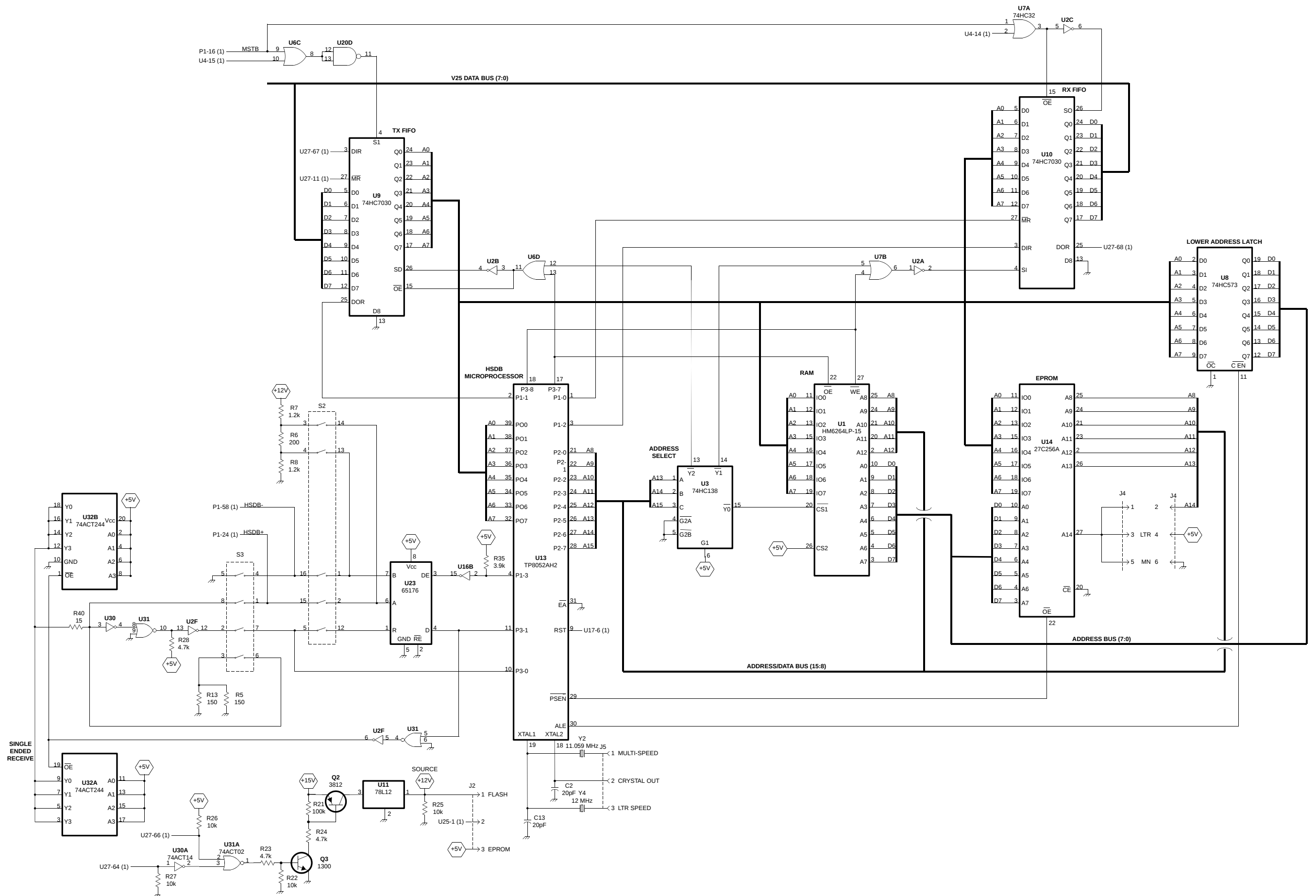
MPC SCHEMATIC (2 OF 2) FIGURE 10-23 10-18
