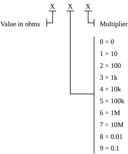
Figure 8-5 3-DIGIT RESISTOR
