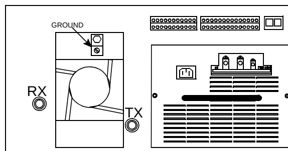
Figure 2-8 ANTENNA CONNECTIONS
