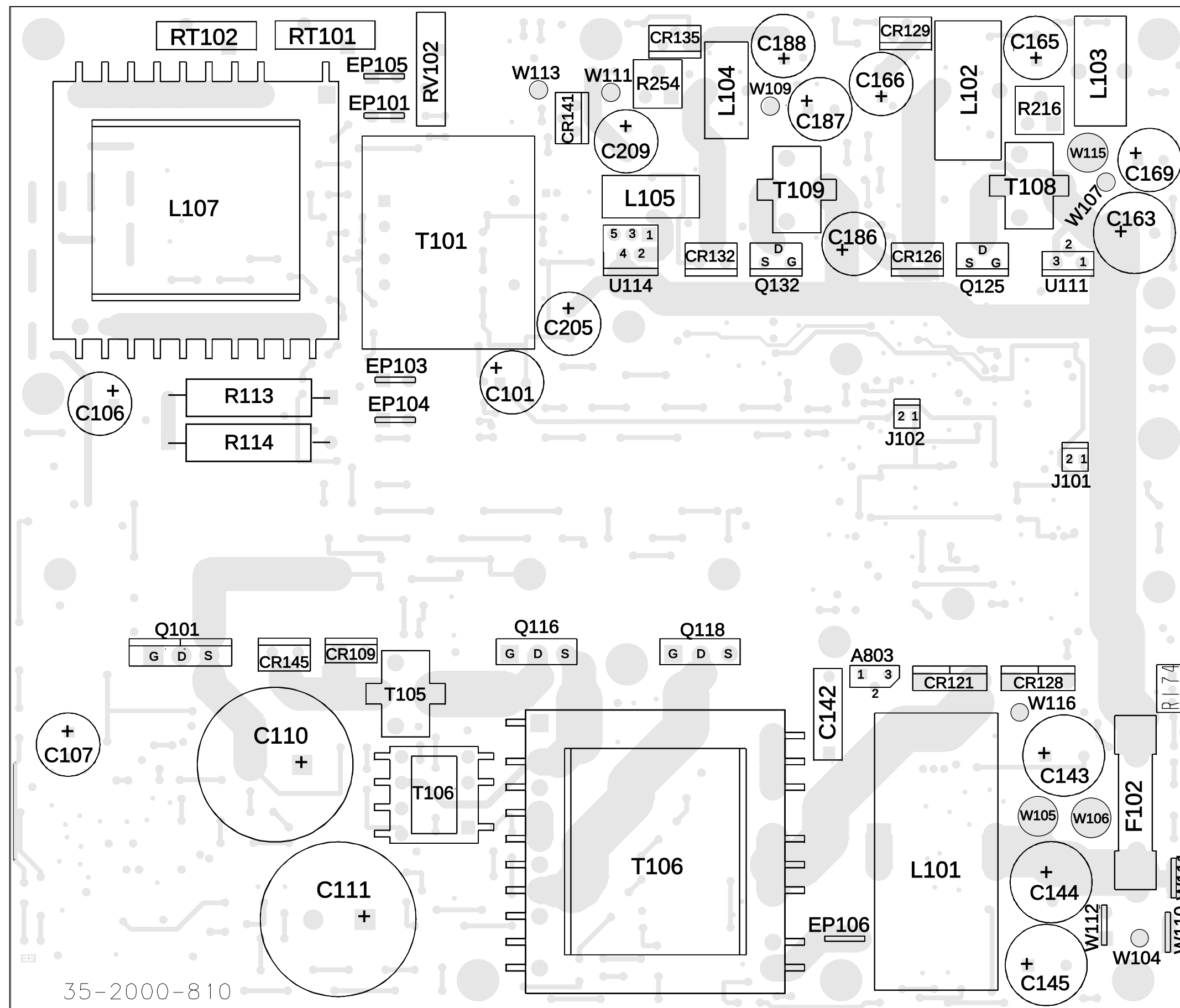
800W POWER SUPPLY COMPONENT LAYOUT (COMPONENT SIDE VIEW) FIGURE 10-35 10-30
