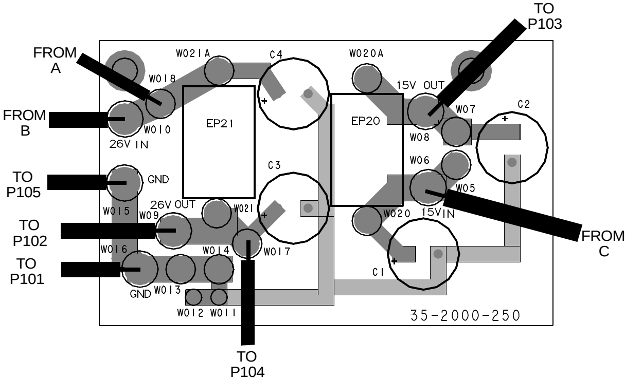
POWER FILTER BOARD COMPONENT LAYOUT FIGURE 10-41
