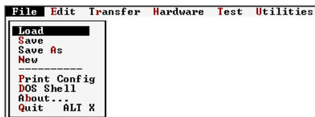
Figure 4-1 FILE MENU
