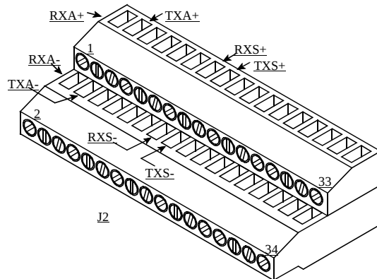
Figure 7-11 J2 TERMINAL BLOCK
