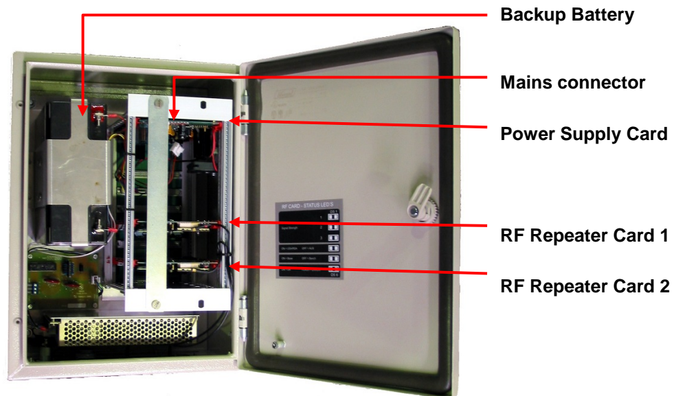
Figure 2: Repeater components
