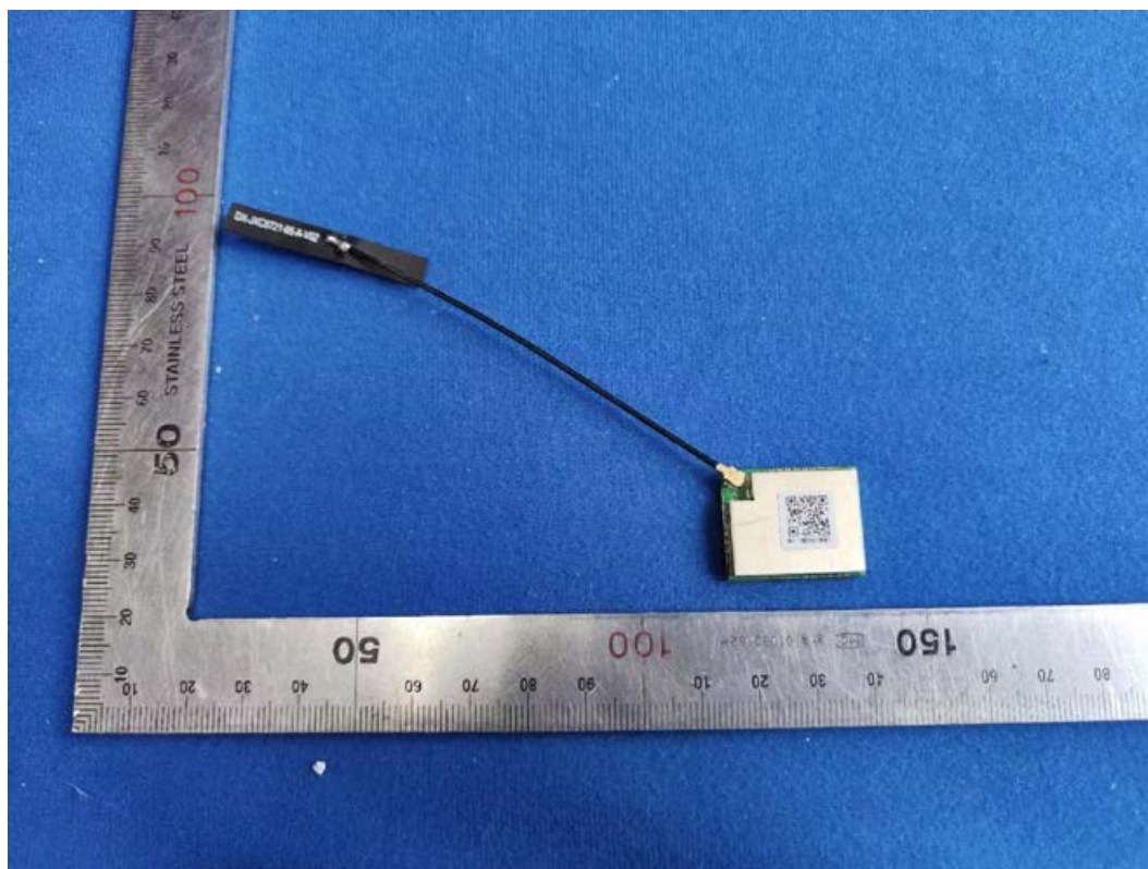
FIGURE 1 RTL8721DM MODULE (M/N: JXC8721-65) GENERAL APPEARANCE
