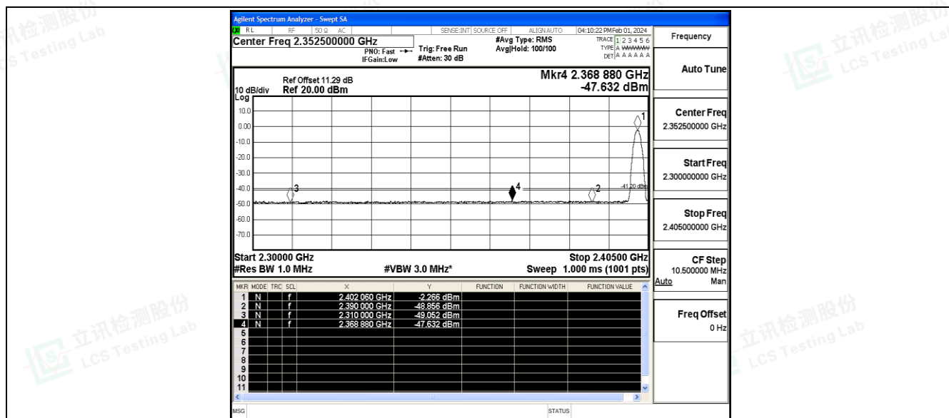
3DH5_Ant1_Low_2402_Peak
