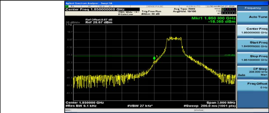
(Channel Bandwidth 3 MHz)_LCH_16QAM_15RB#0
