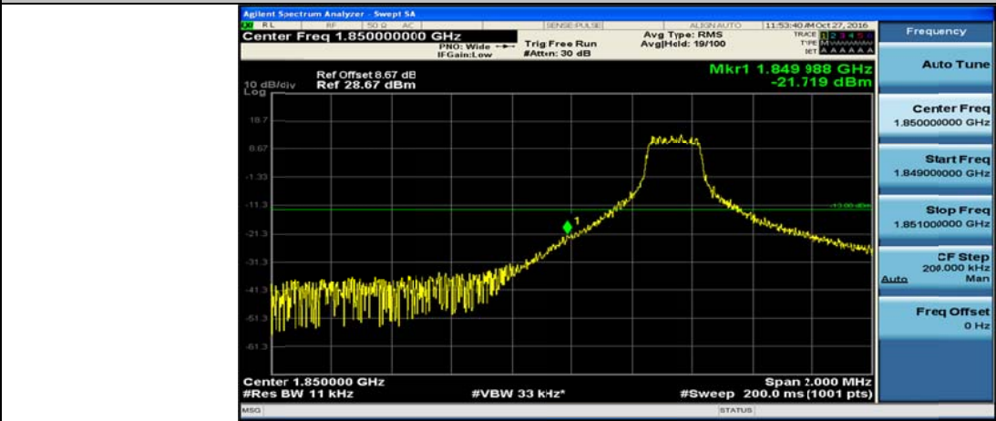
(Channel Bandwidth 5 MHz)_LCH_QPSK_25RB#0
