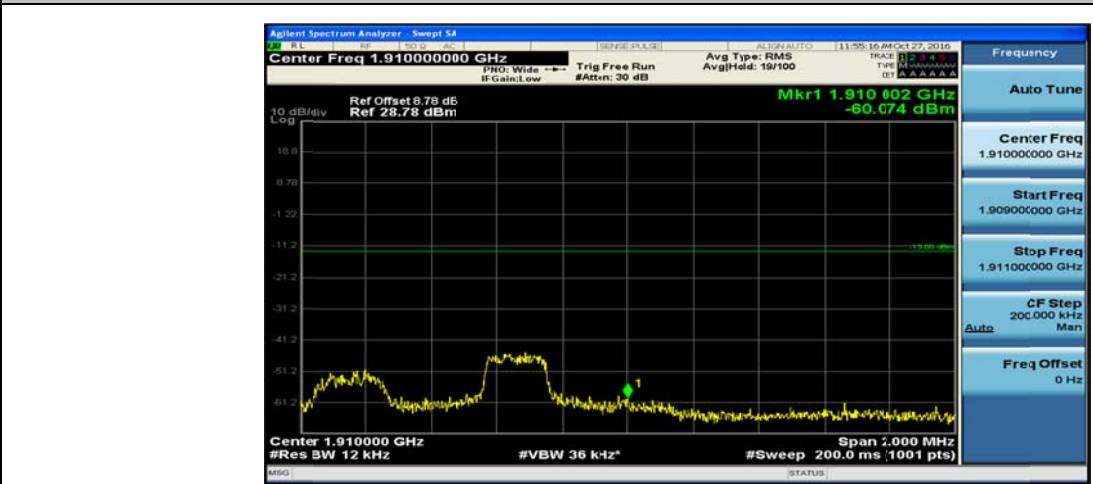
(Channel Bandwidth 5 MHz)_HCH_QPSK_1RB#0
