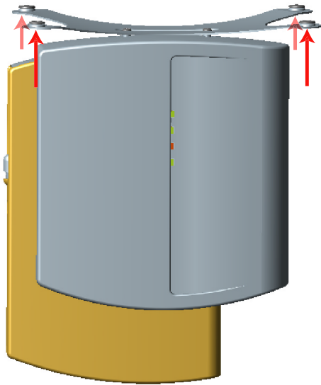
Figure 2-14 Mounting the AP-600 to the Ceiling
