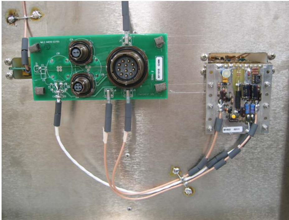
TOP VIEW CLOSE UP OF THE ELECTRONICS. FROM LEFT TO RIGHT: IMPULSE GENERATOR, ELECTRONICS INTERFACE, AND DIFFERENTIAL SAMPLER
