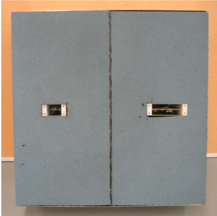
BOTTOM VIEW SHOWING FANS REMOVED IMPULSE GENERATOR ON LEFT. DIFFERENTIAL SAMPLER ON RIGHT
