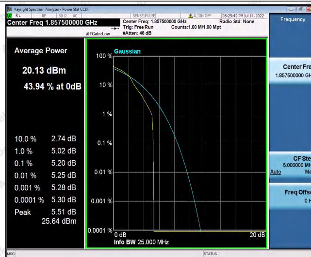
Band2-15MHz-16QAM-18675-5RB#0
