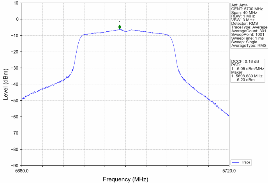
802.11n(HT20)_HCH_5700MHz_MIMO_NTNV
