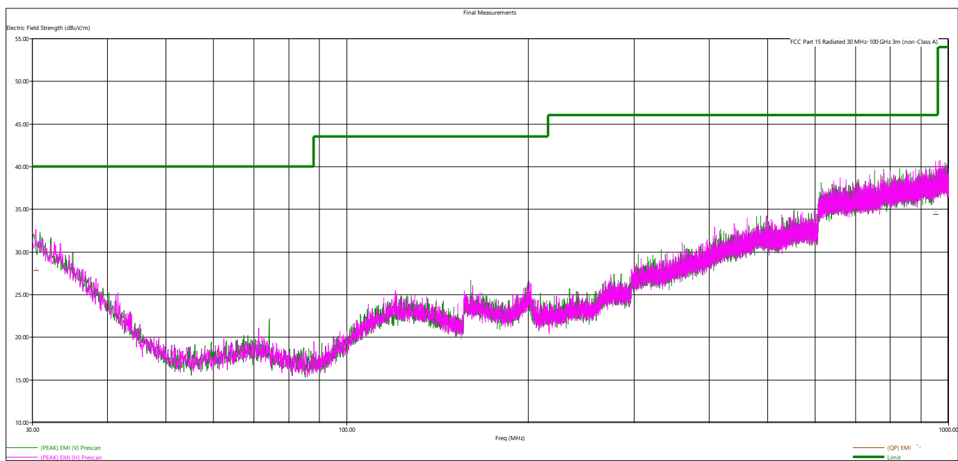
Figure 5 - Radiated Emissions Plot, Receive/ Idle Mode
