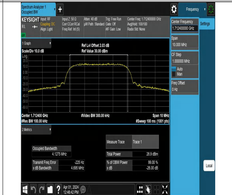
Band4-1312-4-PASS
