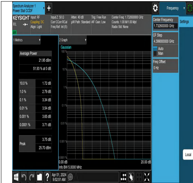
Band4-1413-1-PASS
