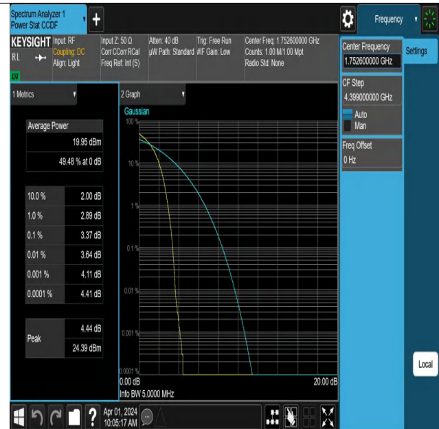
Band4-1513-4-PASS
