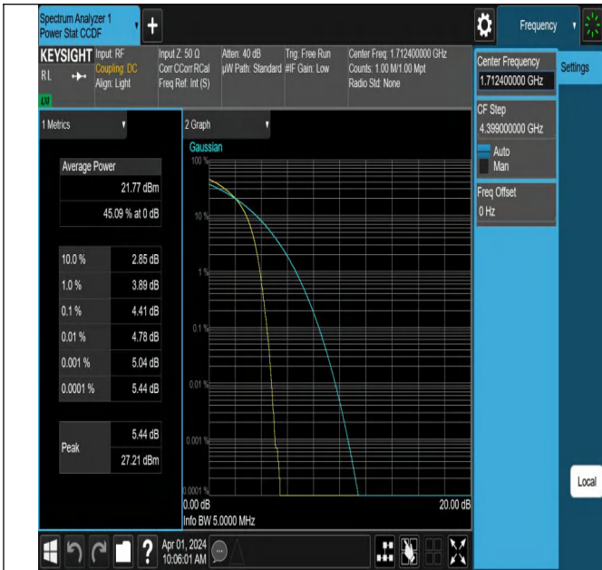
Band4-1312-5-PASS
