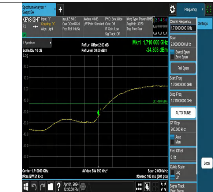
Band4-1312-4-PASS
