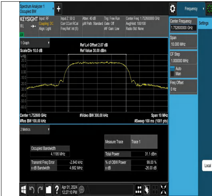
Band4-1513-1-PASS
