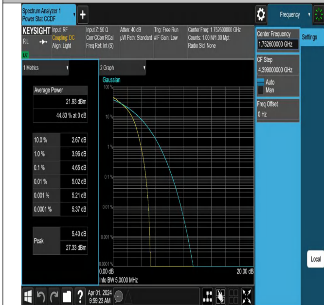
Band4-1513-1-PASS
