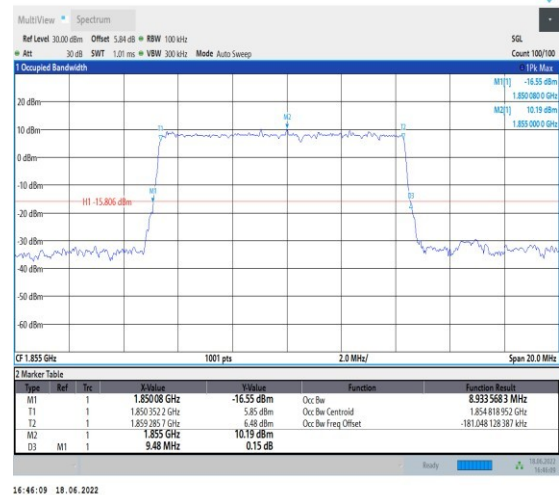
1-N25-PC3-15-10-L-5-DFT-256QAM-Outer_Full-50 @0-Ant1-8.934-9.480-≤10-PASS
