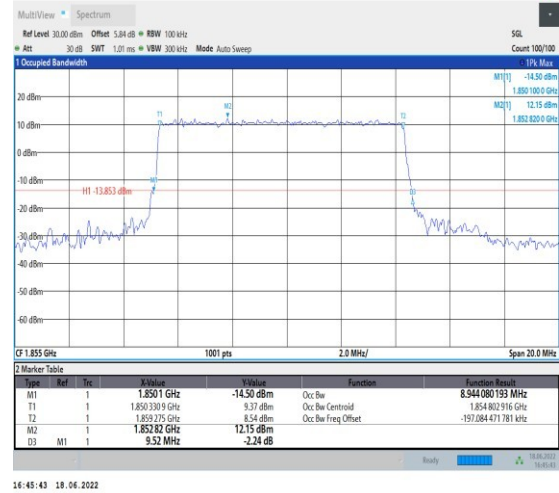
1-N25-PC3-15-10-L-3-DFT-16QAM-Outer_Full-50@ 0-Ant1-8.944-9.520-≤10-PASS
