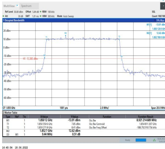
1-N25-PC3-15-10-L-4-DFT-64QAM-Outer_Full-50@ 0-Ant1-8.921-9.440-≤10-PASS
