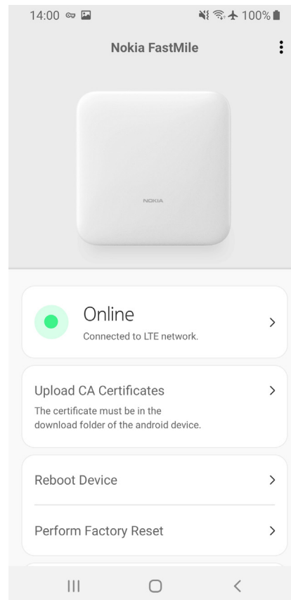
Figure 49 Screen that has the “Upload CA certificates” option for a Nokia FastMile 4G Receiver managed by an ACS through TR-069
