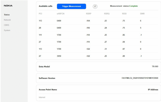
Figure 58 Example of the lower part of the Status screen with available cells when the FastMile 4G Receiver is not connected to a cell
