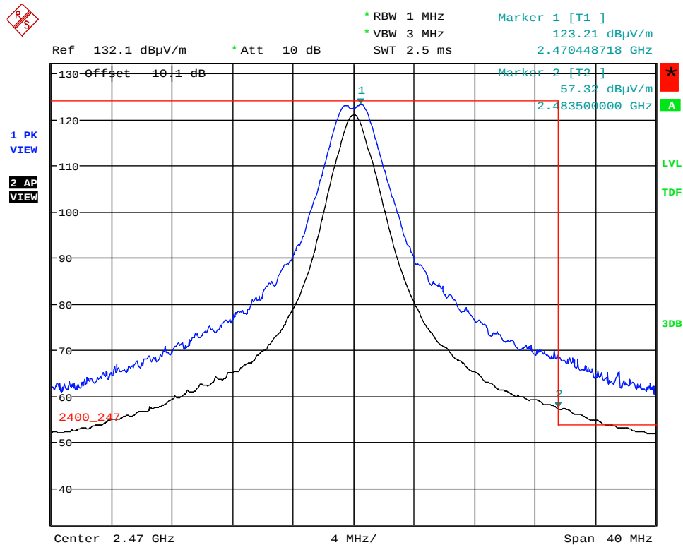
Plot 5.2.4.4.2.6. Band-Edge RF Radiated Emissions at 3 m, Vertical Polarization Highest End of Frequency Band, Ch24- 2470 MHz, QPSK Modulation, Power -8 Mode 3 @ 66% Duty Cycle
