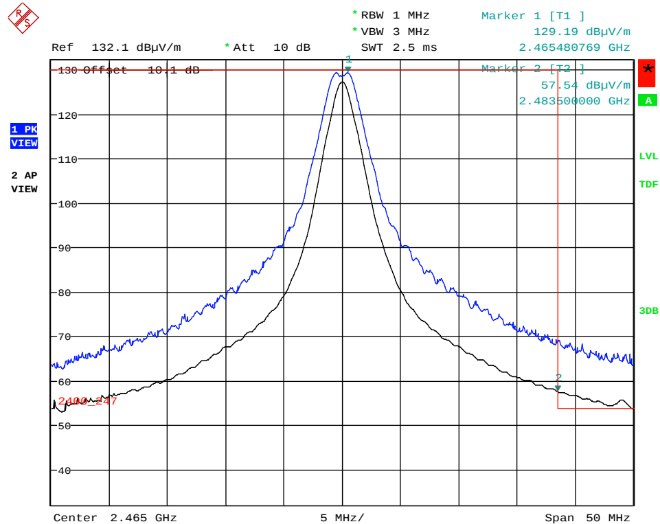
Plot 5.2.4.5.2.4. Band-Edge RF Radiated Emissions at 3 m, Vertical Polarization Higher End of Frequency Band, Ch23- 2465 MHz, QPSK Modulation, Power -8 Mode 3 @ 66% Duty Cycle
