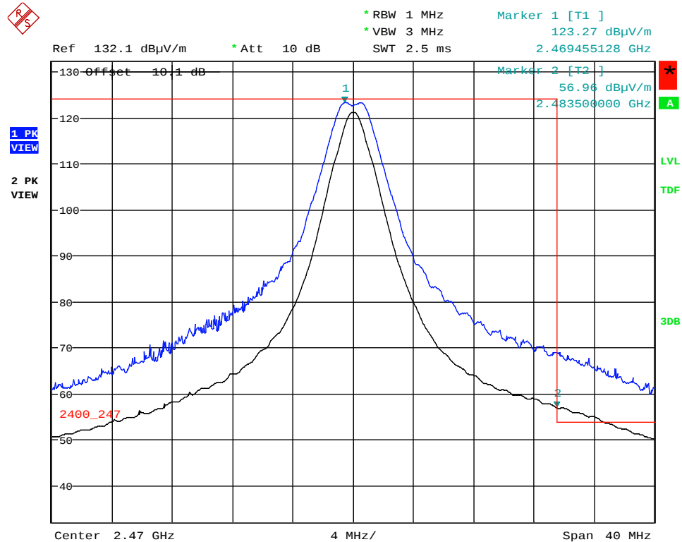
Plot 5.2.4.3.2.6. Band-Edge RF Radiated Emissions at 3 m, Vertical Polarization Highest End of Frequency Band, Ch24- 2470 MHz, QPSK Modulation, Power -8 Mode 3 @ 66% Duty Cycle
