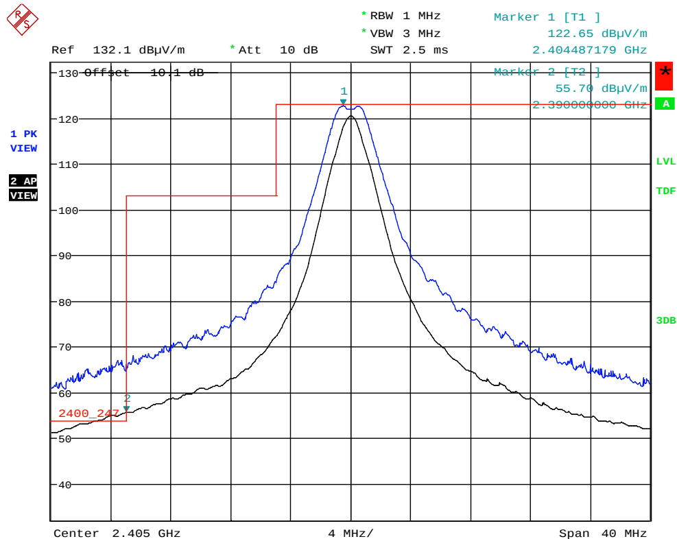
Plot 5.2.4.3.2.1. Band-Edge RF Radiated Emissions at 3 m, Horizontal Polarization Low End of Frequency Band, Ch11- 2405 MHz, QPSK Modulation, Power -8 Mode 3 @ 66% Duty Cycle
