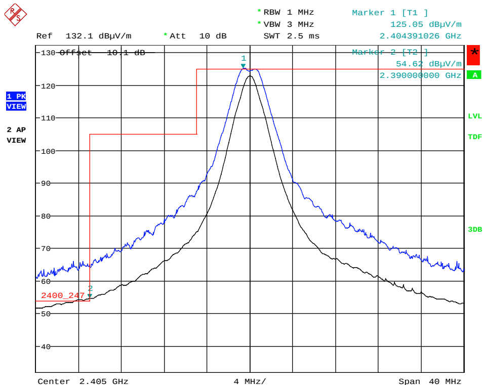
Plot 5.2.4.3.2.2. Band-Edge RF Radiated Emissions at 3 m, Vertical Polarization Low End of Frequency Band, Ch11- 2405 MHz, QPSK Modulation, Power -8 Mode 3 @ 66% Duty Cycle
