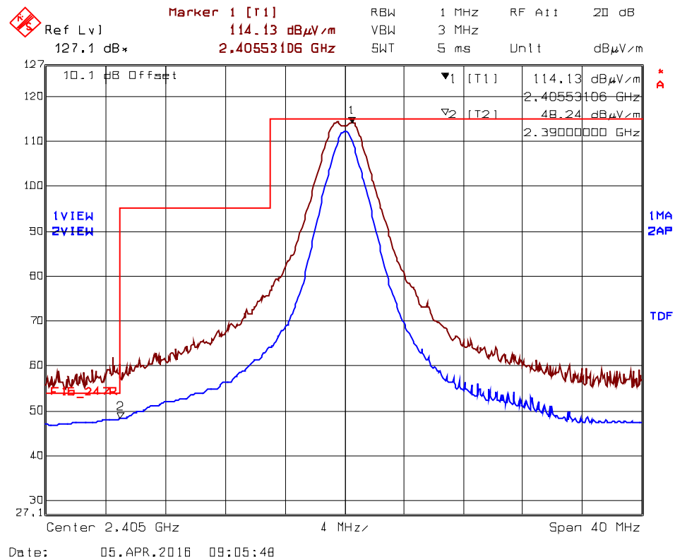
Plot 5.2.4.1.2.1. Band-Edge RF Radiated Emissions at 3 m, Horizontal Polarization Low End of Frequency Band, Ch11- 2405 MHz, QPSK Modulation, Power -8 Mode 3
