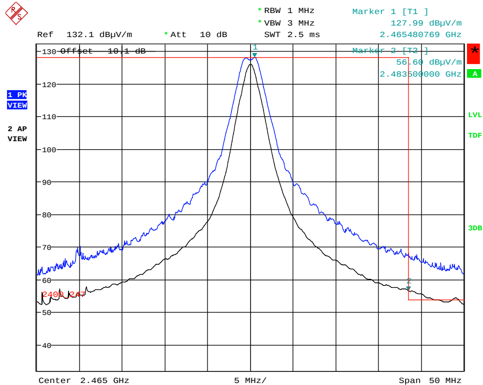
Plot 5.2.4.4.2.4. Band-Edge RF Radiated Emissions at 3 m, Vertical Polarization Higher End of Frequency Band, Ch23- 2465 MHz, QPSK Modulation, Power -8 Mode 3 @ 66% Duty Cycle
