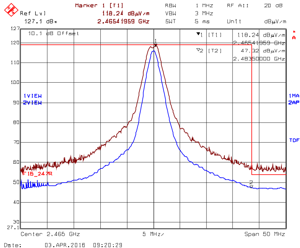
Plot 5.2.4.2.3. Band-Edge RF Radiated Emissions at 3 m, Horizontal Polarization High End of Frequency Band, Ch23- 2465 MHz, QPSK Modulation, Power -8 Mode 3
