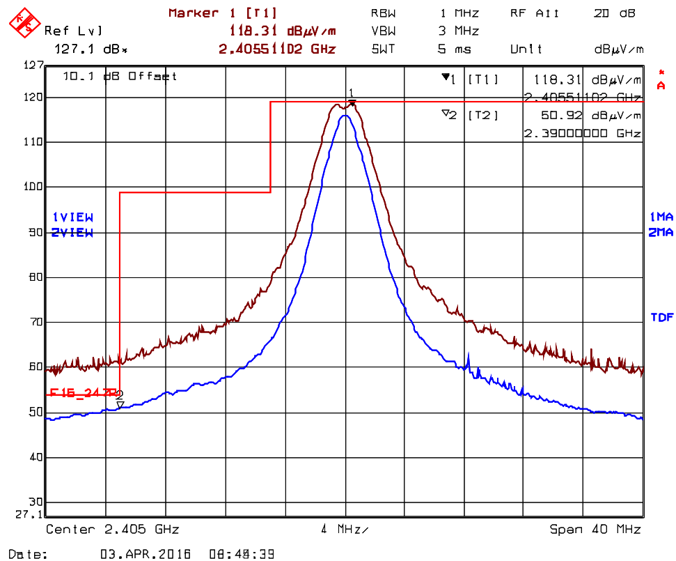
Plot 5.2.4.2.1. Band-Edge RF Radiated Emissions at 3 m, Horizontal Polarization Low End of Frequency Band, Ch11- 2405 MHz, QPSK Modulation, Power -8 Mode 3
