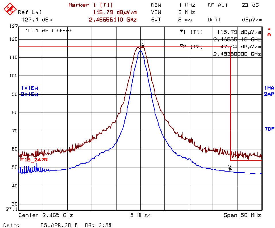
Plot 5.2.4.1.2.4. Band-Edge RF Radiated Emissions at 3 m, Vertical Polarization High End of Frequency Band, Ch23- 2465 MHz, QPSK Modulation, Power -8 Mode 3
