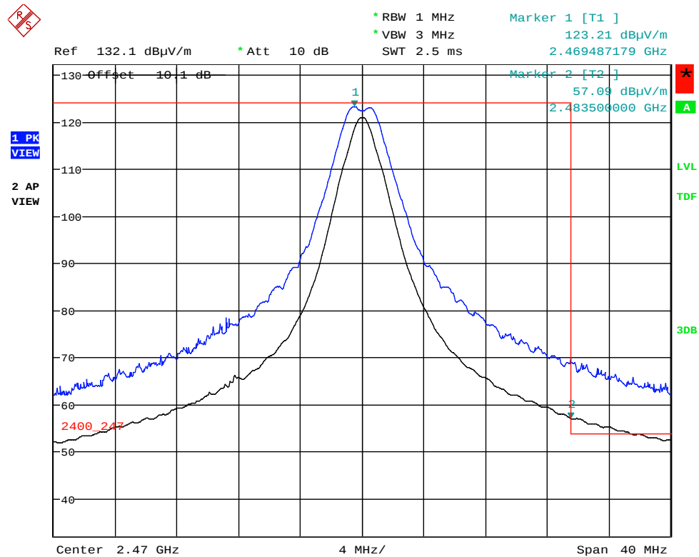
Plot 5.2.4.5.2.6. Band-Edge RF Radiated Emissions at 3 m, Vertical Polarization Highest End of Frequency Band, Ch24- 2470 MHz, QPSK Modulation, Power -8 Mode 3 @ 66% Duty Cycle
