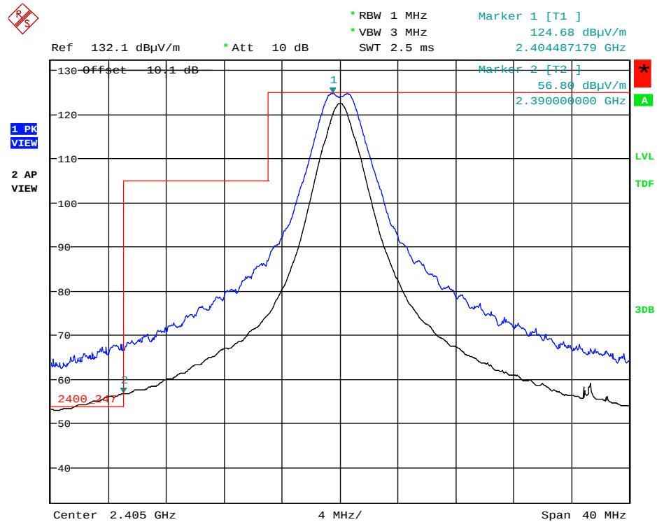
Plot 5.2.4.5.2.2. Band-Edge RF Radiated Emissions at 3 m, Vertical Polarization Low End of Frequency Band, Ch11- 2405 MHz, QPSK Modulation, Power -8 Mode 3 @ 66% Duty Cycle
