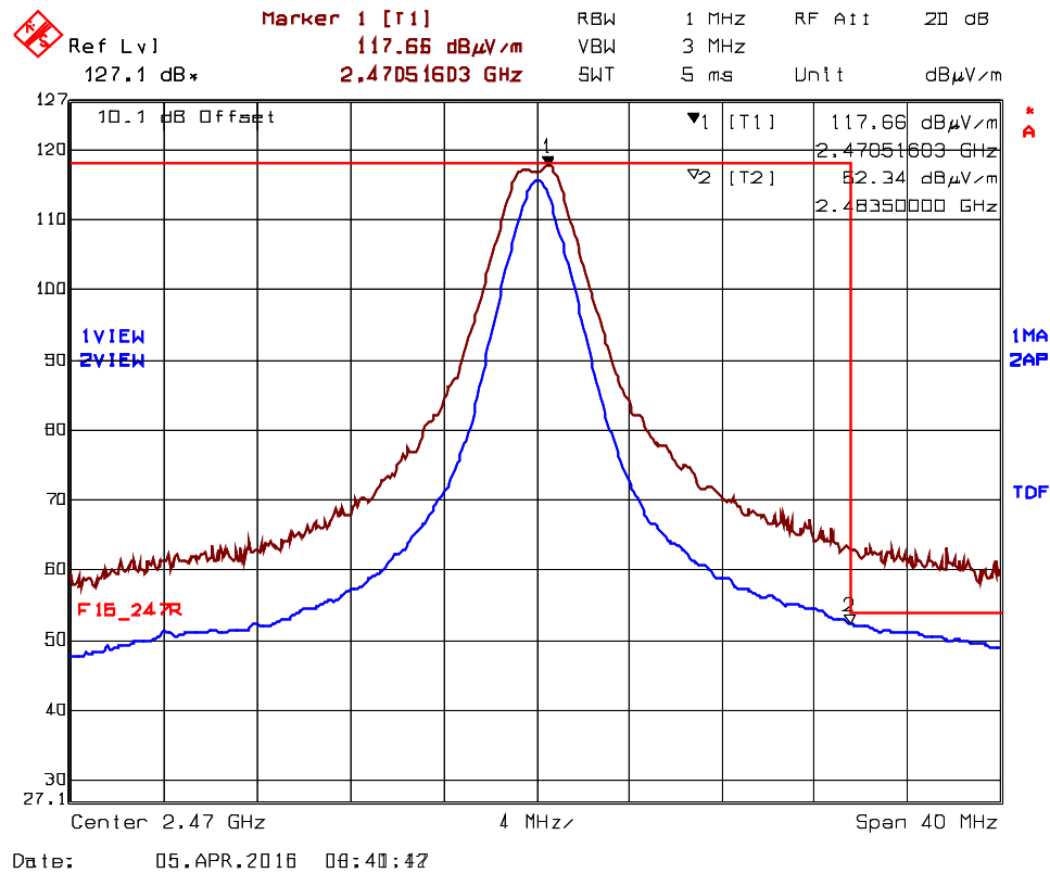
Plot 5.2.4.1.2.5. Band-Edge RF Radiated Emissions at 3 m, Horizontal Polarization Highest End of Frequency Band, Ch24- 2470 MHz, QPSK Modulation, Power -8 Mode 3
