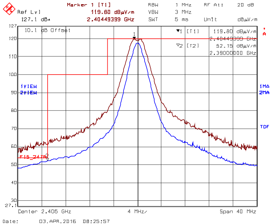
Plot 5.2.4.2.2.2. Band-Edge RF Radiated Emissions at 3 m, Vertical Polarization Low End of Frequency Band, Ch11- 2405 MHz, QPSK Modulation, Power -8 Mode 3
