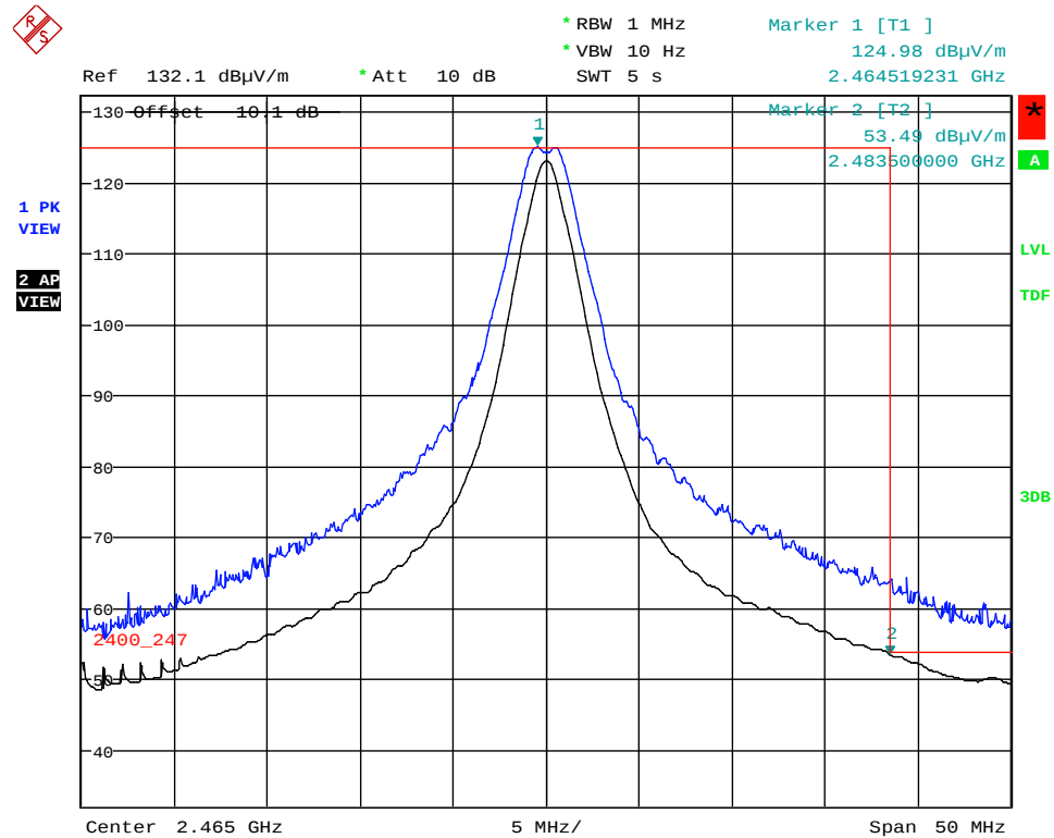
Plot 5.2.4.3.2.4. Band-Edge RF Radiated Emissions at 3 m, Vertical Polarization High End of Frequency Band, Ch23- 2465 MHz, QPSK Modulation, Power -8 Mode 3@ 66% Duty Cycle
