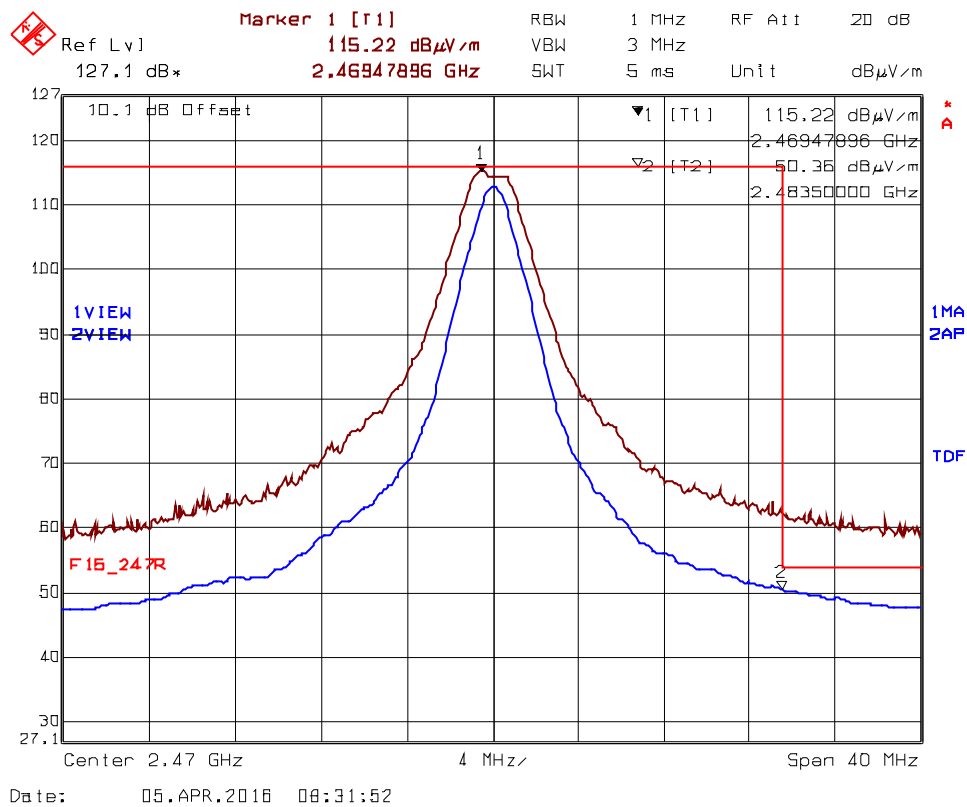
Plot 5.2.4.1.2.6. Band-Edge RF Radiated Emissions at 3 m, Vertical Polarization Highest End of Frequency Band, Ch24- 2470 MHz, QPSK Modulation, Power -8 Mode 3
