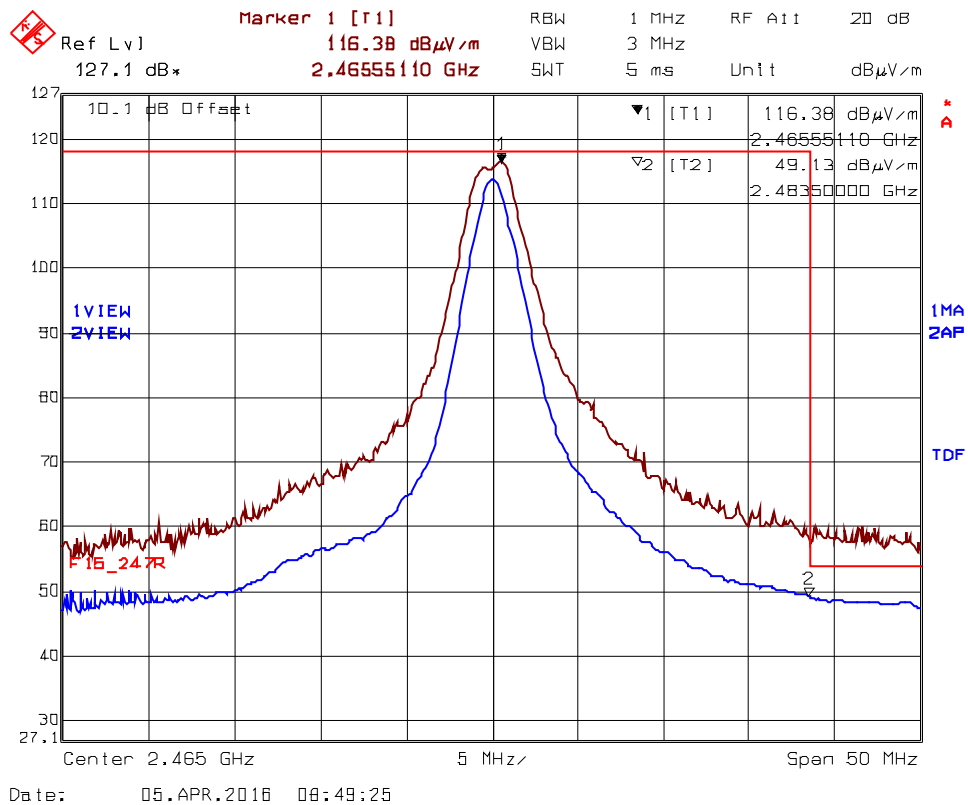
Plot 5.2.4.1.2.3. Band-Edge RF Radiated Emissions at 3 m, Horizontal Polarization High End of Frequency Band, Ch23- 2465 MHz, QPSK Modulation, Power -8 Mode 3
