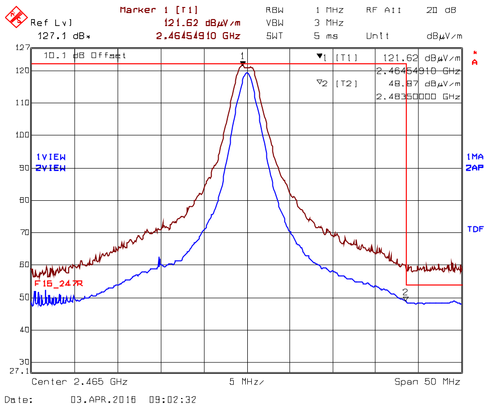
Plot 5.2.4.2.2.4. Band-Edge RF Radiated Emissions at 3 m, Vertical Polarization High End of Frequency Band, Ch23- 2465 MHz, QPSK Modulation, Power -8 Mode 3
