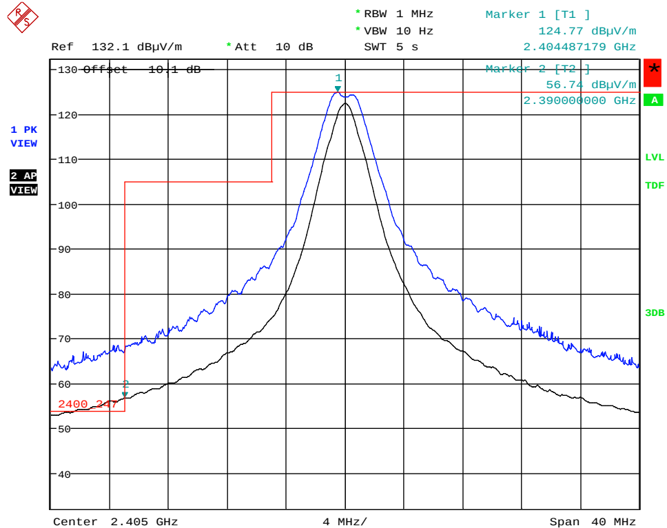
Plot 5.2.4.4.2.2. Band-Edge RF Radiated Emissions at 3 m, Vertical Polarization Low End of Frequency Band, Ch11- 2405 MHz, QPSK Modulation, Power -8 Mode 3 @ 66% Duty Cycle
