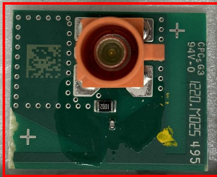
PCB Antenna WLAN 2.4 GHz
