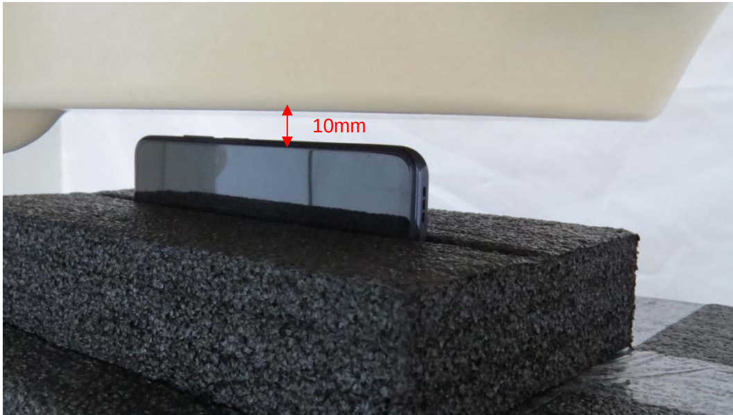
Picture 11: Right Side, the distance from handset to the bottom of the Phantom is 10mm
