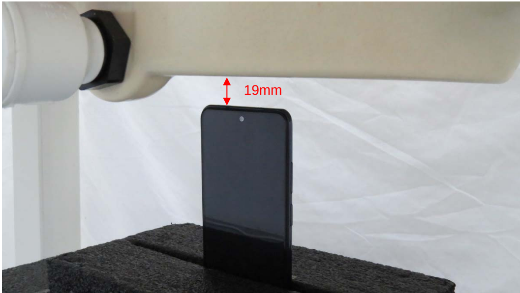
Picture 13: Top Side, the distance from handset to the bottom of the Phantom is 19mm
