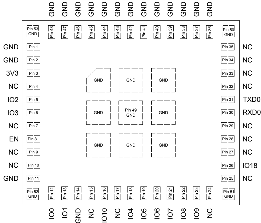
Figure 1: Pin Layout (Top View)
