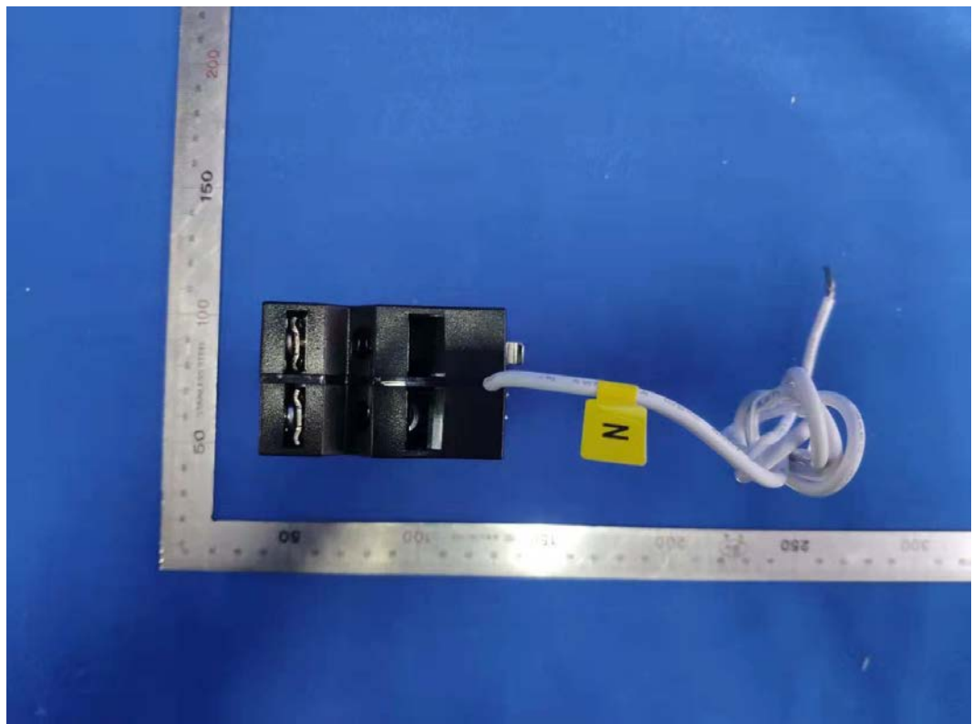
FIGURE 6 QO DUAL 20A RELAY, WITH CT, PIGTAIL (M/N: GPM-Q2R20120-21) RIGHT
