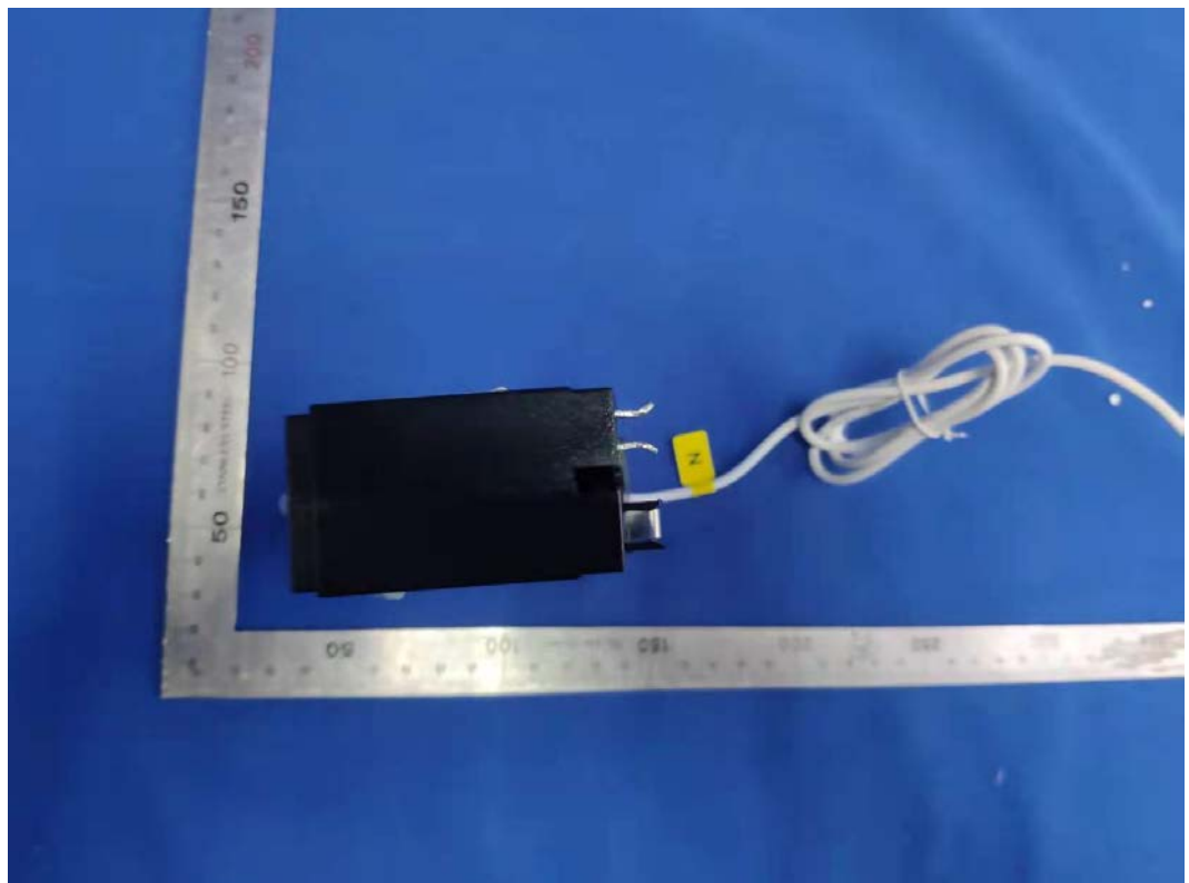
FIGURE 4 QO DUAL 20A RELAY,WITH CT, PIGTAIL (M/N: GPM-Q2R20120-21) LEFT
