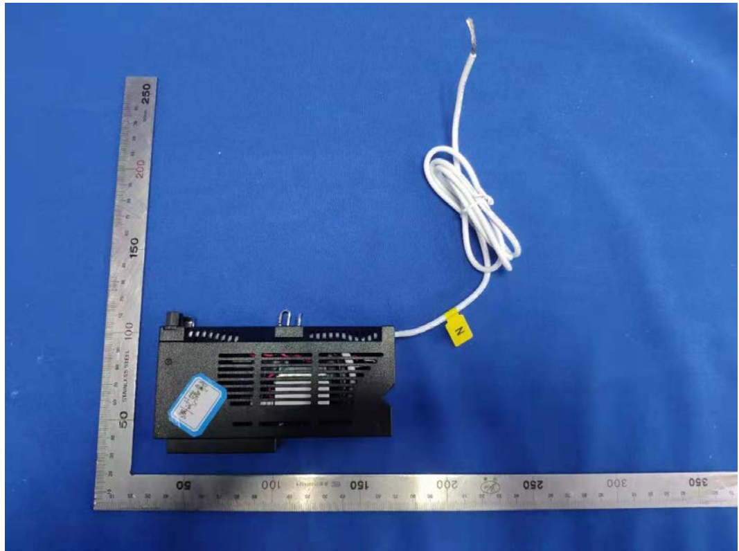
FIGURE 7 QO DUAL 20A RELAY, WITH CT, PIGTAIL (M/N: GPM-Q2R20120-21) BOTTOM
