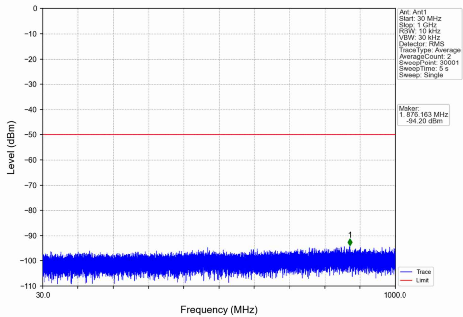
n48_30kHz_SISO_NTNV_20MHz_DFT-s-OFDM QPSK_3624.99MHz_Edge_1RB_Left
