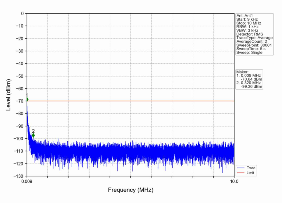
n48_30kHz_SISO_NTNV_20MHz_DFT-s-OFDM QPSK_3690MHz_Outer_Full
