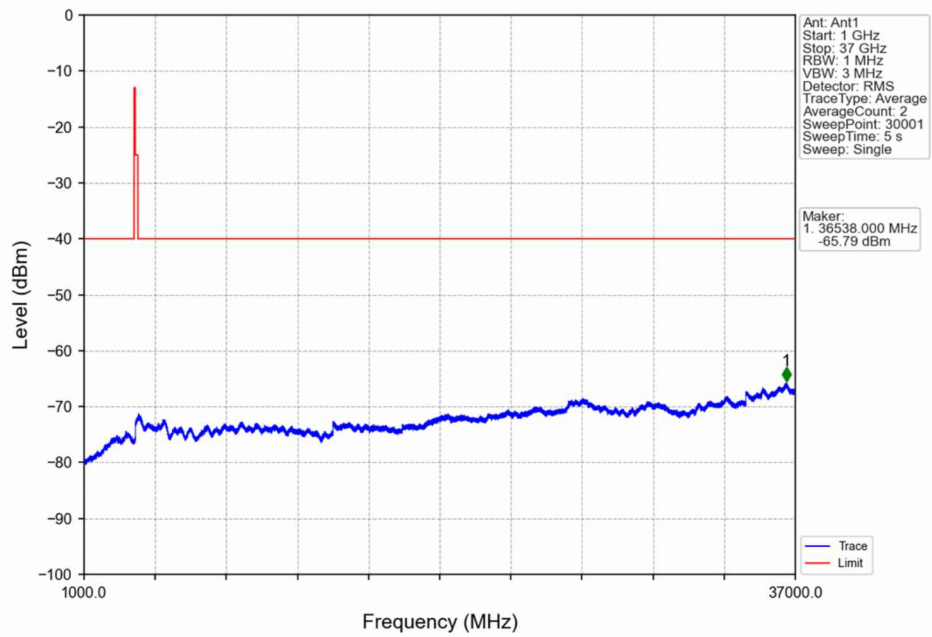
n48_30kHz_SISO_NTNV_20MHz_CP-OFDM QPSK_3560.01MHz_Outer_Full
