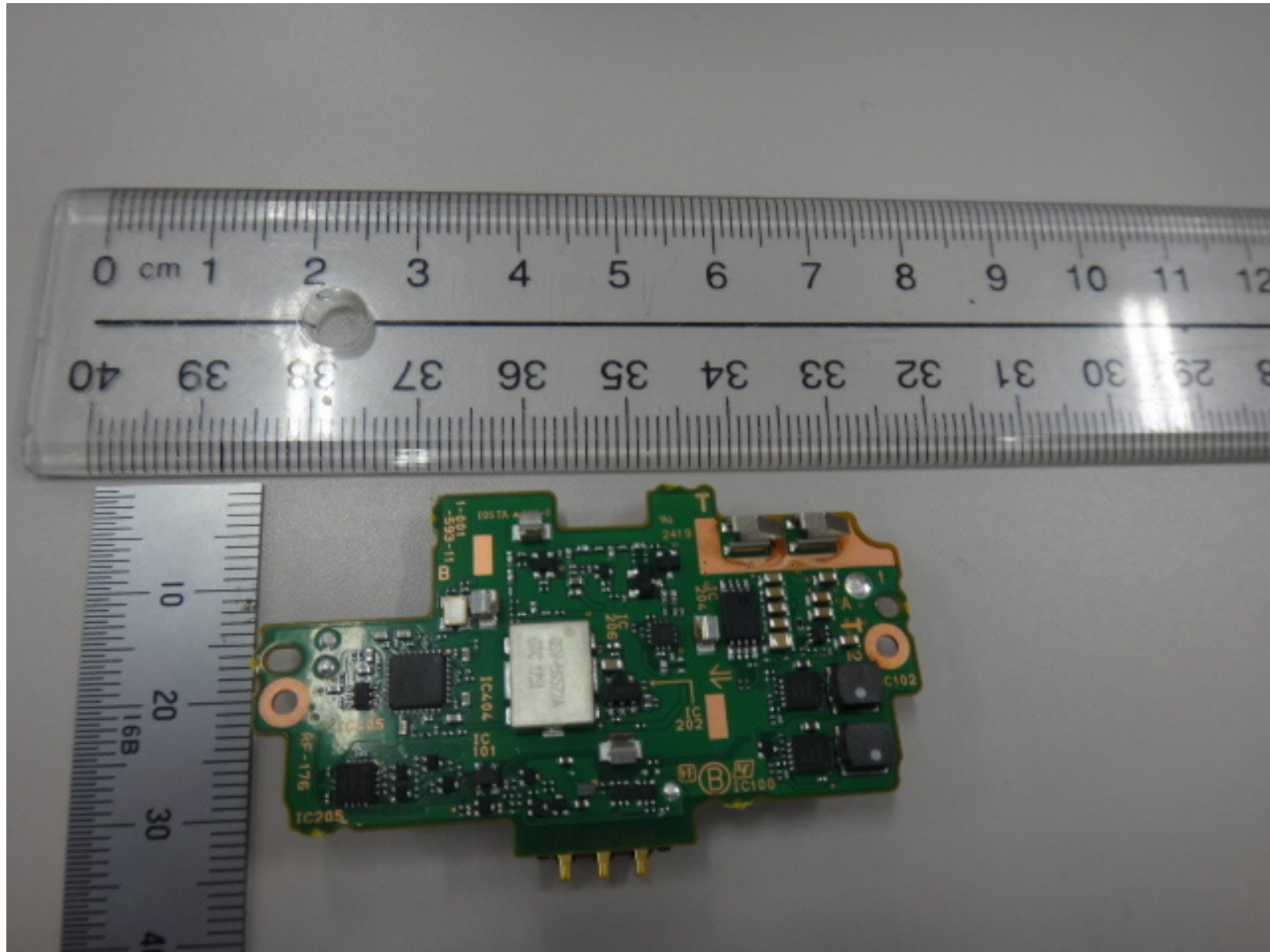
Side B of Board RF-176. (Without Shield case)
