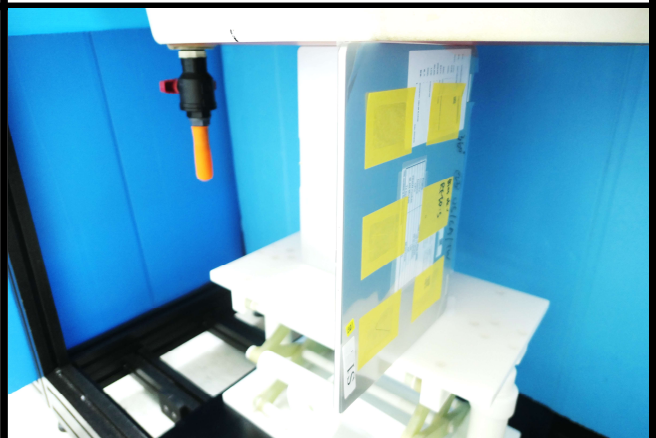
Keyboard Left Side of Laptop Tested at 0 mm
