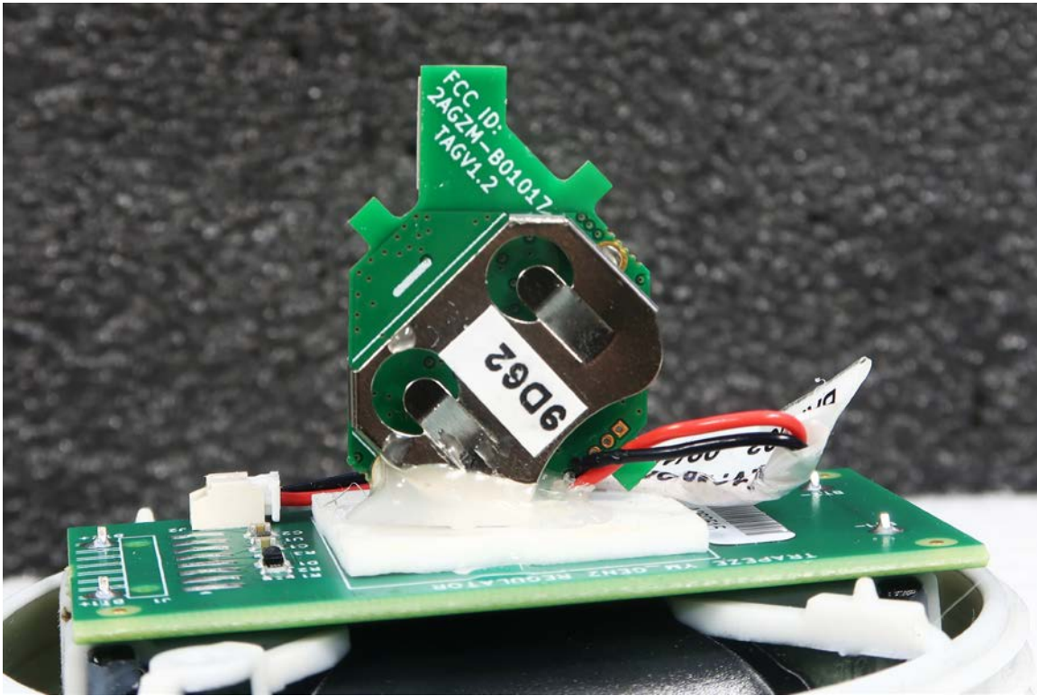
TAGV1.2T Transmitter Module Back
