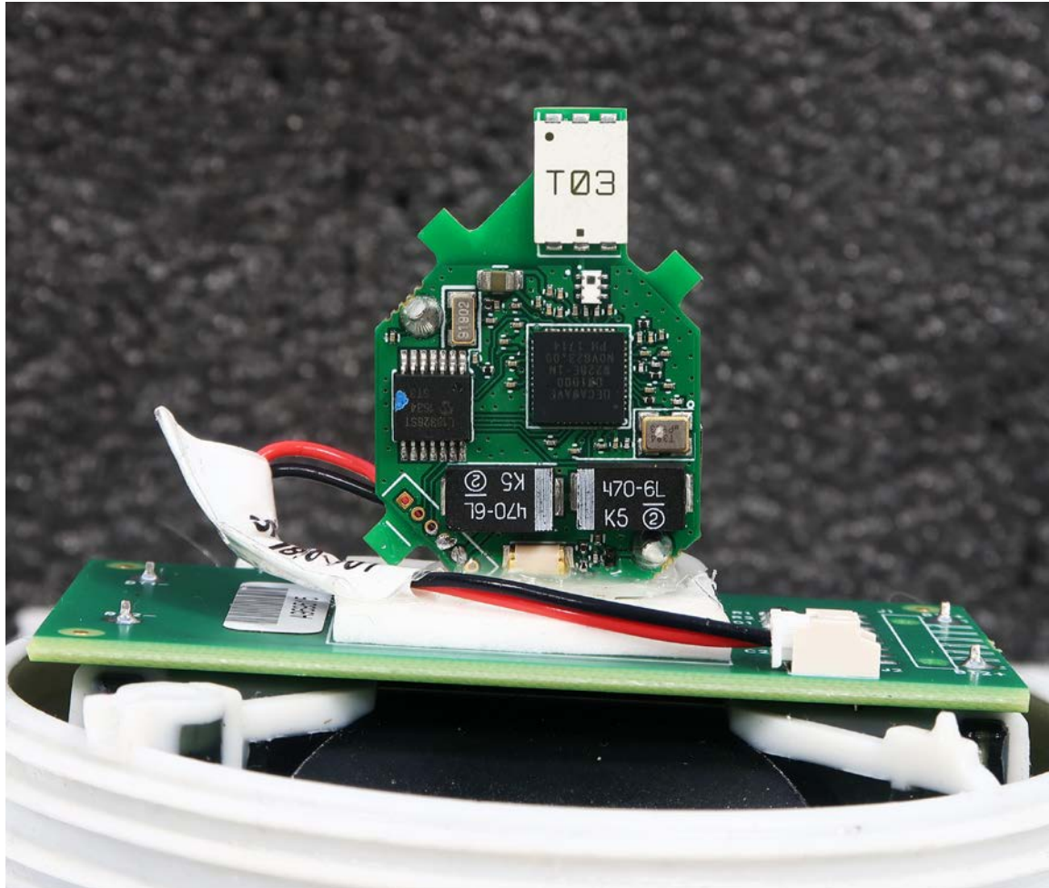
TAGV1.2T Transmitter Module Front close up
