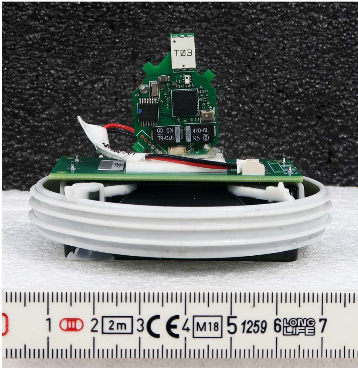
TAGV1.2T Transmitter Module Front
