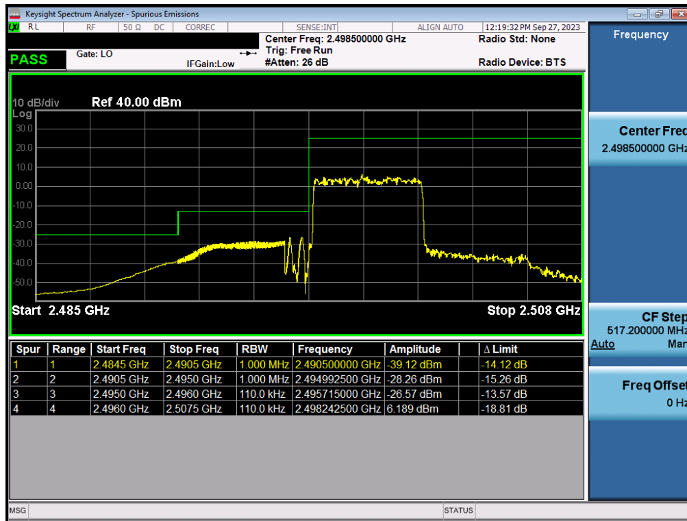
Plot 7-15. Lower ACP Plot (LTE Band 41(PC3) - 5MHz QPSK – Full RB)
