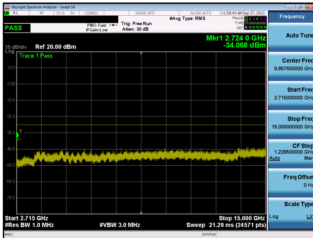
Plot 7-12. Conducted Spurious Plot (LTE Band 41(PC3) - 20MHz QPSK - RB Size 1, RB Offset 0 - High Channel)
